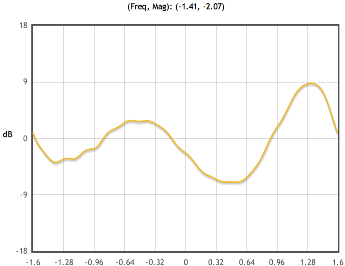
Figure 6: Frequency Response from Pre-Equalization Data
