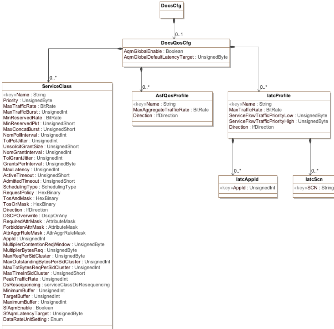
Figure 6-9 - DOCSIS QoS Configuration Objects
