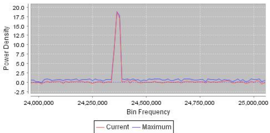
Figure VI-3 - Spectrum Amplitude Detail Graph from Collected Data
