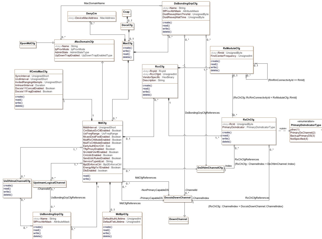
Figure 6-11 - MAC Domain Configuration Objects 28
