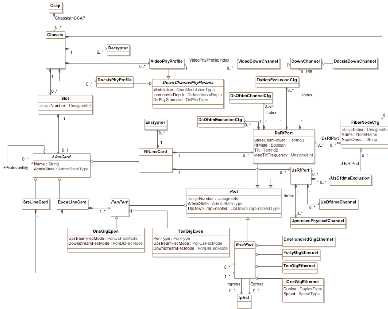
Figure 6-4 - CCAP Chassis Objects 15
