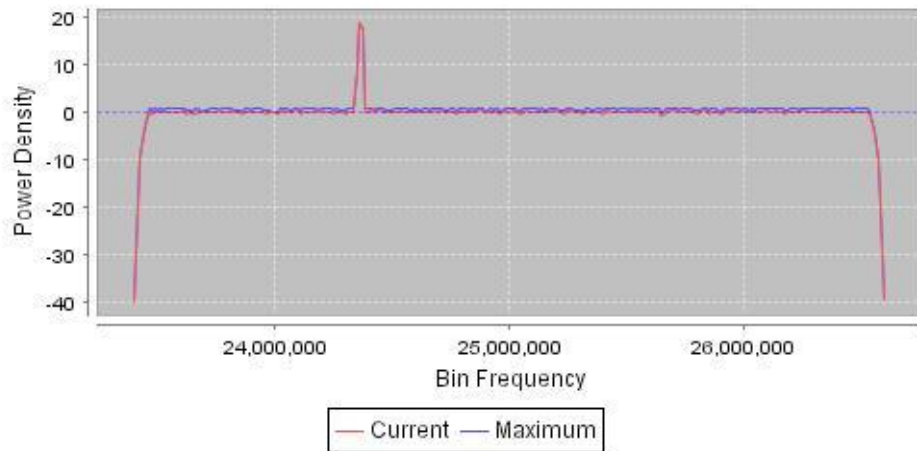
Figure VI-2 - Spectrum Amplitude Constructed Graph from Collected Data
