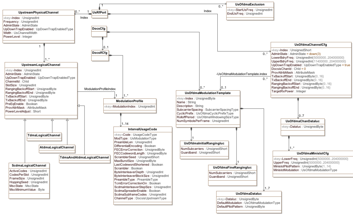
Figure 6-13 - DOCSIS Upstream Interface Configuration Objects 34
