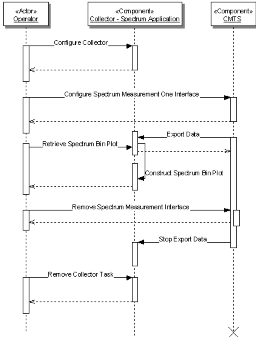
Figure VI-1 - Sequence Diagram for Streaming of Spectrum Analysis Measurement Data
