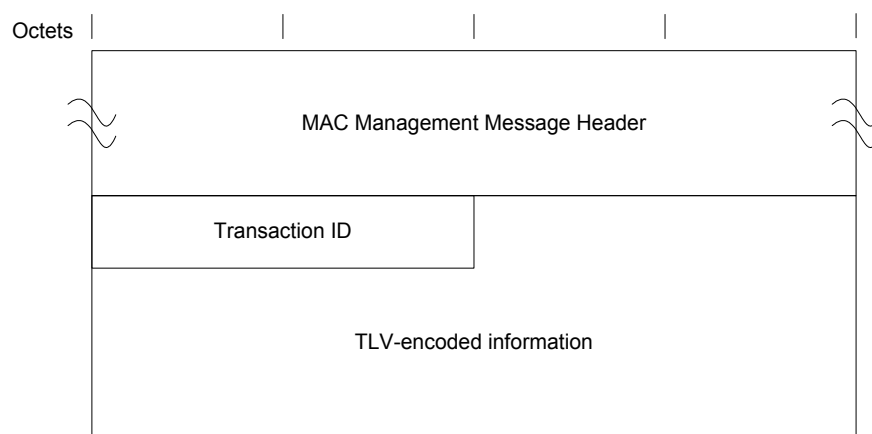
Figure 6–51 - Dynamic Bonding Change Acknowledge Message 161
