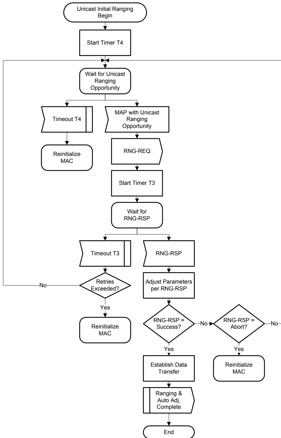
Figure 10-13 - Unicast Initial Ranging - CM 317
