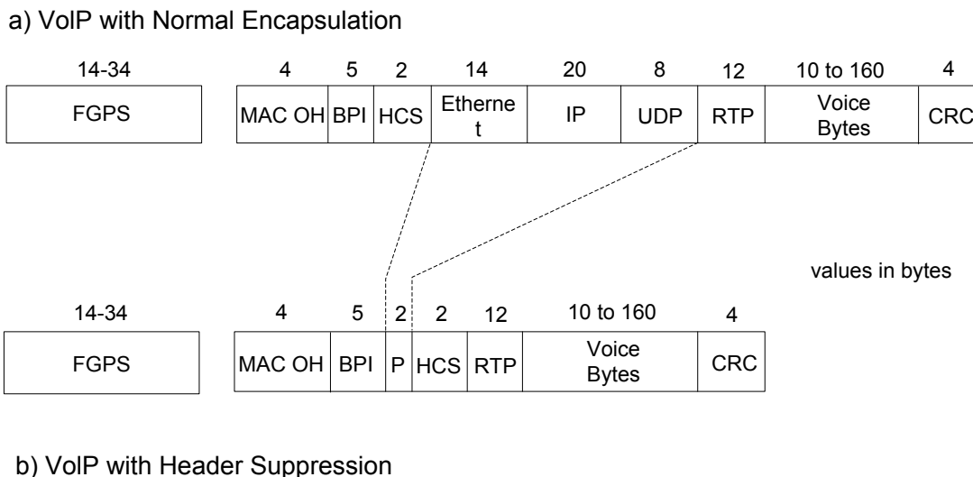
Figure 7–22 - Upstream Payload Header Suppression Example
