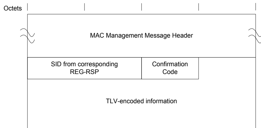
Figure 6–30 - Registration Acknowledgment 107
