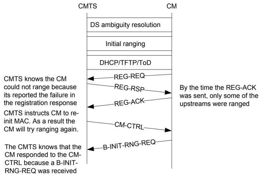
Figure V-1 - Example 1 - Modem can't range on all upstreams 728
