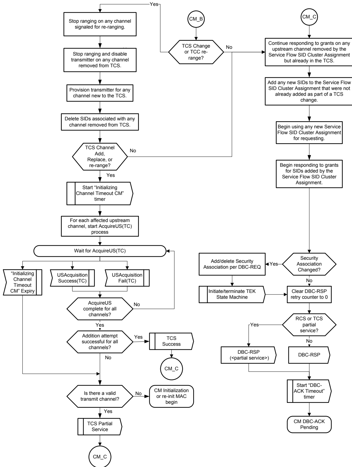
Figure 11-56 - CM DBC-RSP (part 3) 429
