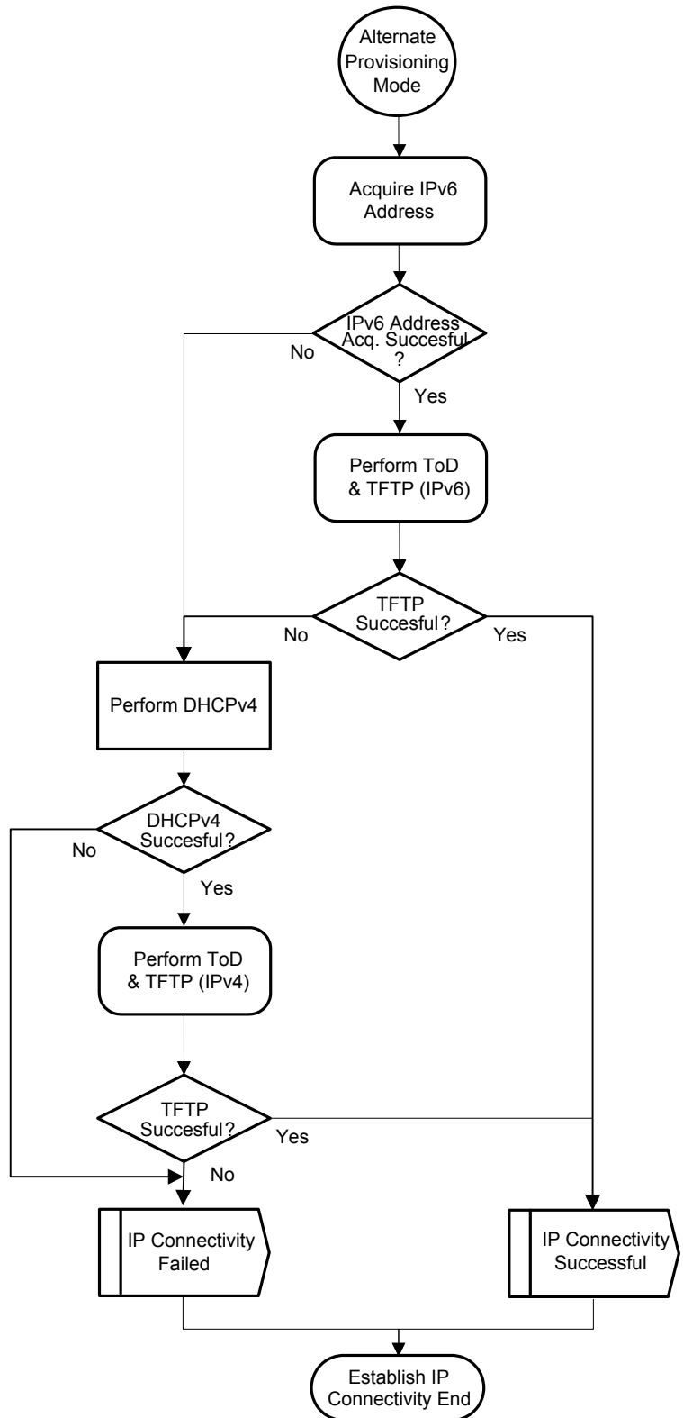
Figure 10-19 - Alternate Provisioning Mode
