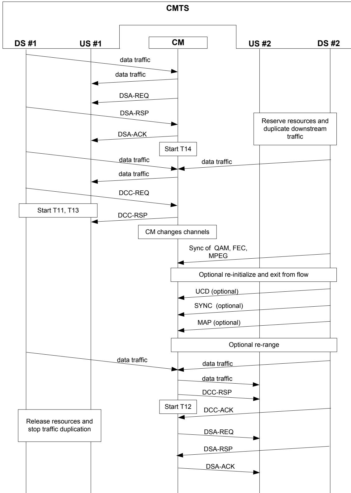
Figure XII-1 - DCC Example Operational Flow
