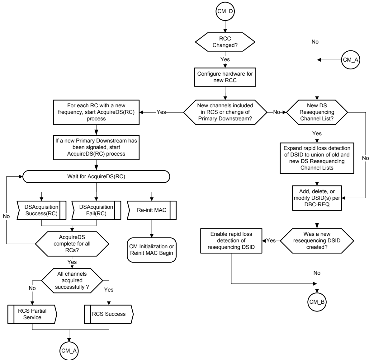
Figure 11-55 - CM DBC-RSP (part 2) 428
