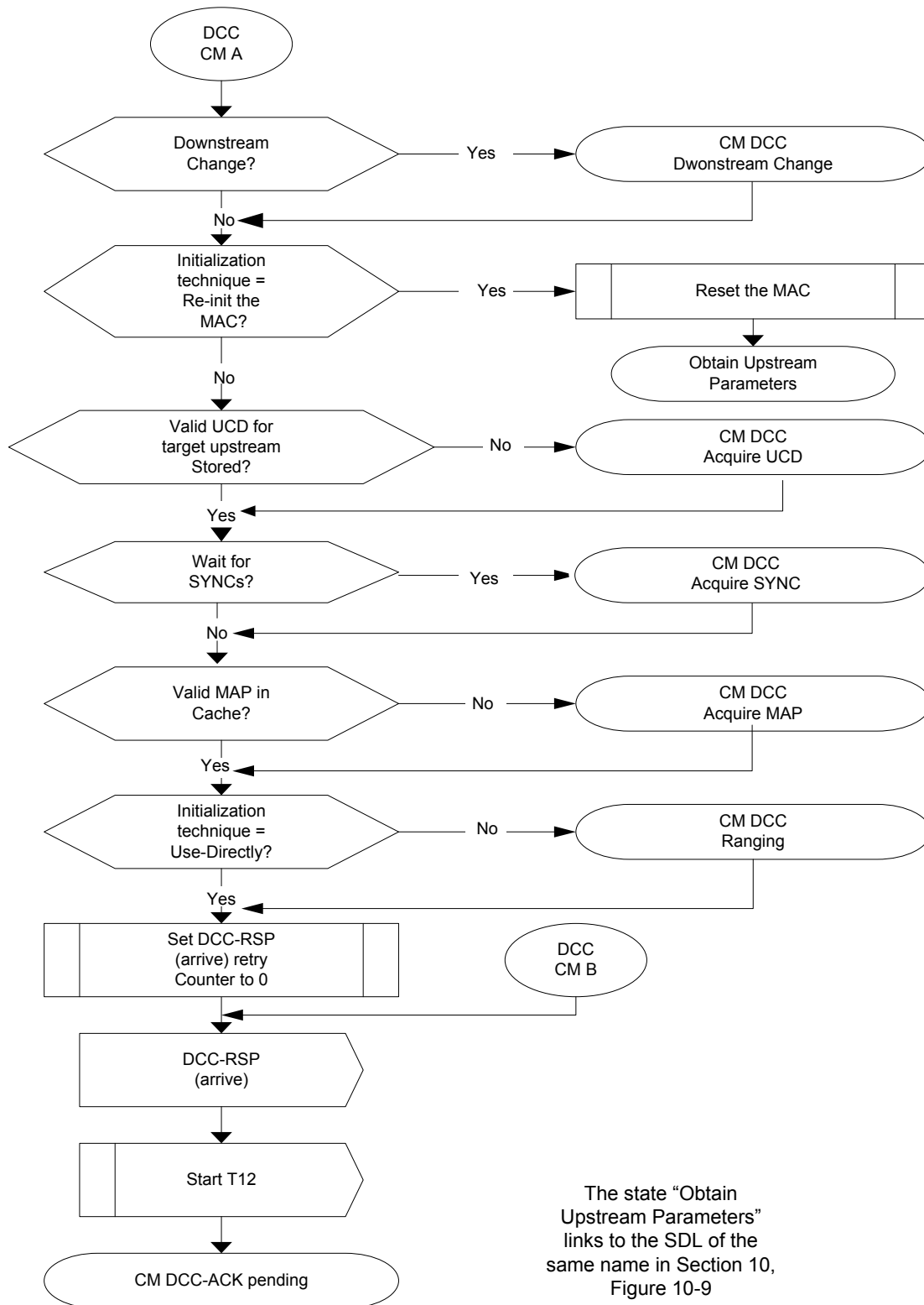
Figure 11-47 - Dynamically Changing Channels: CM View Part 2 405
