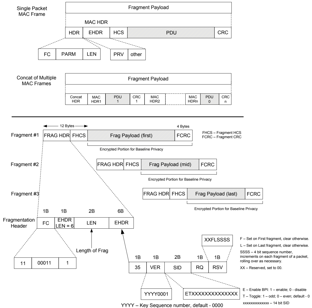
Figure 7-6 - Fragmentation Details 204
