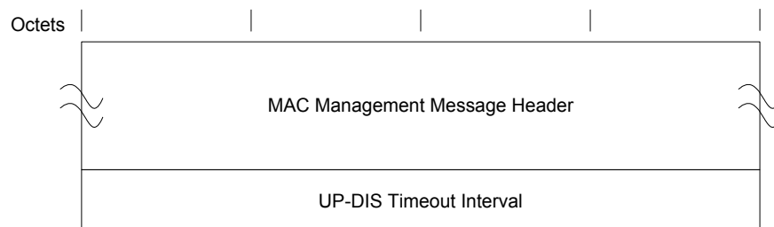
Figure 6–46 - UP-DIS message format 130
