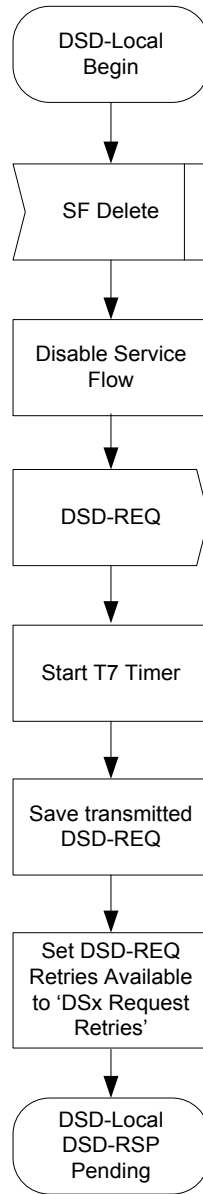
Figure 11–34 - DSD—Locally Initiated Transaction Begin State Flow Diagram
