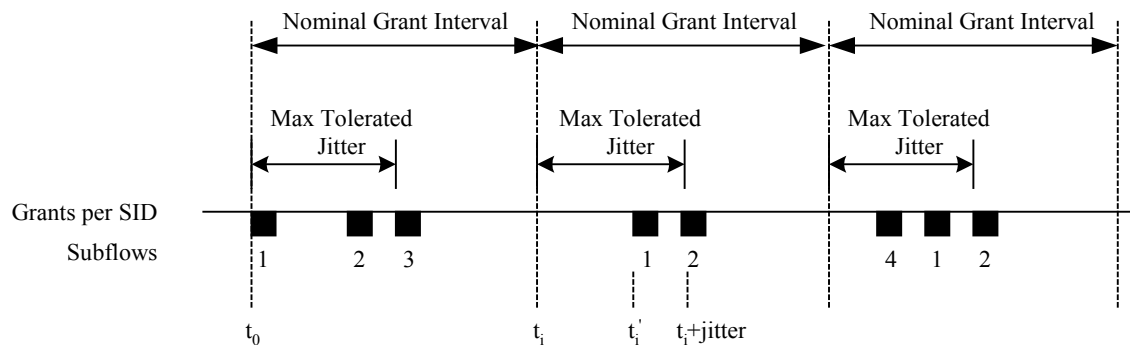
Figure IV-1 - Example Jitter with Multiple Grants per SID
