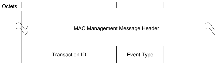
Figure 6–59 - CM STATUS-ACK message
