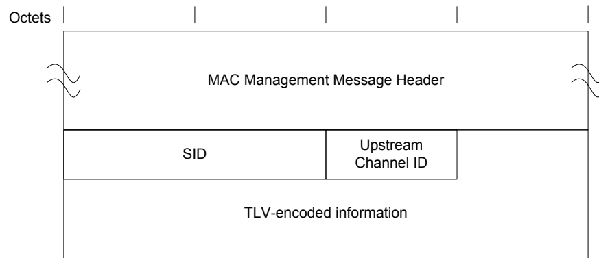
Figure 6–23 - Ranging Response 80
