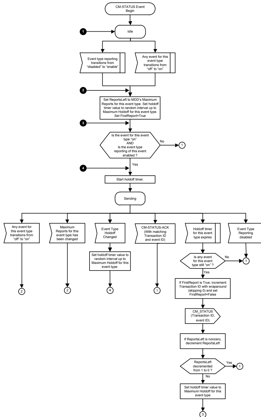
Figure 10–36 - CM-STATUS Event Type State Machine 382
