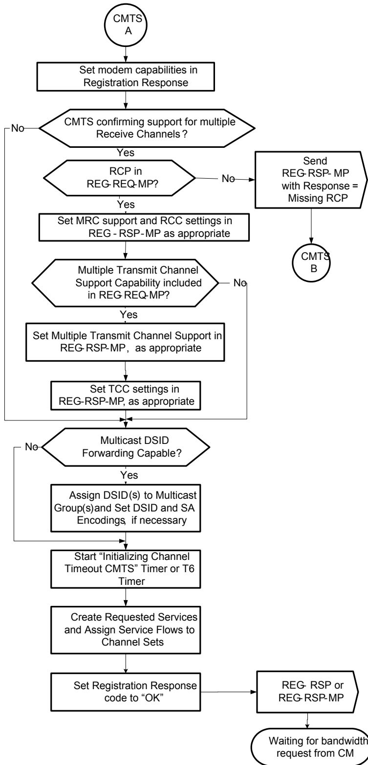
Figure 10-32 - CMTS Registration - Continued 365
