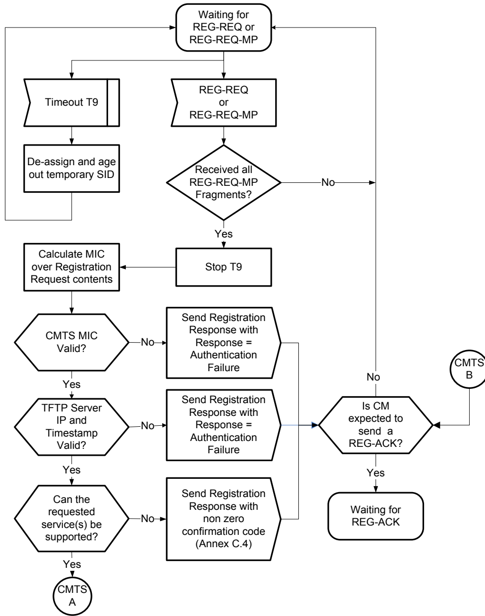
Figure 10-31 - CMTS Registration - Begin 364
