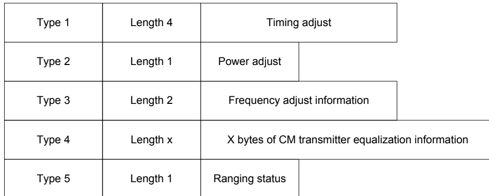
Figure 6–24 - Example of TLV Encoded Data
