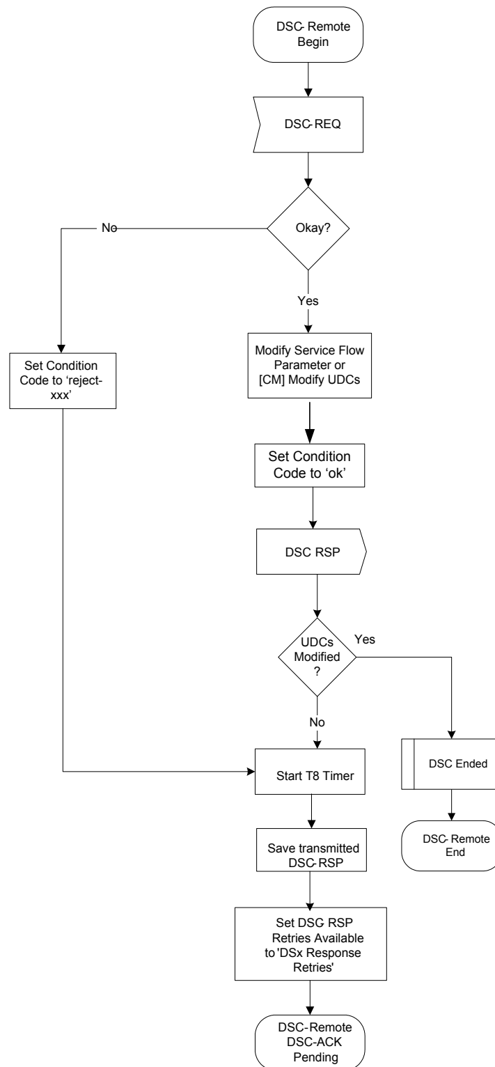
Figure 11-28 - DSC—Remotely Initiated Transaction Begin State Flow Diagram 396
