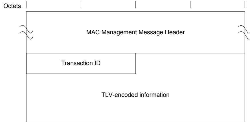
Figure 6–56 - CM-CTRL-RSP 174
