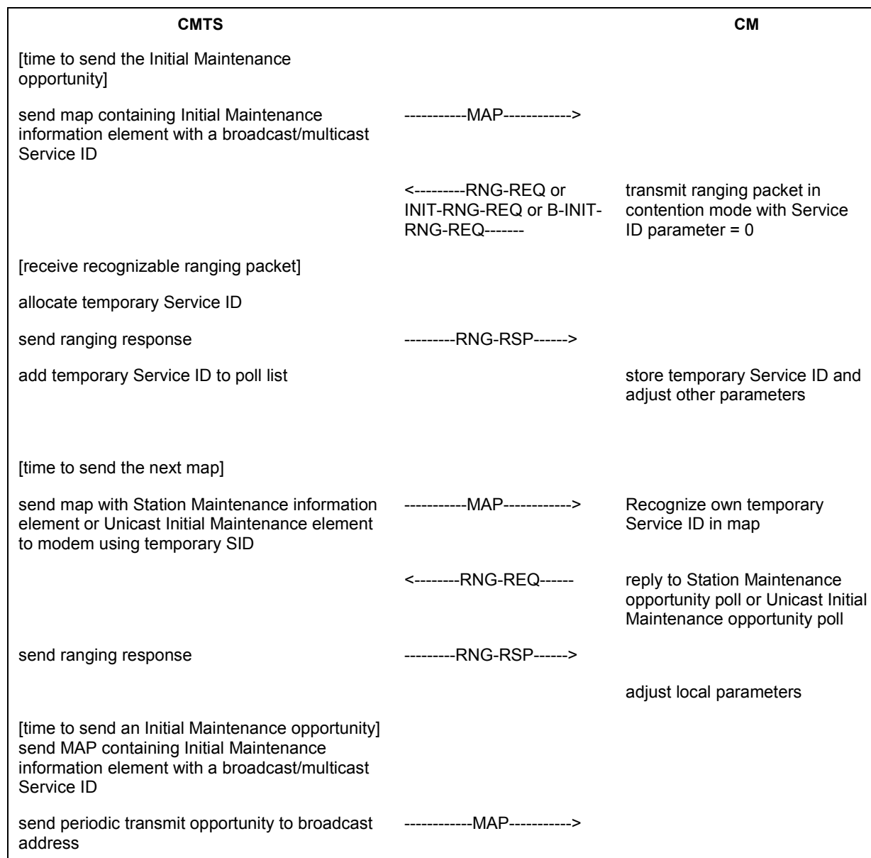
Figure 10–11 - Ranging and Automatic Adjustments Procedure
