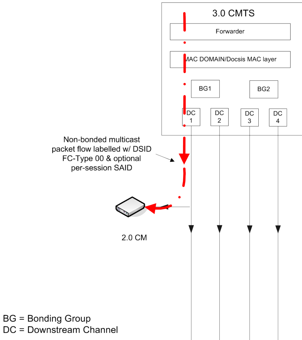
Figure VIII-1 - Multicast Session Replication for a client behind a 2.0 CM
