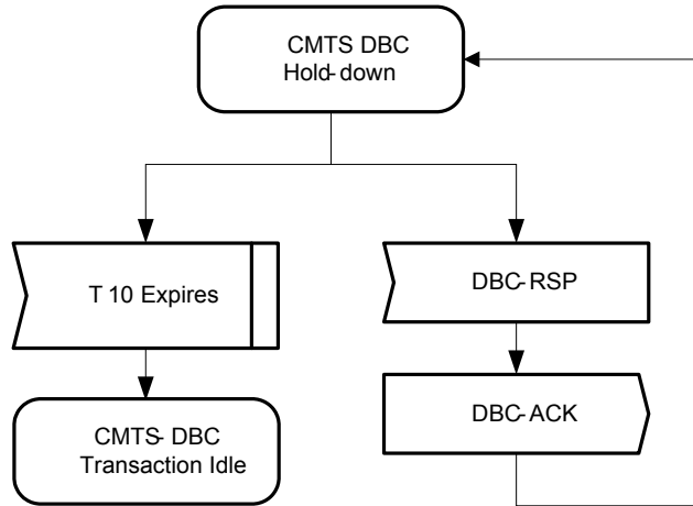
Figure 11-53 - CMTS DBC Hold-down 426
