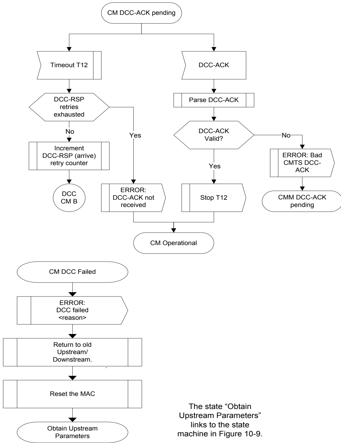
Figure 11-49 - Dynamically Changing Channels: CM View Part 4 407
