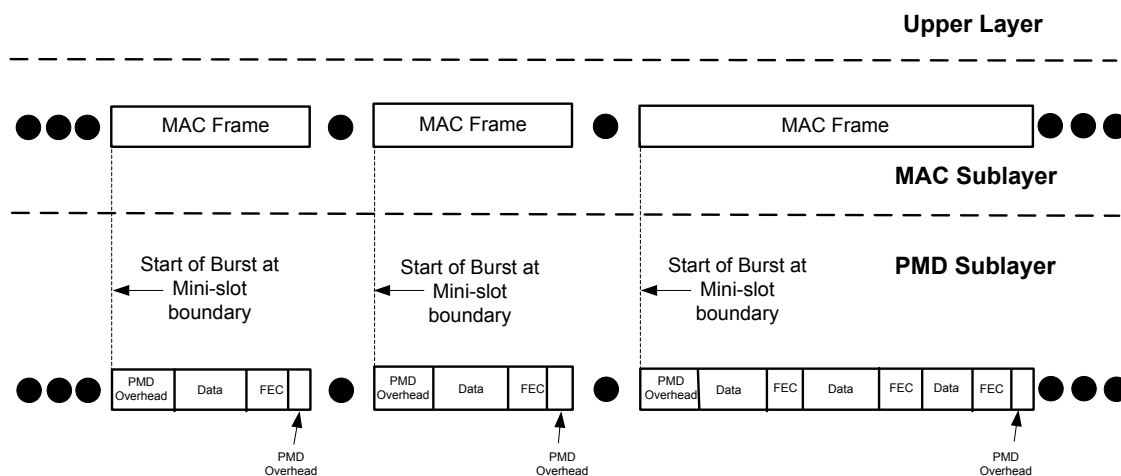
Figure 6–2 - Upstream MAC/PMD Convergence
