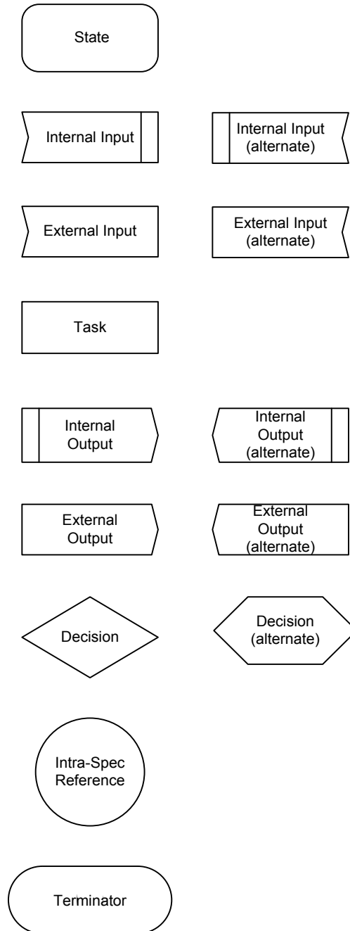
Figure VI-1 - Specification and Description Language (SDL) Notation
