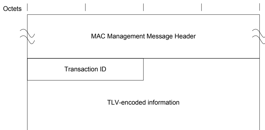
Figure 6–55 - CM-CTRL-REQ 171
