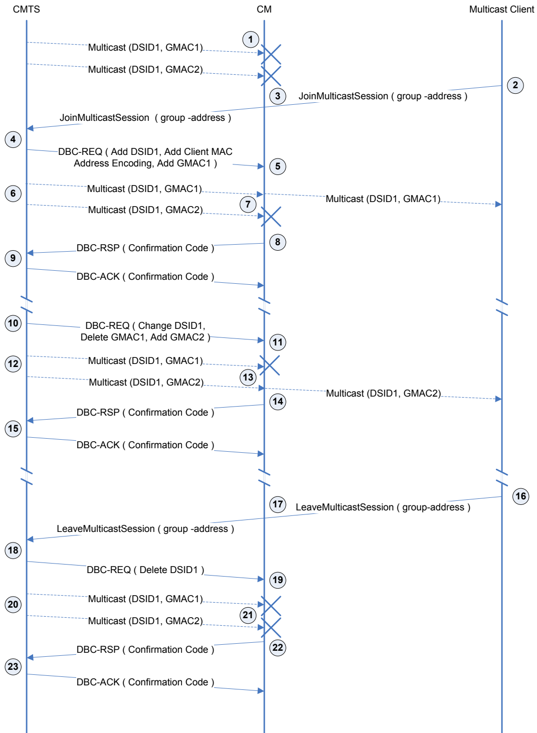
Figure G-1- Multicast Forwarding by a GMAC-Explicit CM 707
