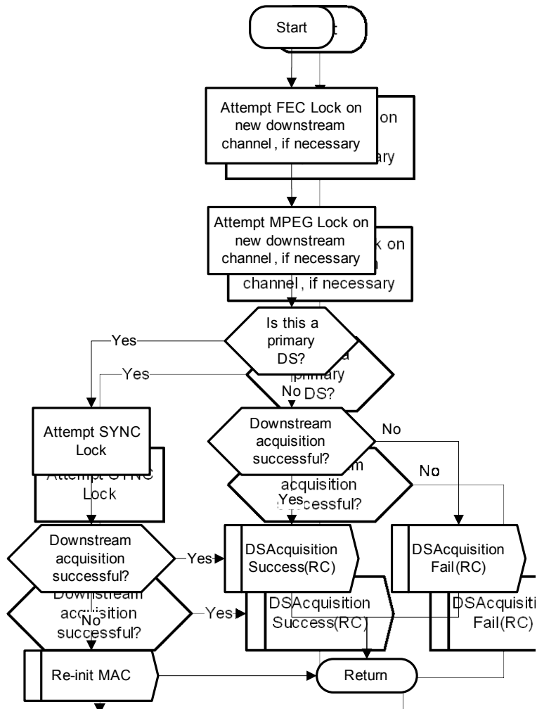
Figure 11-57 - CM AcquireDS Procedure 430
