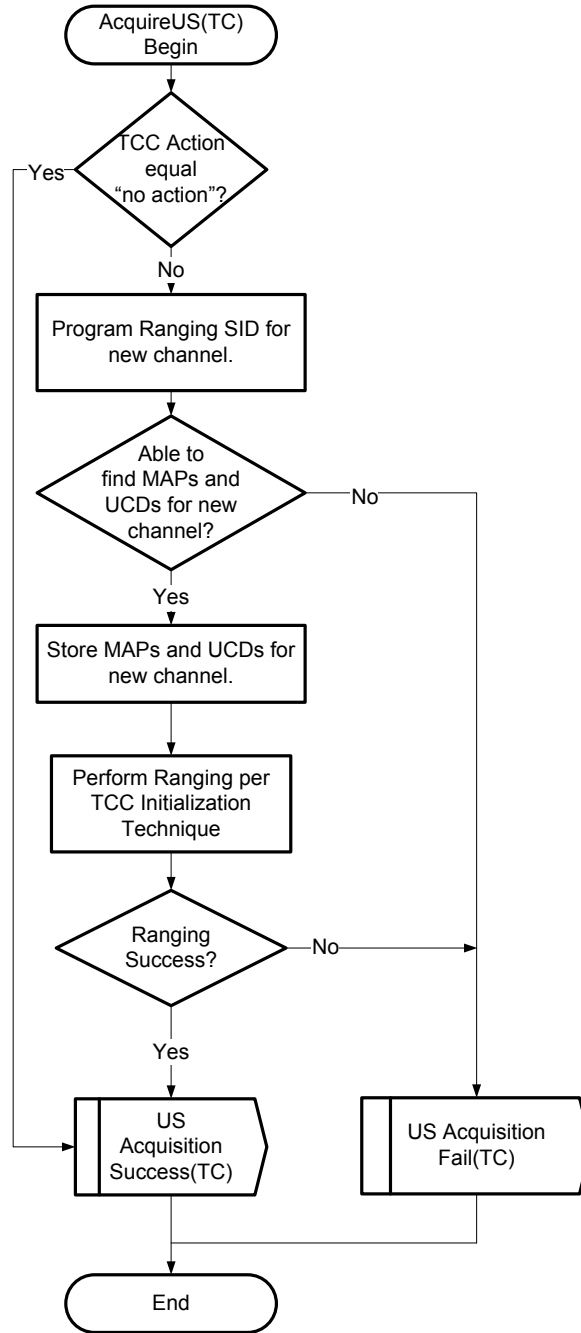
Figure 10–29 - CM Acquires Upstream Channels 354
