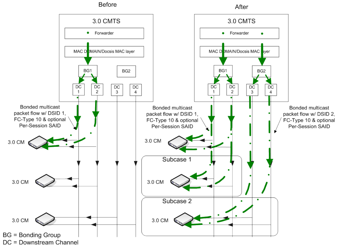
Figure VIII-8 - Multicast session replication to clients behind two 3.0 CMs 742
