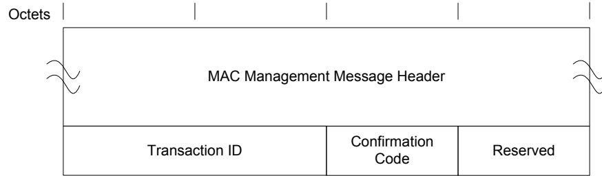
Figure 6–40 - Dynamic Service Deletion — Response 121
