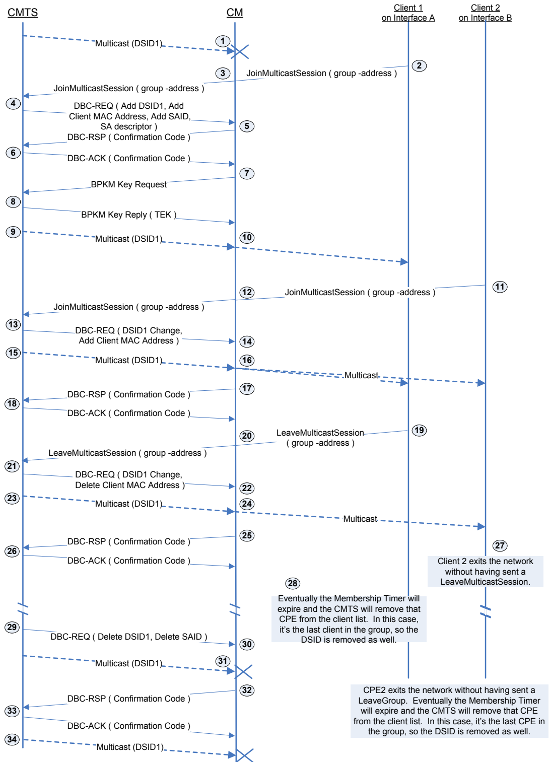
Figure 9-5 - Example: Encrypted Downstream Multicast Forwarding 296
