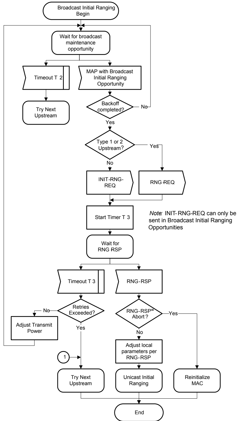
Figure 10-12 - Broadcast Initial Ranging – CM 316
