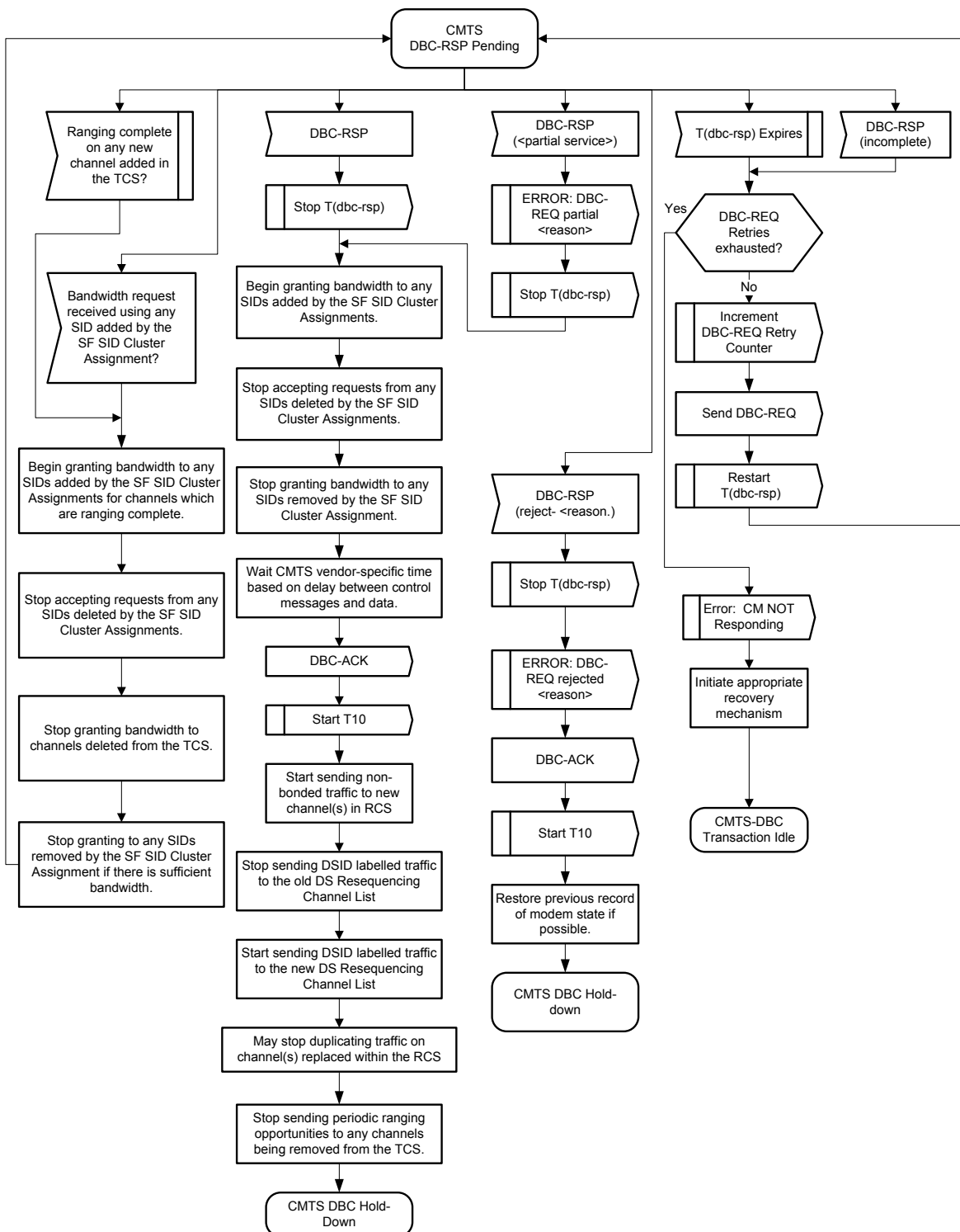
Figure 11-52 - CMTS DBC-RSP Pending 425
