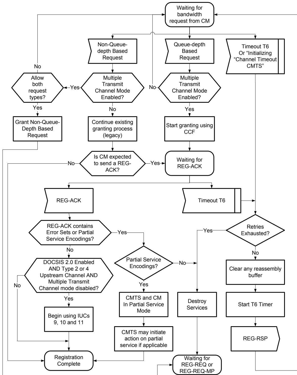
Figure 10-33 - CMTS Registration - End 366
