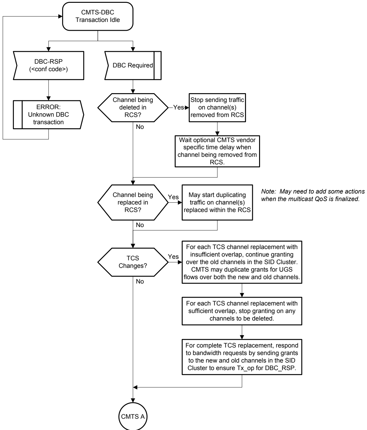
Figure 11–50 - CMTS DBC Request (part 1) 423
