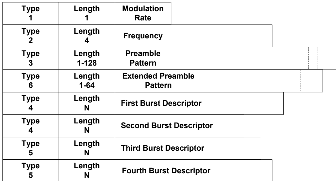
Figure 6–17 - Example of UCD Encoded TLV Data
