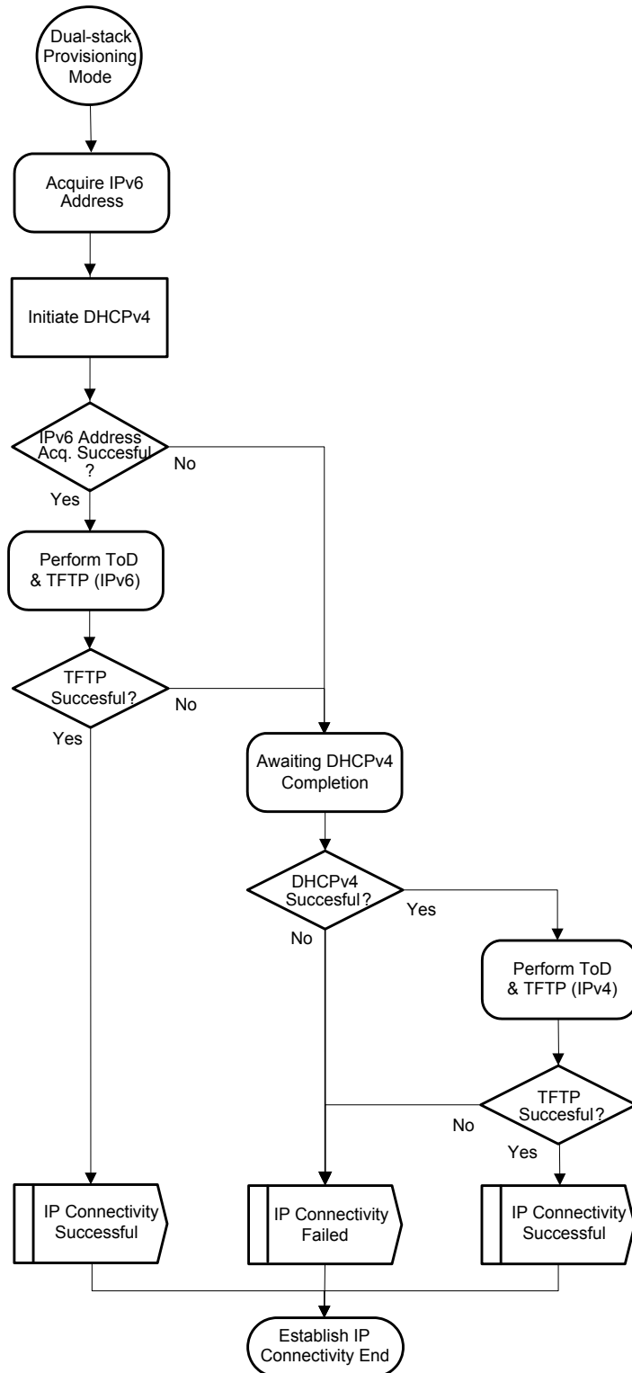
Figure 10–20 - Dual-stack Provisioning Mode 320
