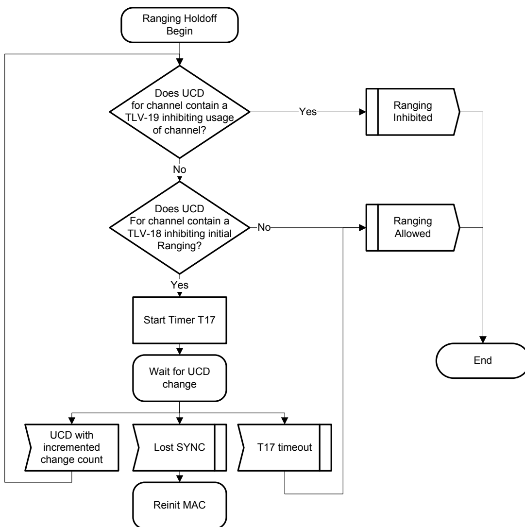
Figure 10–5 - Ranging Holdoff
