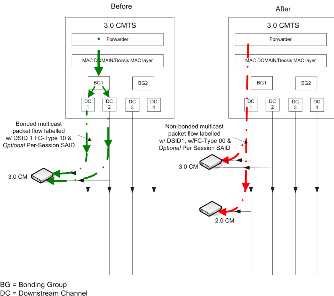
Figure VIII-4 - Multicast Session Replication to clients behind both a 3.0 CM and a 2.0 CM on the same downstream channel (Subcase 1)
