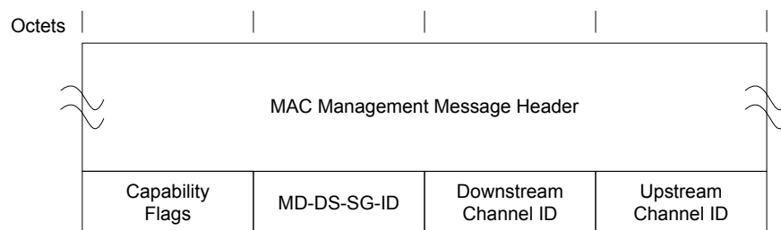
Figure 6–22 - B-INIT-RNG-REQ Format 79
