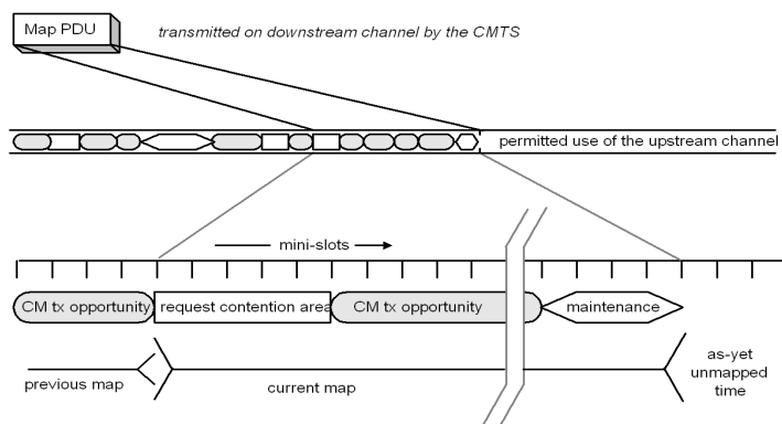
Figure 7-1 - Allocation Map
