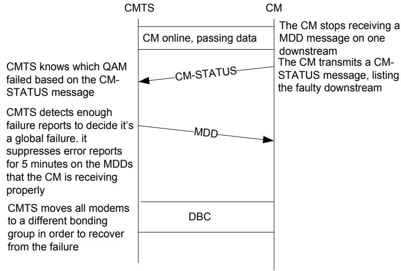
Figure V-2 - Example 2 - Option 4 729
