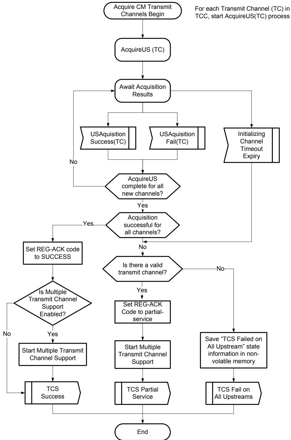
Figure 10–28 - CM Acquires Transmit Channels 353
