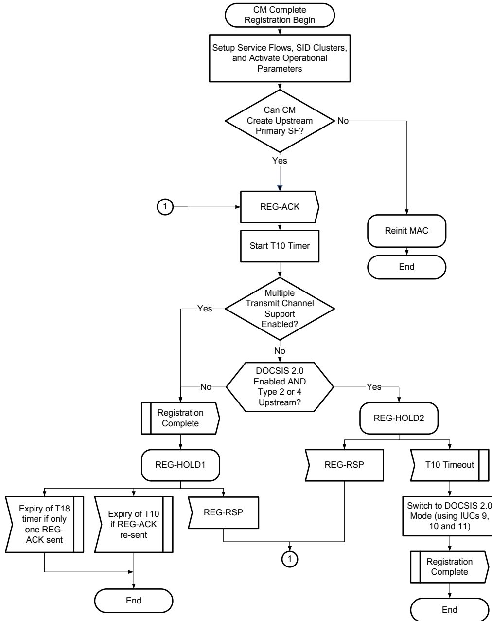
Figure 10-30 - CM Completes Registration 355
