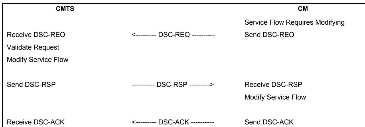
Figure 11–20 - CM-Initiated DSC
