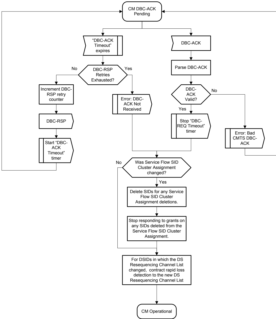
Figure 11-59 - CM DBC-ACK Pending 432
