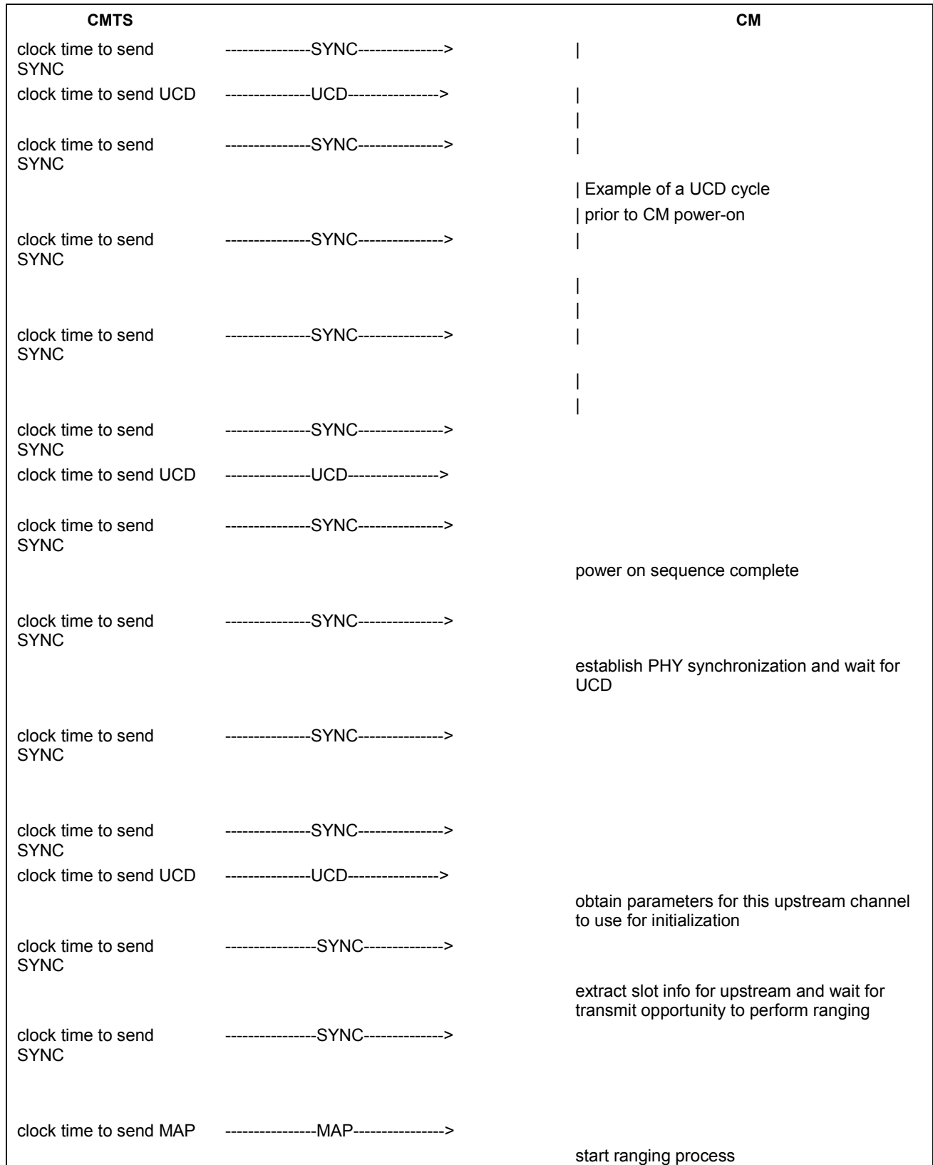
Figure 10–10 - Message Flows During Scanning and Upstream Parameter Acquisition
