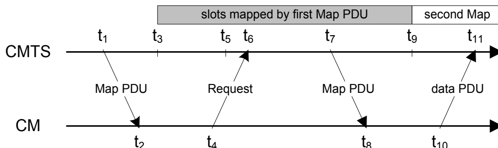
Figure 7–2 - Protocol Example
