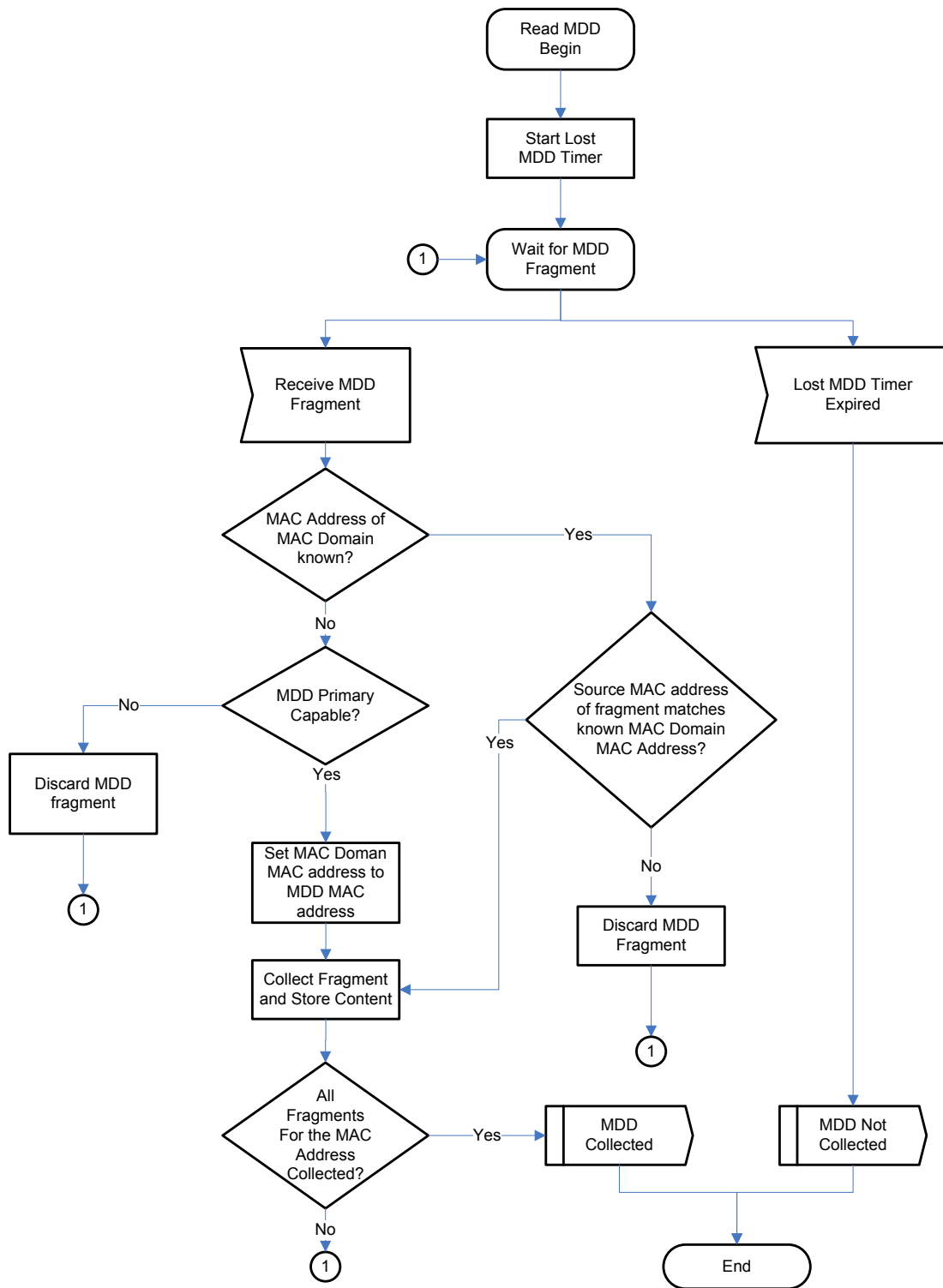
Figure 10-3 - Read MAC Domain Descriptor (MDD) 307
