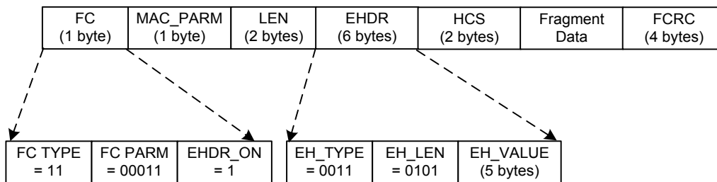
Figure 6–8 - Fragmentation MAC Header Format
