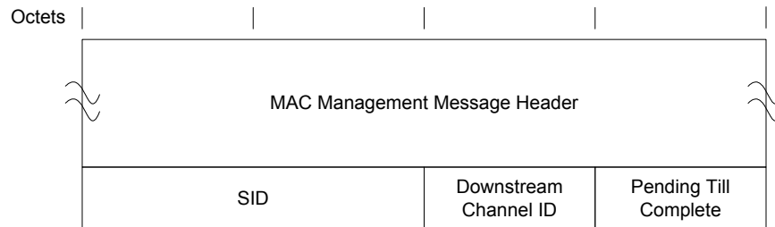
Figure 6–20 - RNG-REQ Format 74
