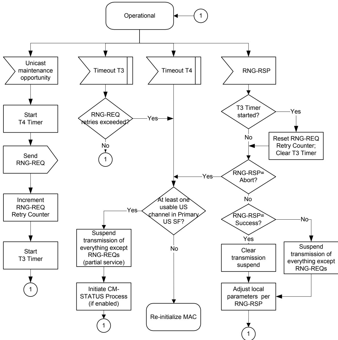
Figure 10-35 - Periodic Ranging - CM View 371
