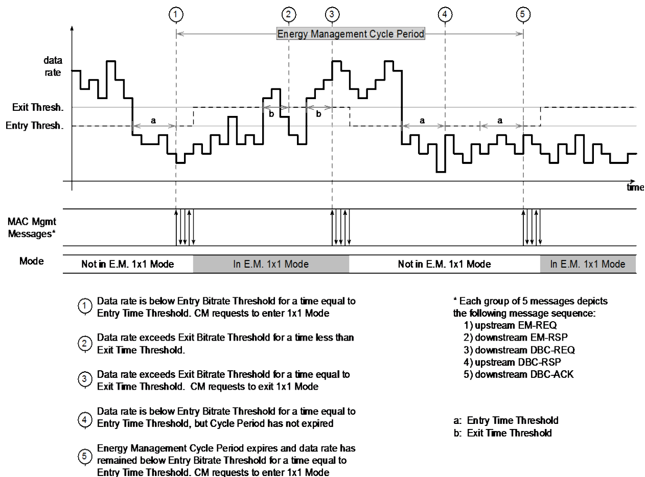
Figure 11-61 - Example Energy Management 1x1 Feature Operation
