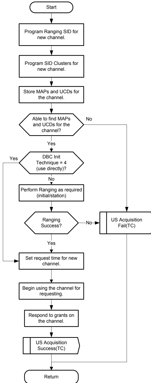
Figure 11–58 - CM AcquireUS Procedure 431
