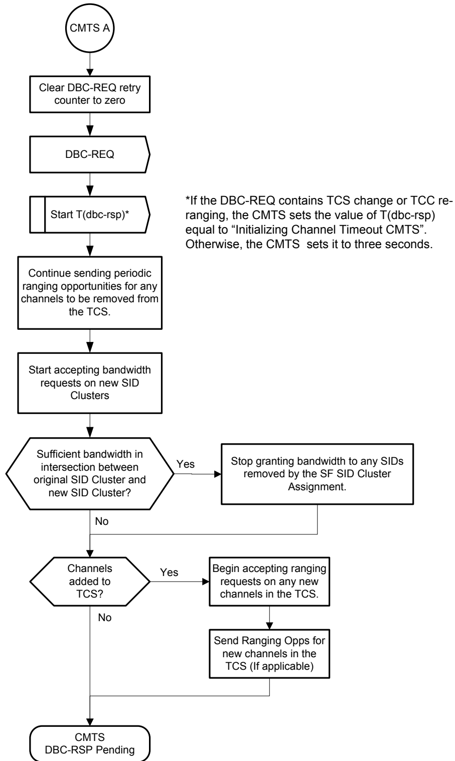
Figure 11-51 - CMTS DBC Request (part 2) 424
