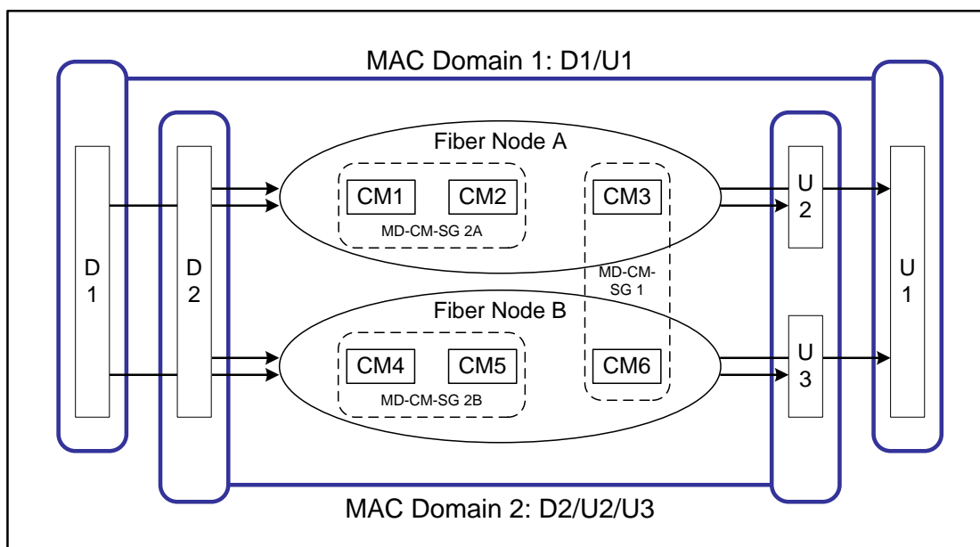
Figure 5–12 - Multiple MAC Domains per Fiber Node
