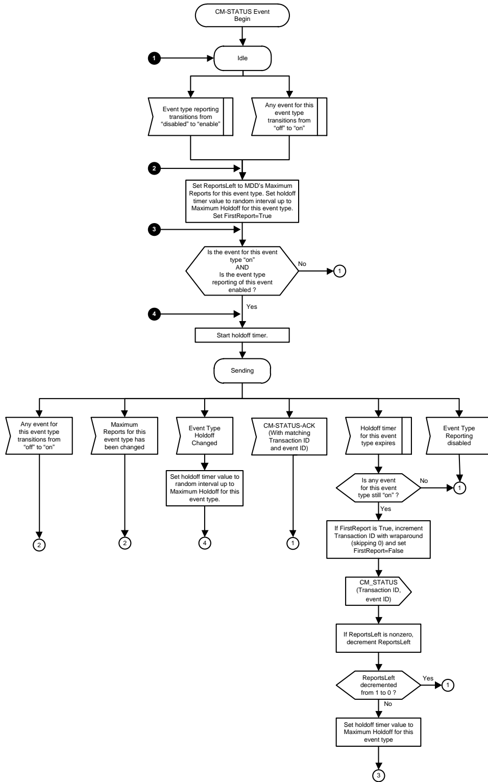
Figure 10-46 - CM-STATUS Event Type State Machine 144
