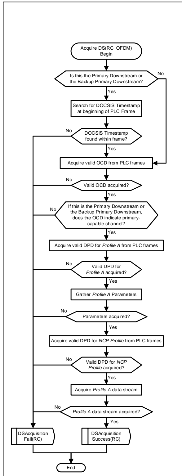
Figure 10-29 - CM Acquires OFDM Downstream Channel
