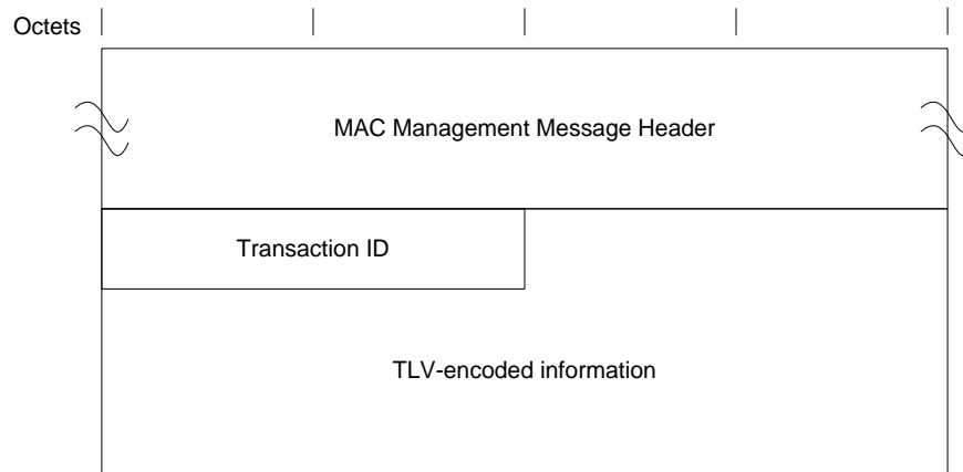
Figure 6–67 - DTP Request Message
