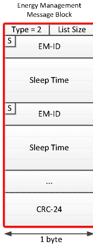
Figure 6–74 - Energy Management Message Block
