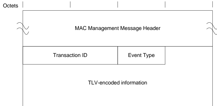
Figure 6–55 - CM-STATUS Report
