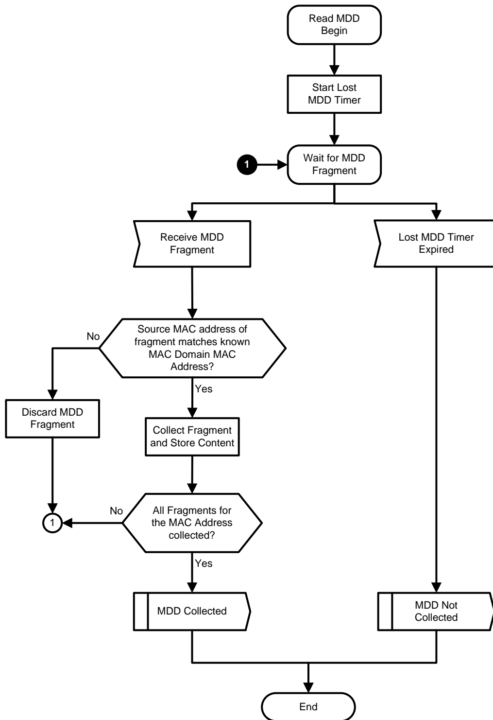
Figure 10-5 - Read MAC Domain Descriptor (MDD)
