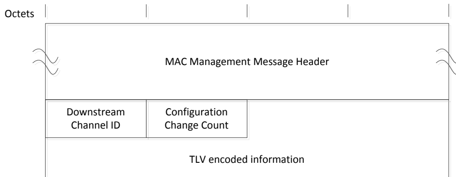
Figure 6–61 - OFDM Channel Descriptor
