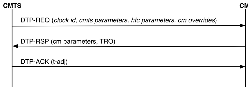
Figure 10–53 - CMTS is DTP Master
