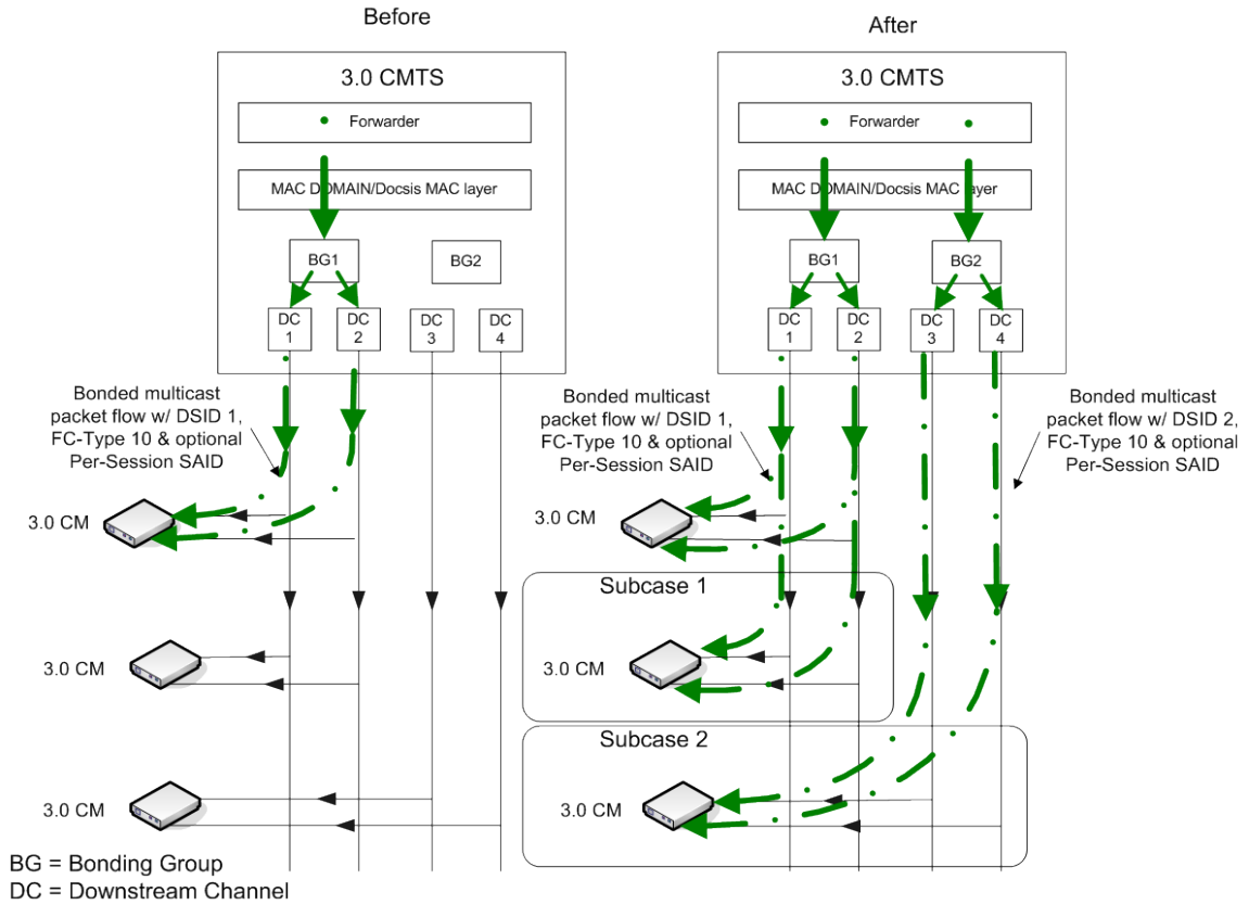
Figure VIII-8 - Multicast Session Replication to Clients Behind Two 3.0 CMs
