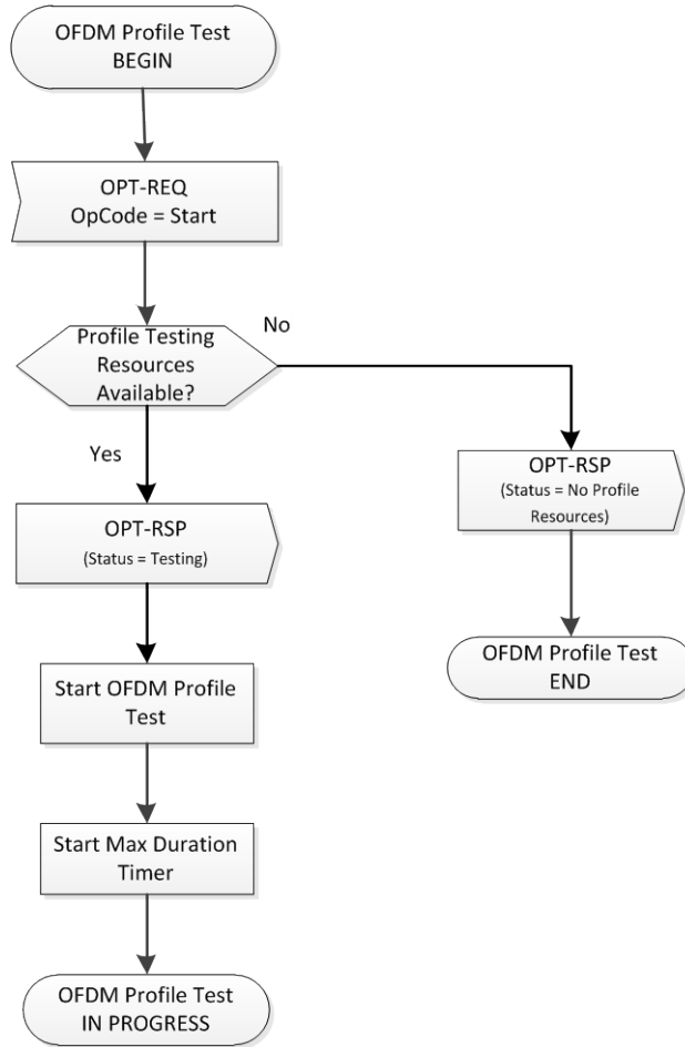
Figure 10–40 - CM OPT State Machine - OPT Idle
