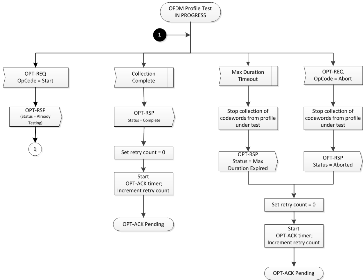
Figure 10-41 - CM OPT State Machine - OFDM Profile Test in Progress
