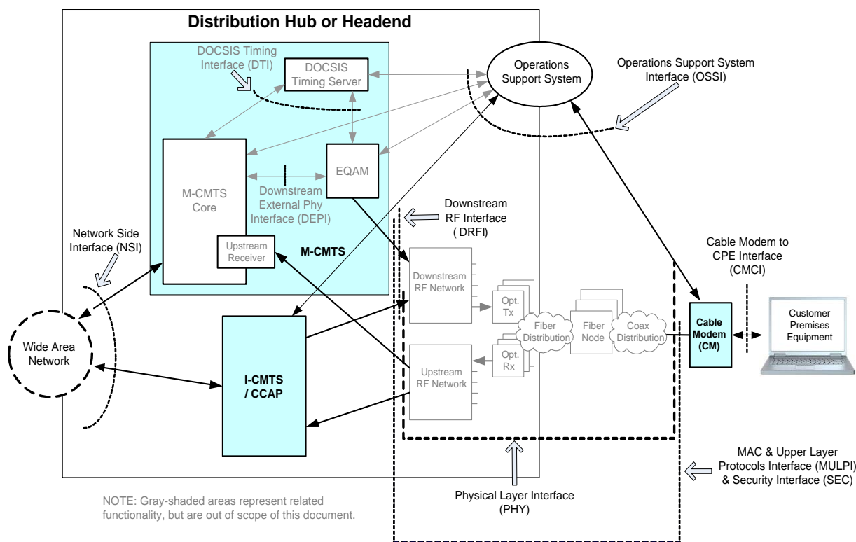
Figure 1-3 - Data-Over-Cable Reference Architecture
