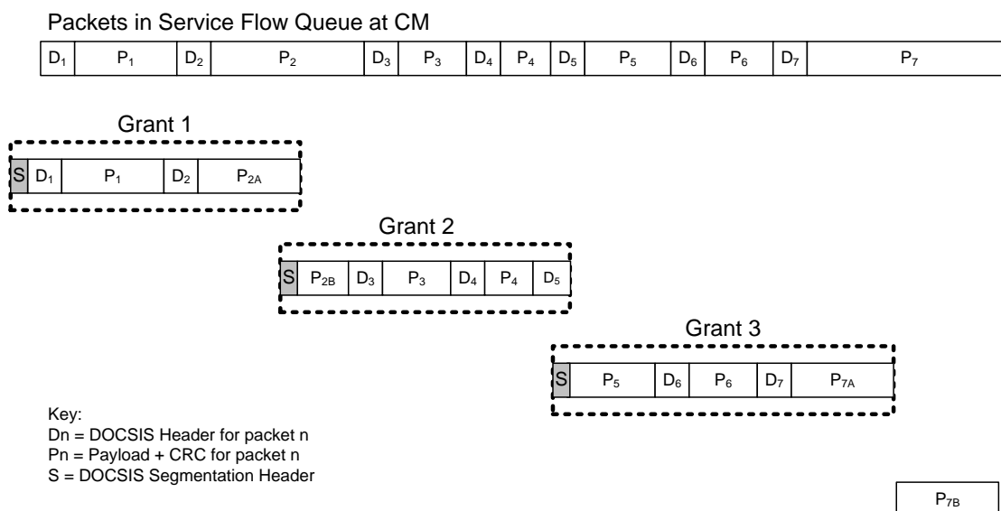
Figure 7-8 - CCF Using Segment Headers
