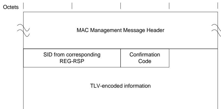
Figure 6–37 - Registration Acknowledgment
