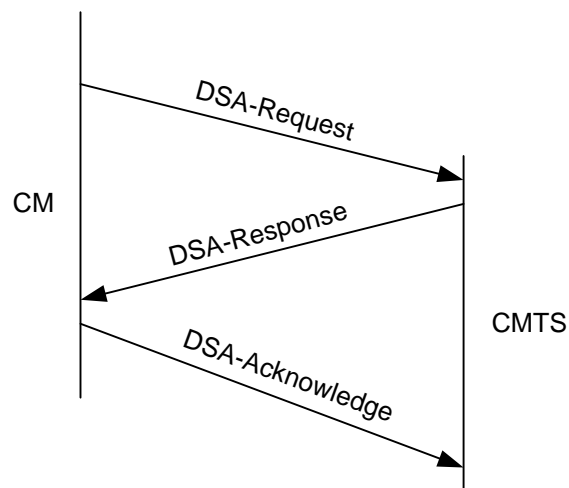
Figure 7–14 - Dynamic Service Addition Message Flow - CM Initiated
