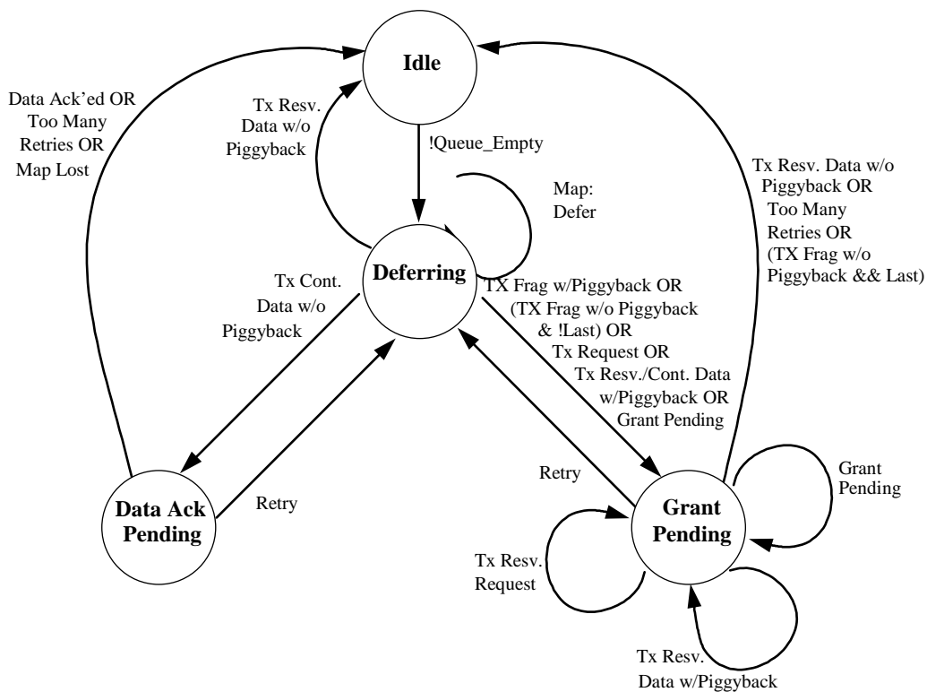
Figure III-2 - Transmission and Deferral State Transition Diagram
