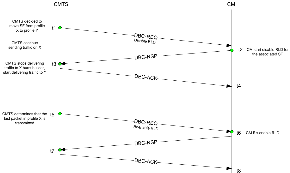
Figure XII-3 - DBC procedure for SF profile switch on OFDM channel
