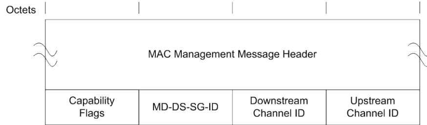
Figure 6–27 - B-INIT-RNG-REQ Format
