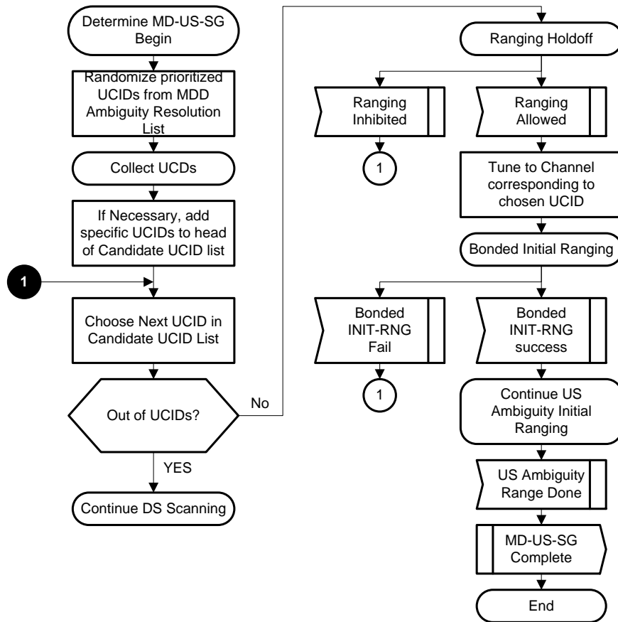
Figure 10–7 - Determine MD-US-SG
