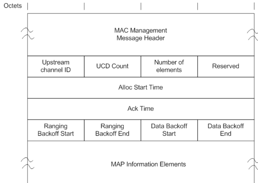
Figure 6–19 - Version 1 MAP Format
