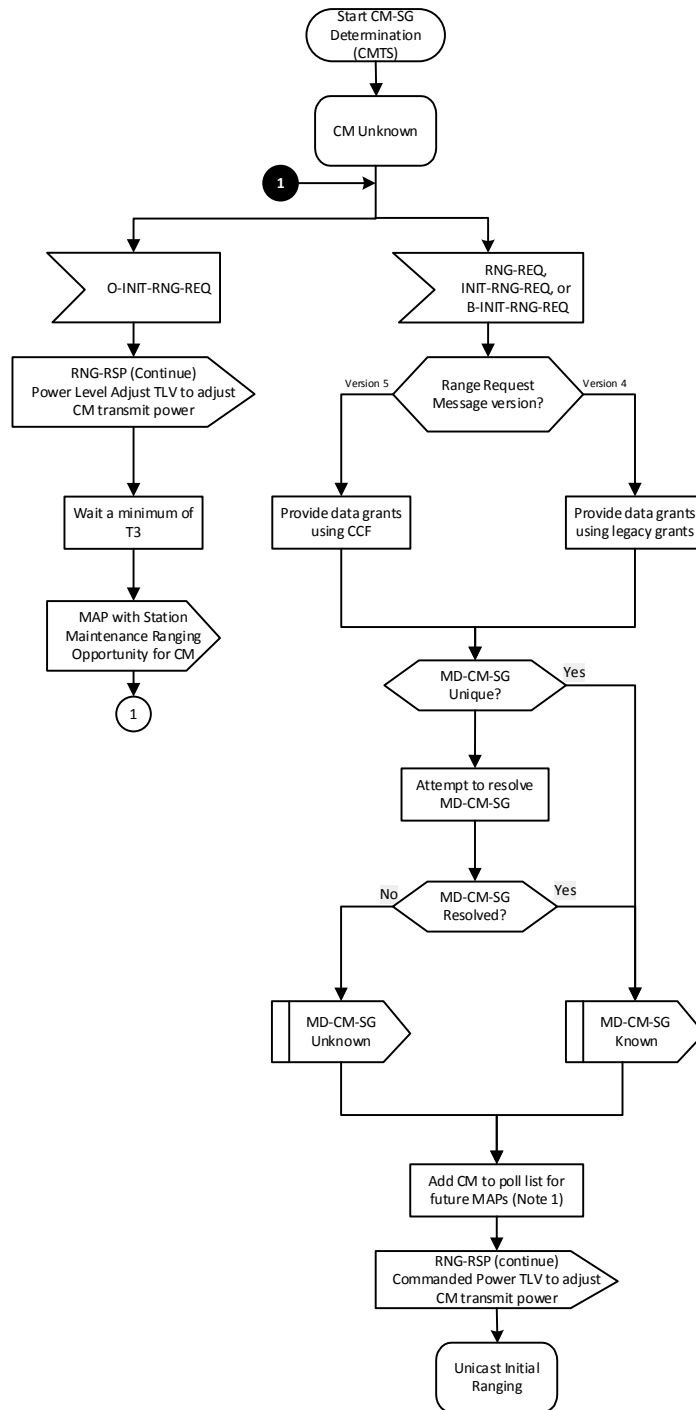
Figure 10–15 - CM-SG Determination - CMTS 121
