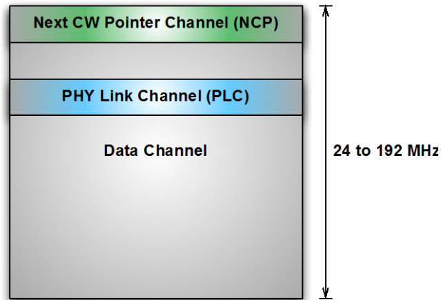
Figure 6–71 - OFDM Channel with PLC Prior to Interleaving
