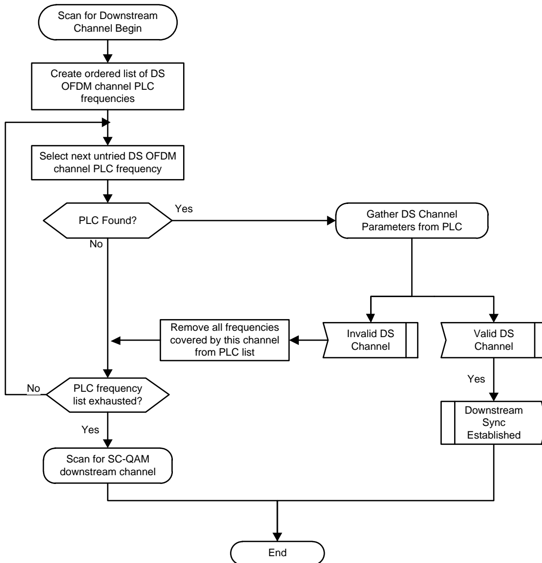
Figure 10–2 - Scan for Downstream Channel
