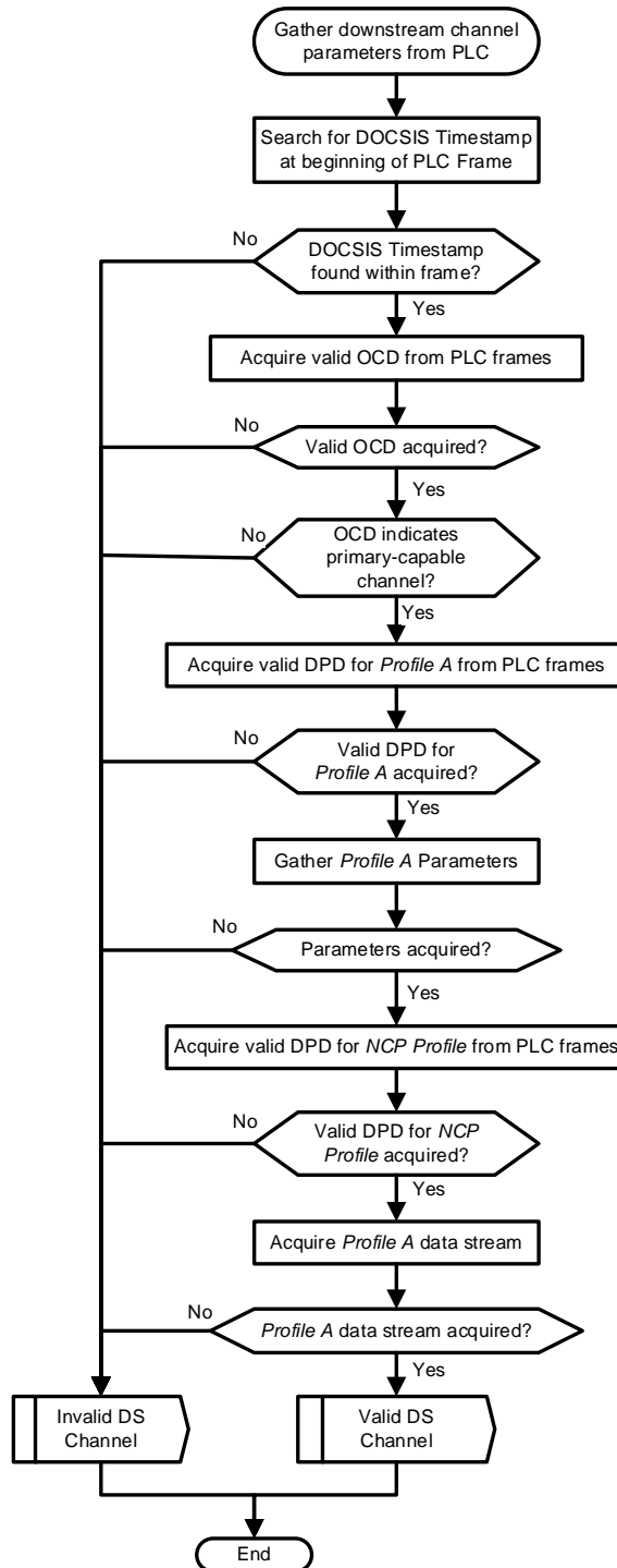
Figure 10–3 - Gather Downstream Channel Parameters from PLC
