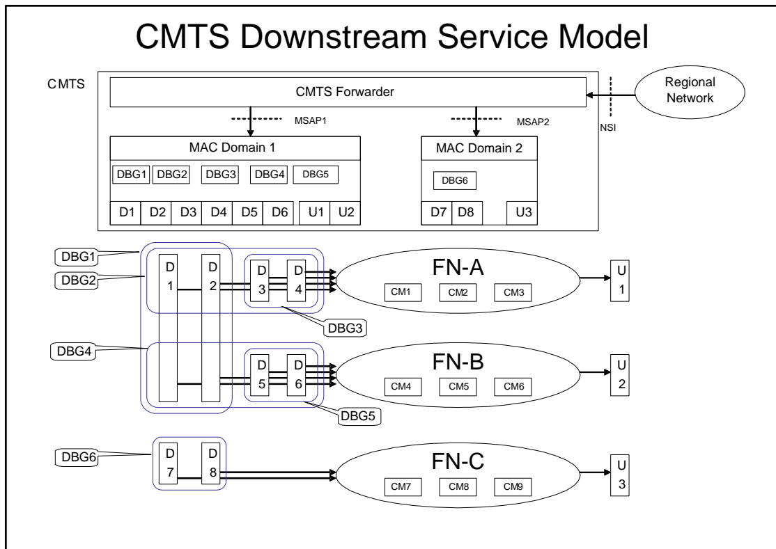
Figure 5–14 - CMTS Downstream Service Model
