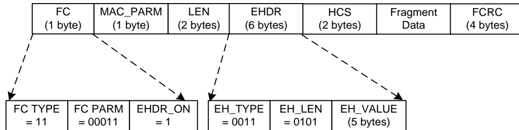
Figure 6–7 - Fragmentation MAC Header Format
