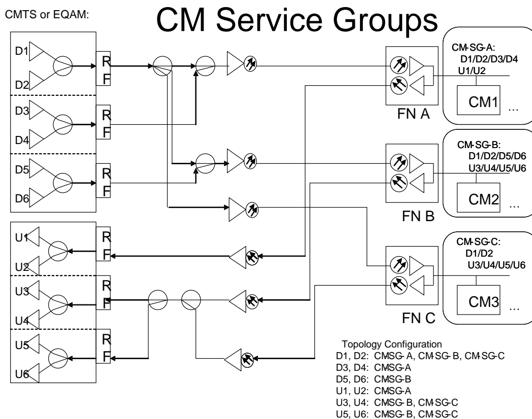
Figure 5–8 - CM Topology Configuration Example
