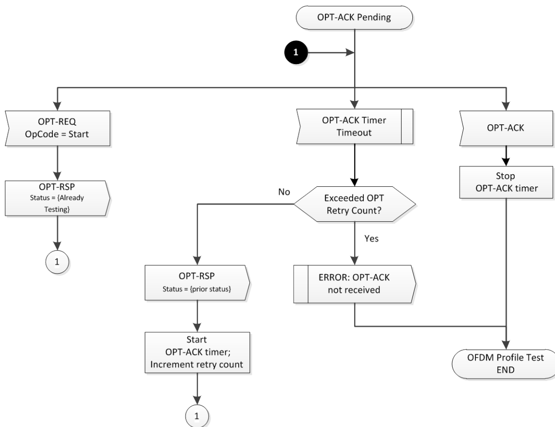
Figure 10–42 - CM OPT State Machine - OPT-ACK Pending
