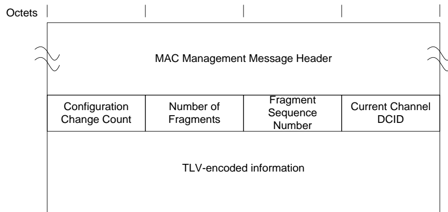
Figure 6–49 - MAC Domain Descriptor
