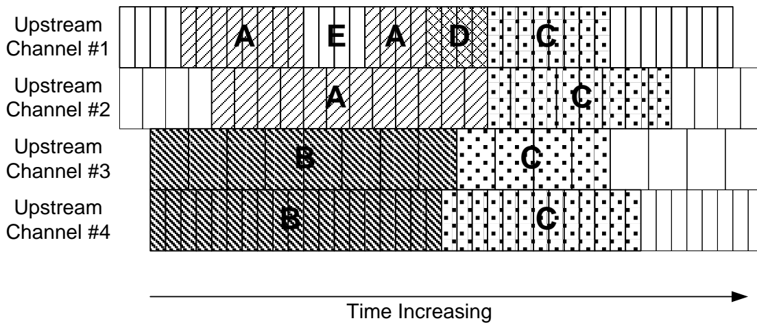
Figure 5–6 - Segmentation Example
