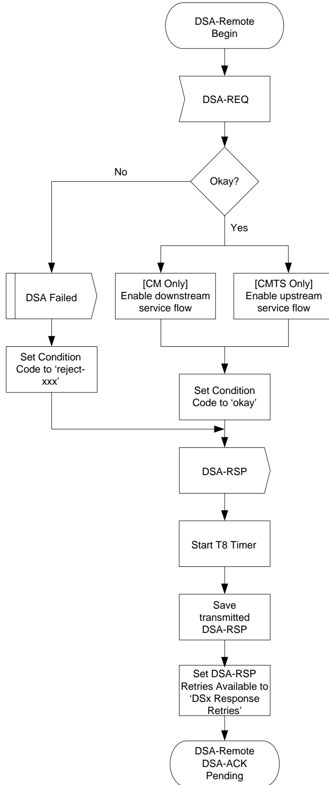
Figure 11–16 - DSA-Remotely Initiated Transaction Begin State Flow Diagram
