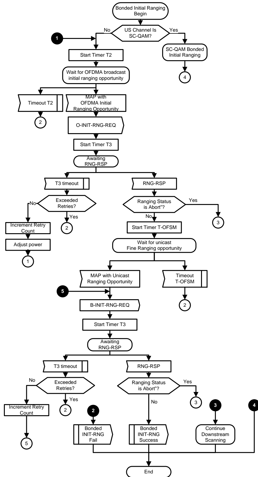
Figure 10-9 - Bonded Initial Ranging
