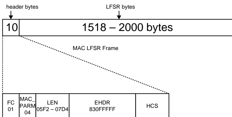
Figure 10–44 - MAC LFSR Frame
