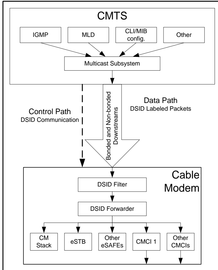
Figure 9-2 - Multicast Model
