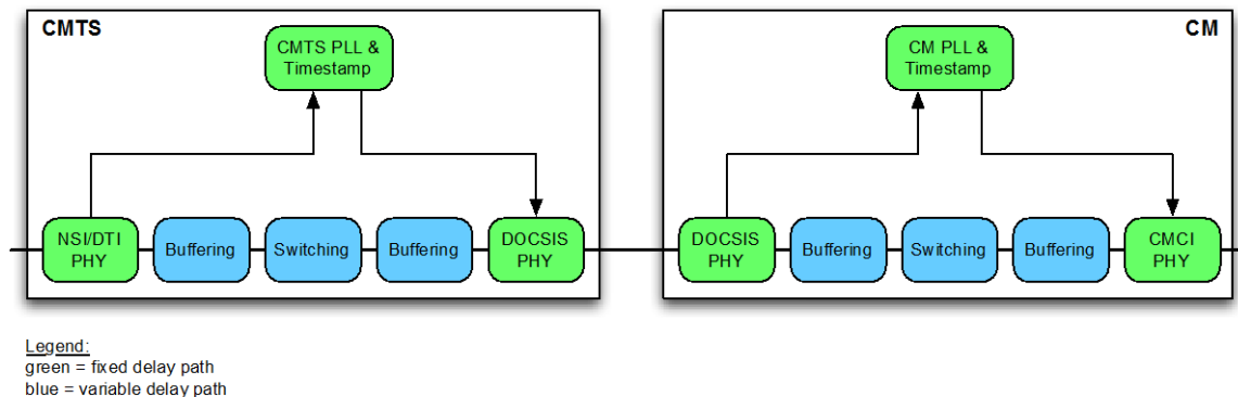
Figure 10-49 - DOCSIS Time Protocol Fixed Latency Path Example
