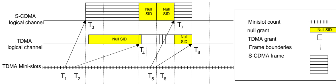
Figure 7-4 - Logical S-CDMA and TDMA channels
