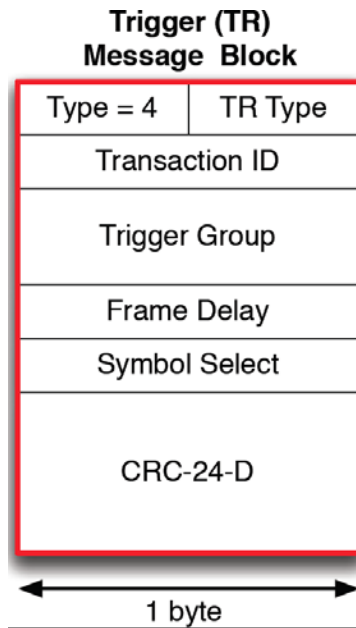
Figure 6–76 - Trigger Message Block
