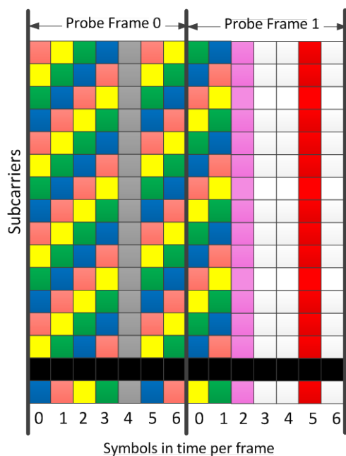
Figure 6-24 - Sample Probe Frame and P-IEs
