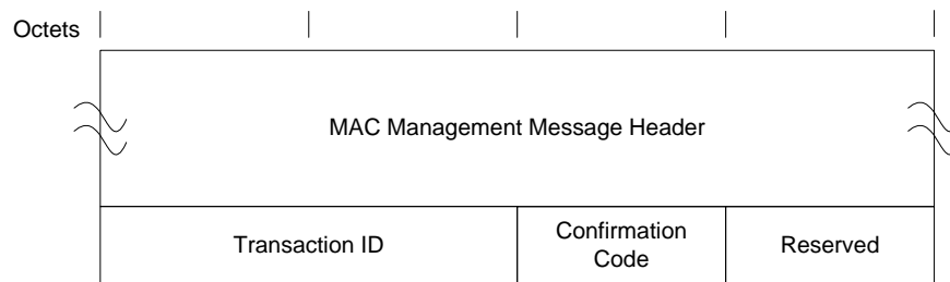
Figure 6–45 - Dynamic Service Deletion - Response
