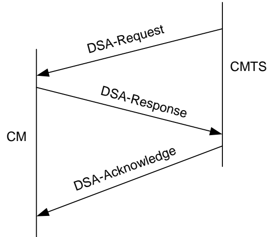
Figure 7–15 - Dynamic Service Addition Message Flow - CMTS Initiated
