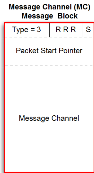
Figure 6-75 - Message Channel Message Block
