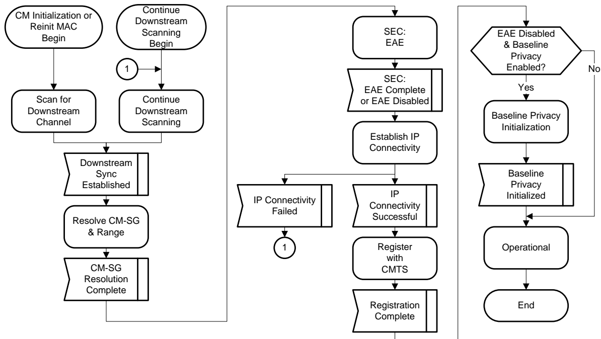
Figure 10–1 - Cable Modem Initialization Overview
