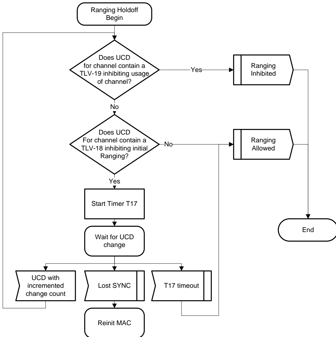
Figure 10–8 - Ranging Holdoff
