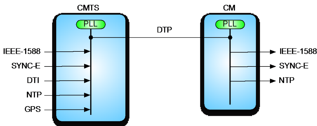
Figure 10–48 - DOCSIS Time Protocol System Overview
