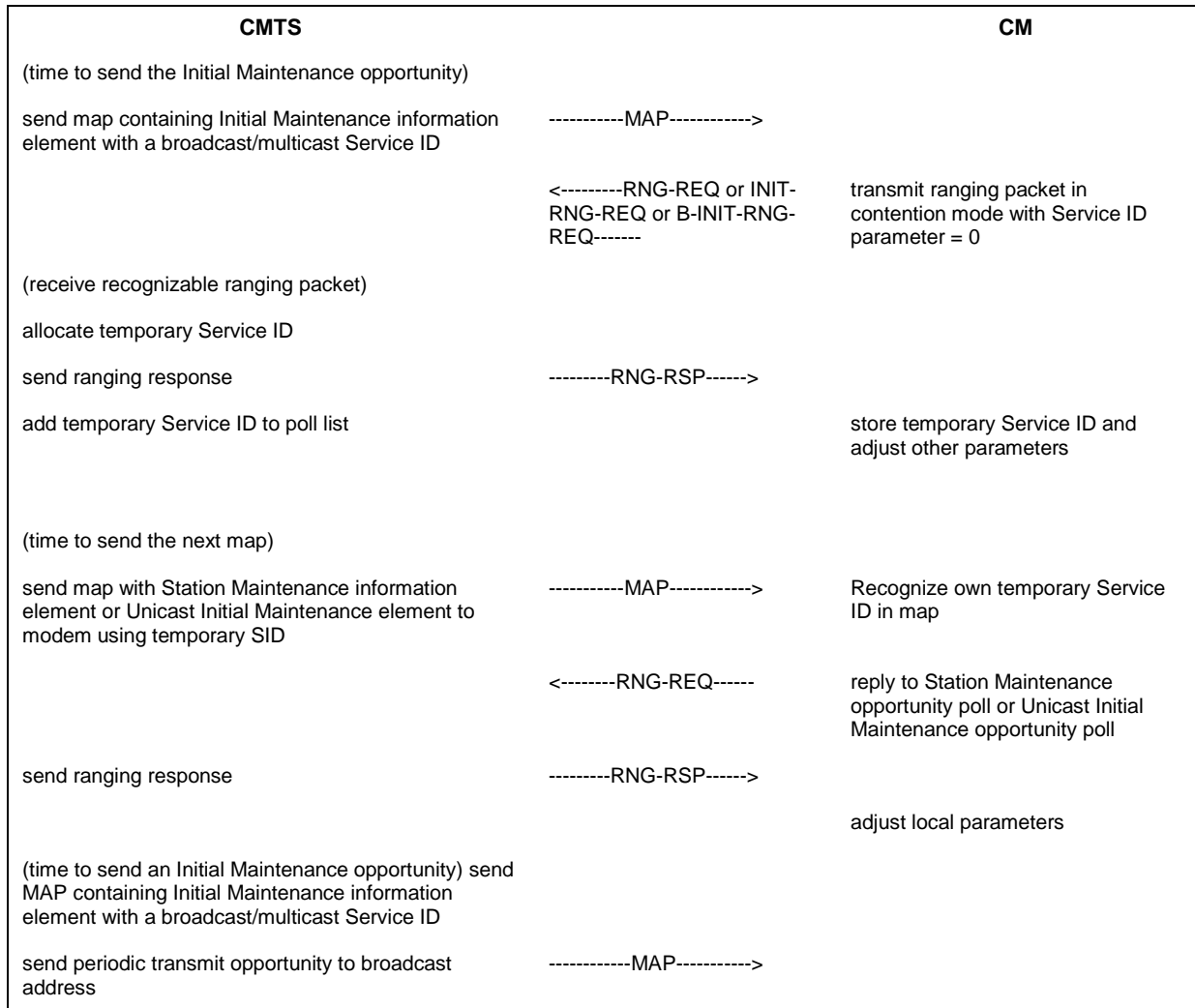
Figure 10–12 - Ranging and Automatic Adjustments Procedure for SC-QAM Upstreams
