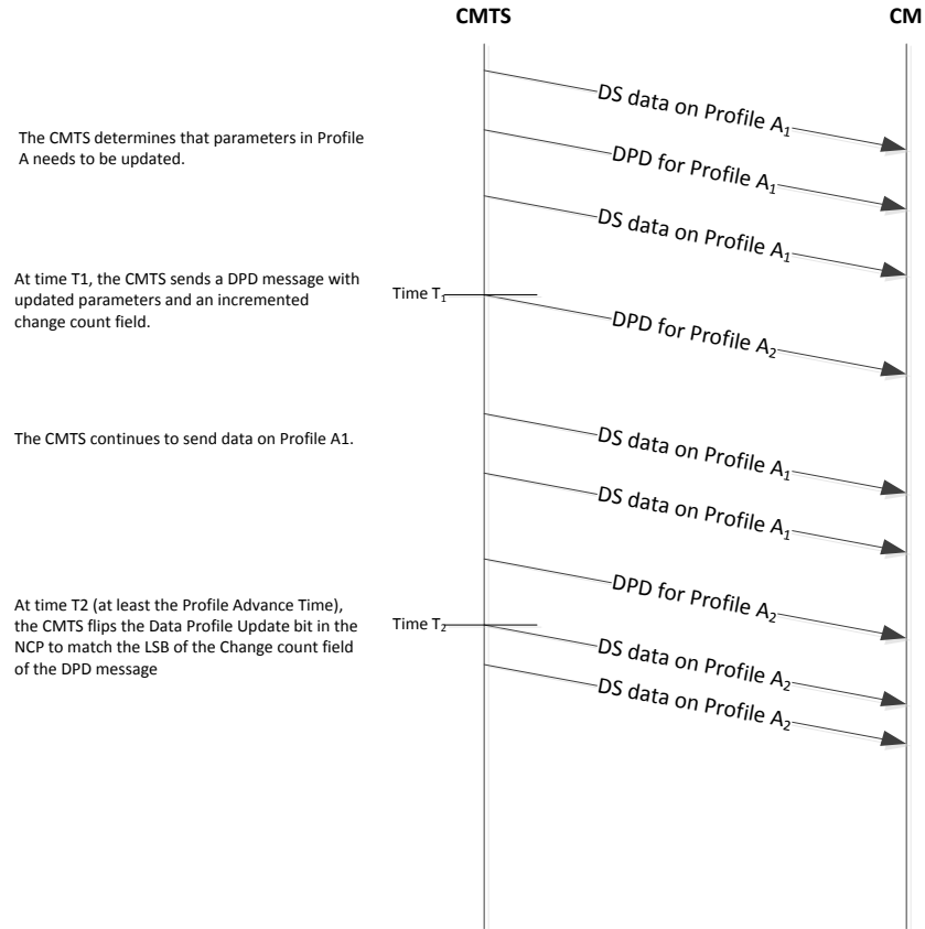
Figure XII-6 - DPD Change to Profile A
