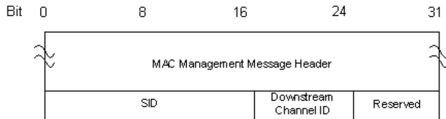
Figure 6–25 - RNG-REQ Format
