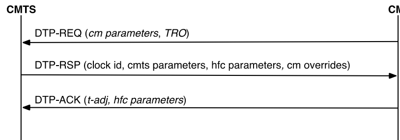
Figure 10–54 - CM is DTP Master
