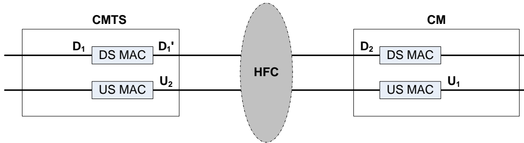
Figure 10–47 - DPV Reference Diagram
