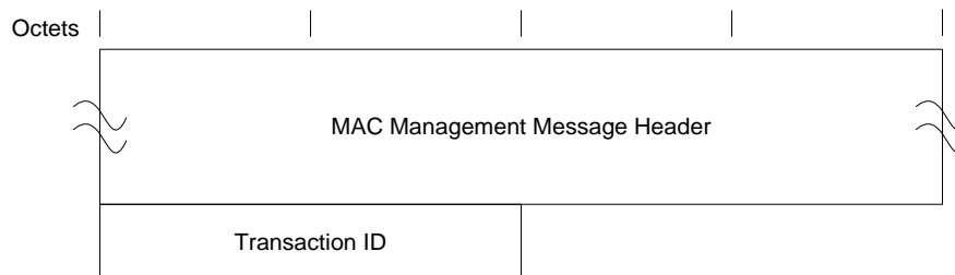
Figure 6–70 - DTP Acknowledge Message
