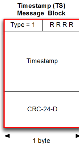
Figure 6–73 - Timestamp Message Block
