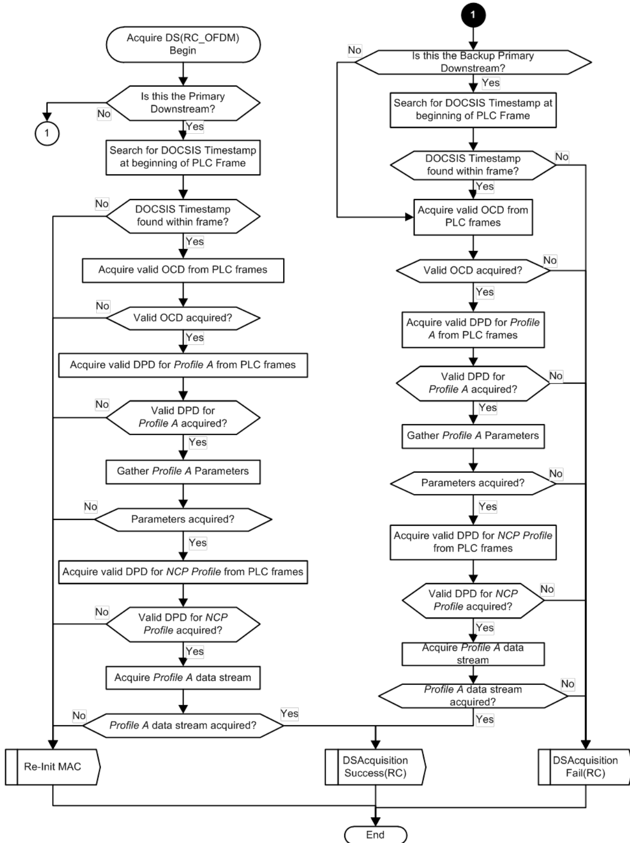
Figure 11-52 - CM Acquired DS Procedure for OFDM
