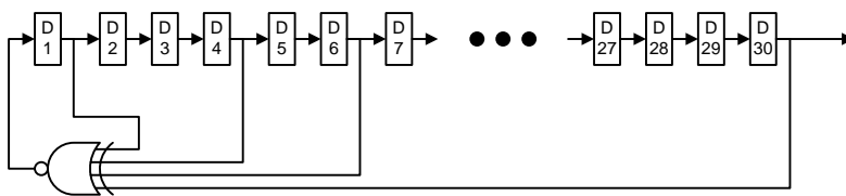
Figure 10–43 - Linear Feedback Shift Register for Synthetic Data Generation
