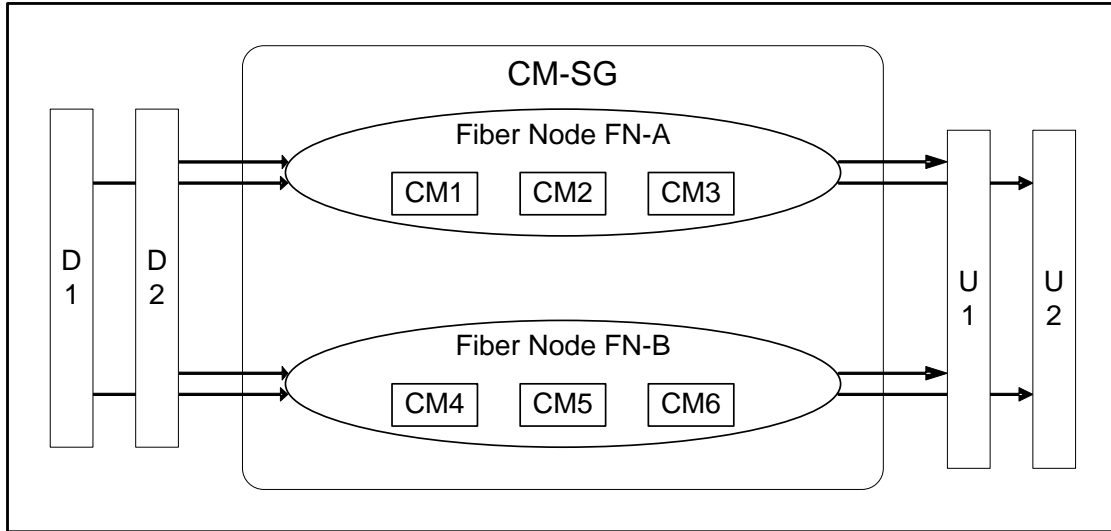
Figure 5–10 - Multiple Fiber Nodes per CM-SG
