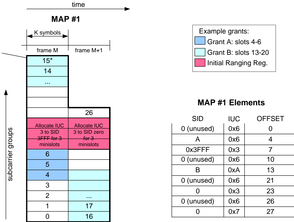
Figure 7-7 - Example MAP for Initial Ranging Region on an OFDMA Channel
