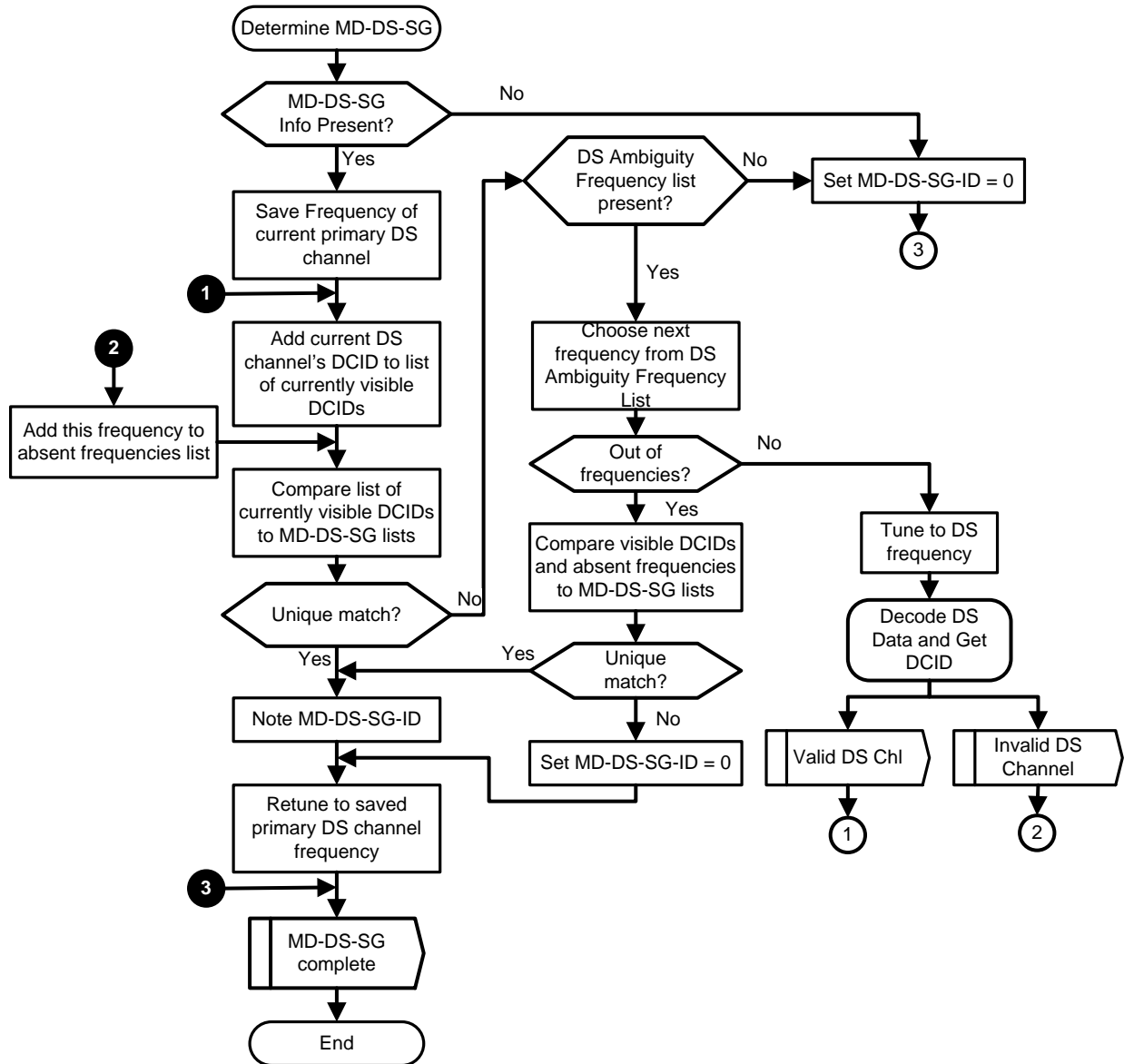
Figure 10-6 - Determine MD-DS-SG
