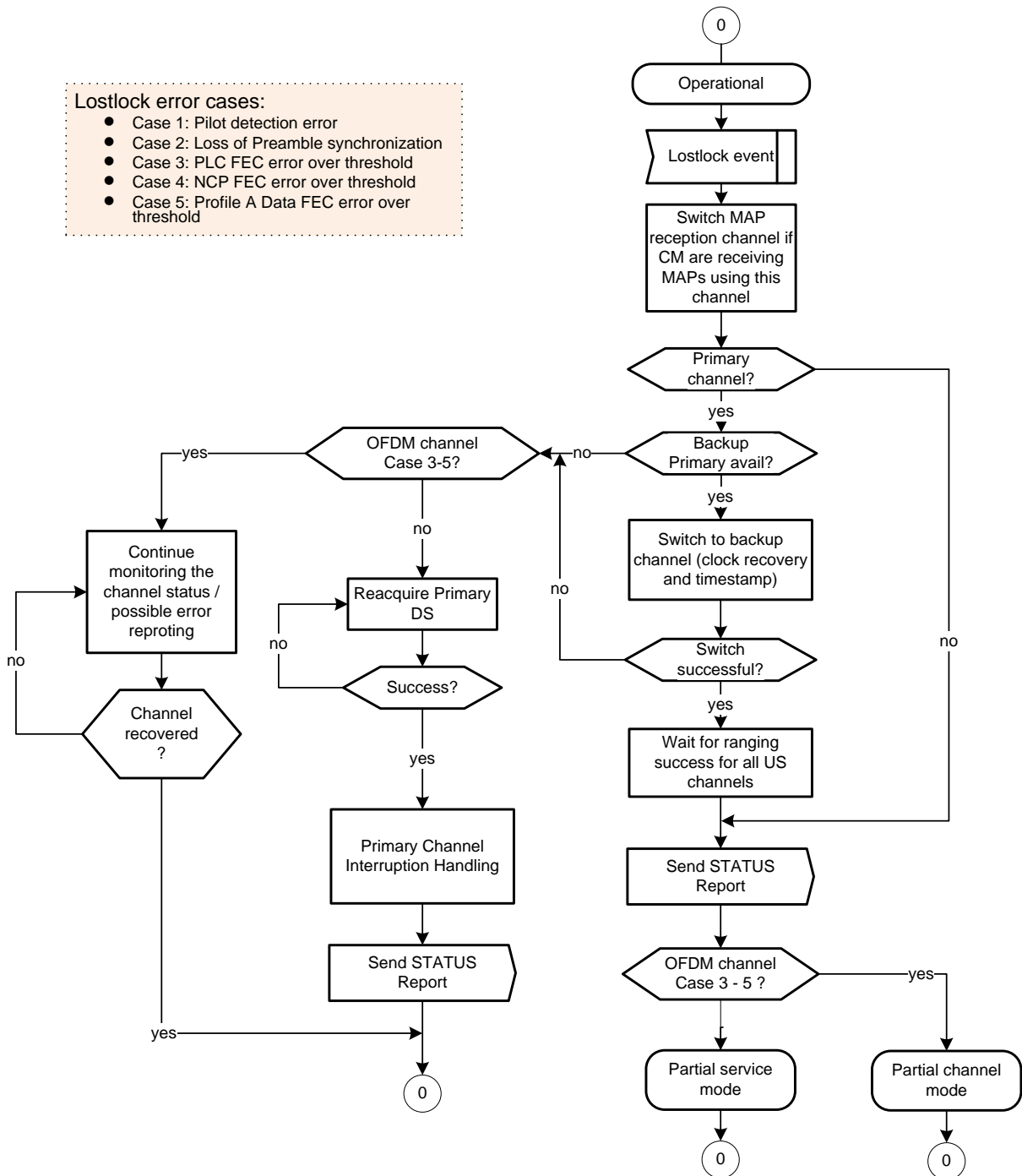
Figure 10-45 - Lost Lock on an OFDM Channel Procedure 139
