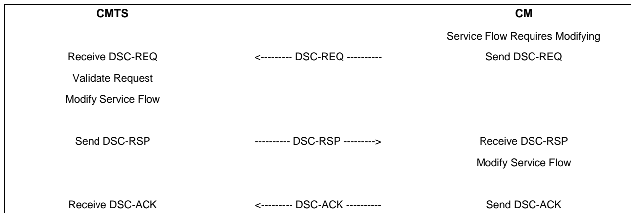
Figure 11–20 - CM-Initiated DSC
