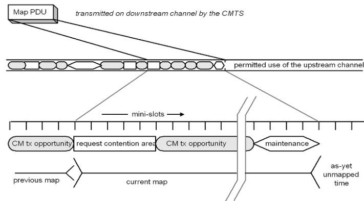
Figure 7-2 - Allocation Map
