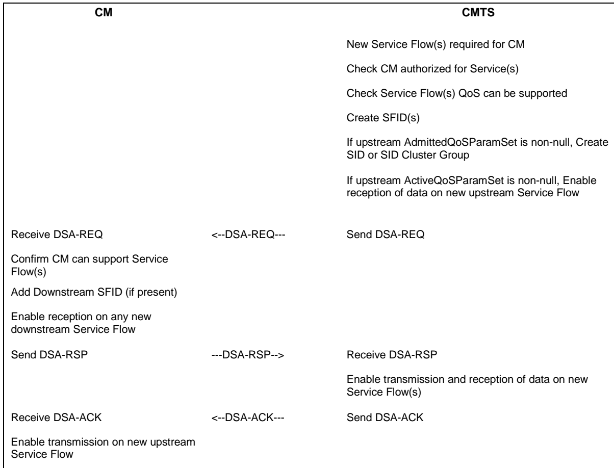
Figure 11–10 - Dynamic Service Addition Initiated from CMTS
