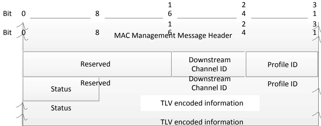
Figure 6–65 - The OFDM Profile Test Response (OPT-RSP) message
