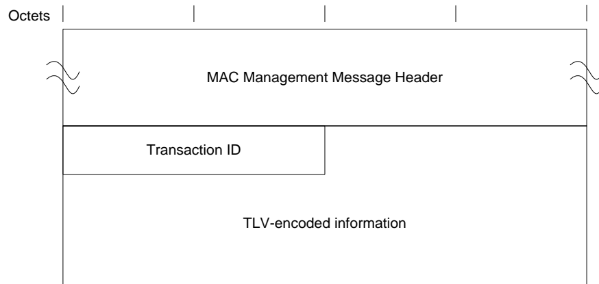
Figure 6-48 - Dynamic Channel Change Acknowledge
