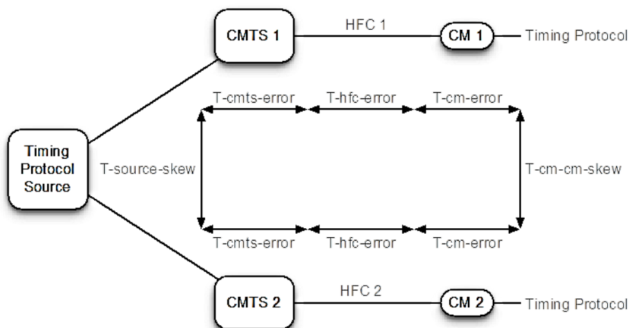
Figure 10–55 - DTP System Performance
