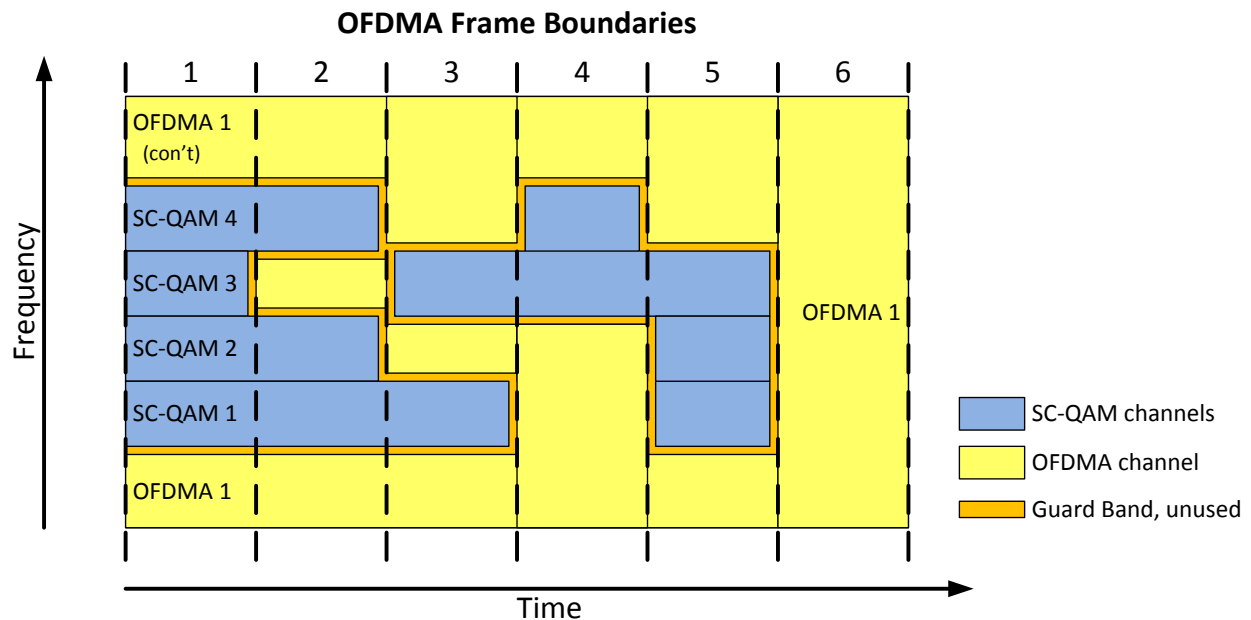
Figure 5–7 - Upstream Time and Frequency Multiplexing
