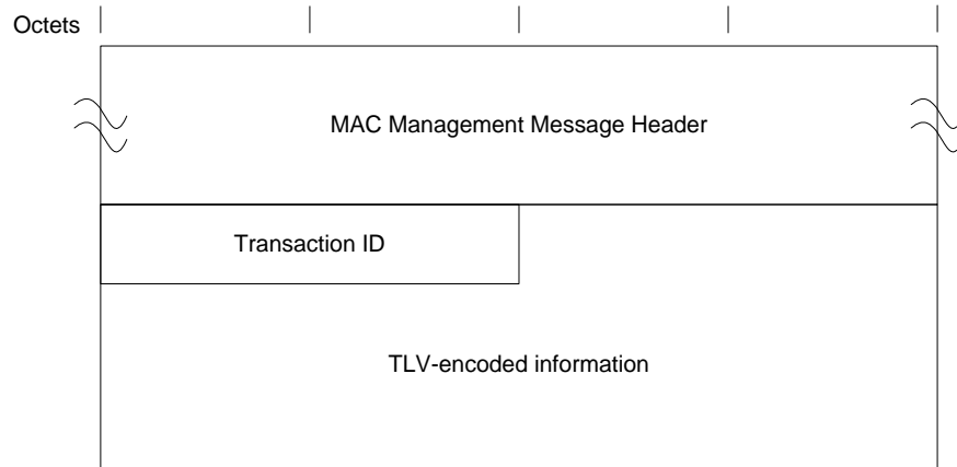
Figure 6–68 - DTP Response Message
