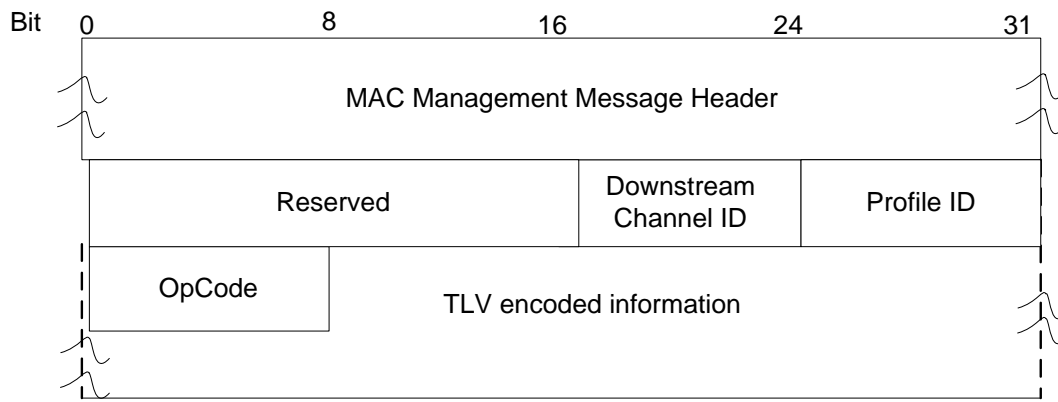
Figure 6–64 - The OFDM Downstream Profile Test Request (OPT-REQ) message
