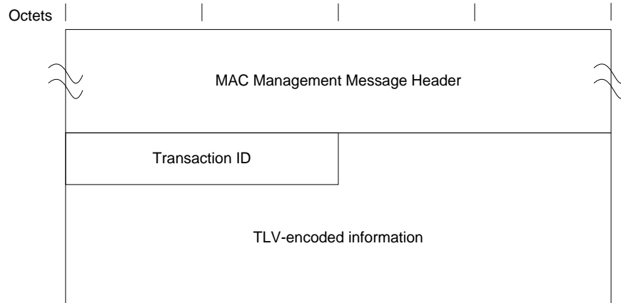
Figure 6–56 - CM-CTRL-REQ
