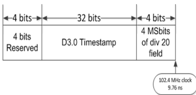
Figure 6–15 - OFDMA Timestamp Snapshot subTLV relationship to the Extended Timestamp
