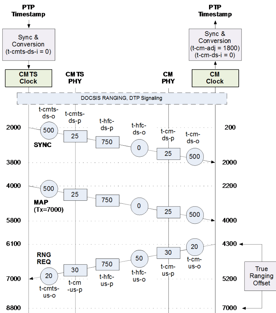
Figure 10–52 - True Ranging Offset Example
