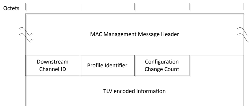
Figure 6–62 - Downstream Profile Descriptor
