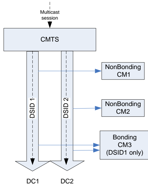
Figure 9–3 - DSIDs prevent duplication of non-bonded replications
