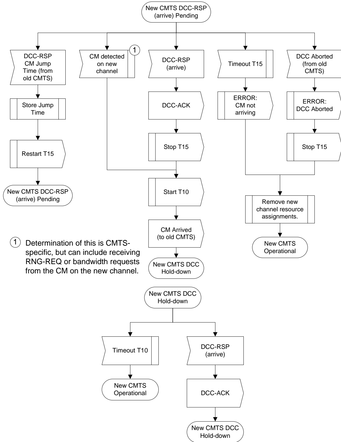
Figure 11-42 - Dynamically Changing Channels: CMTS View Part 4
