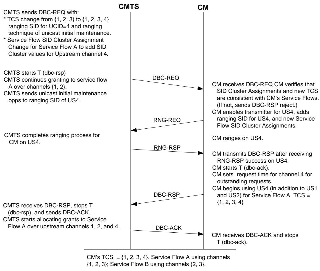
Figure XII–1 - Adding a Channel to the TCS and making a Service Flow SID Cluster Assignment
