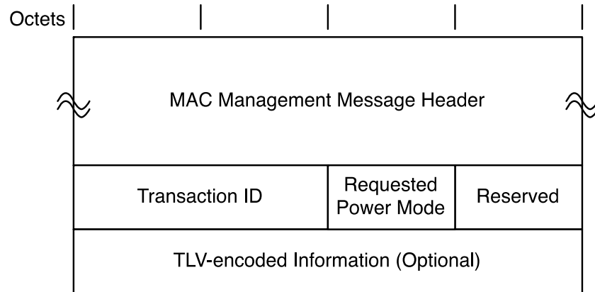
Figure 6–58 - Energy Management Request Message
