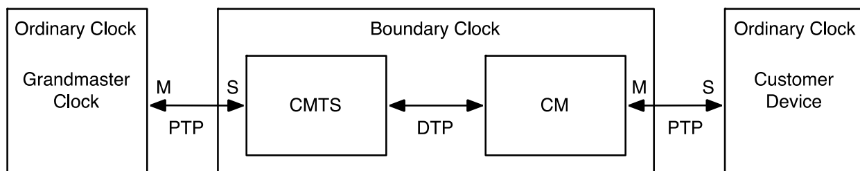
Figure 10-50 - DTP/PTP Reference Architecture
