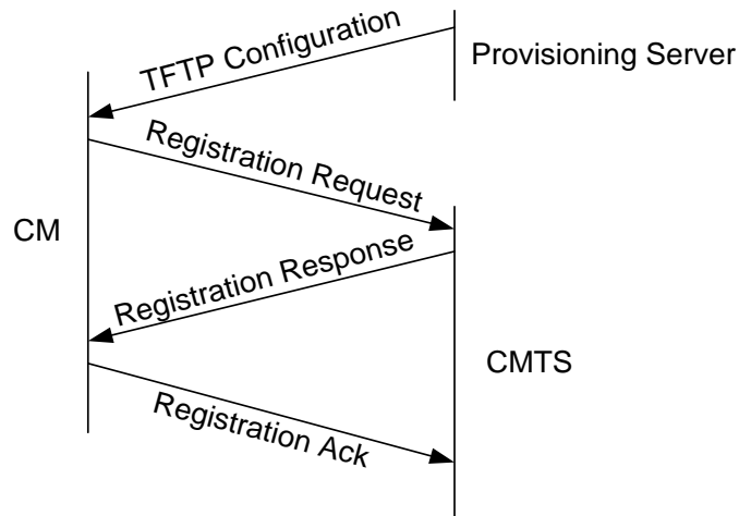
Figure 7-13 - Registration Message Flow
