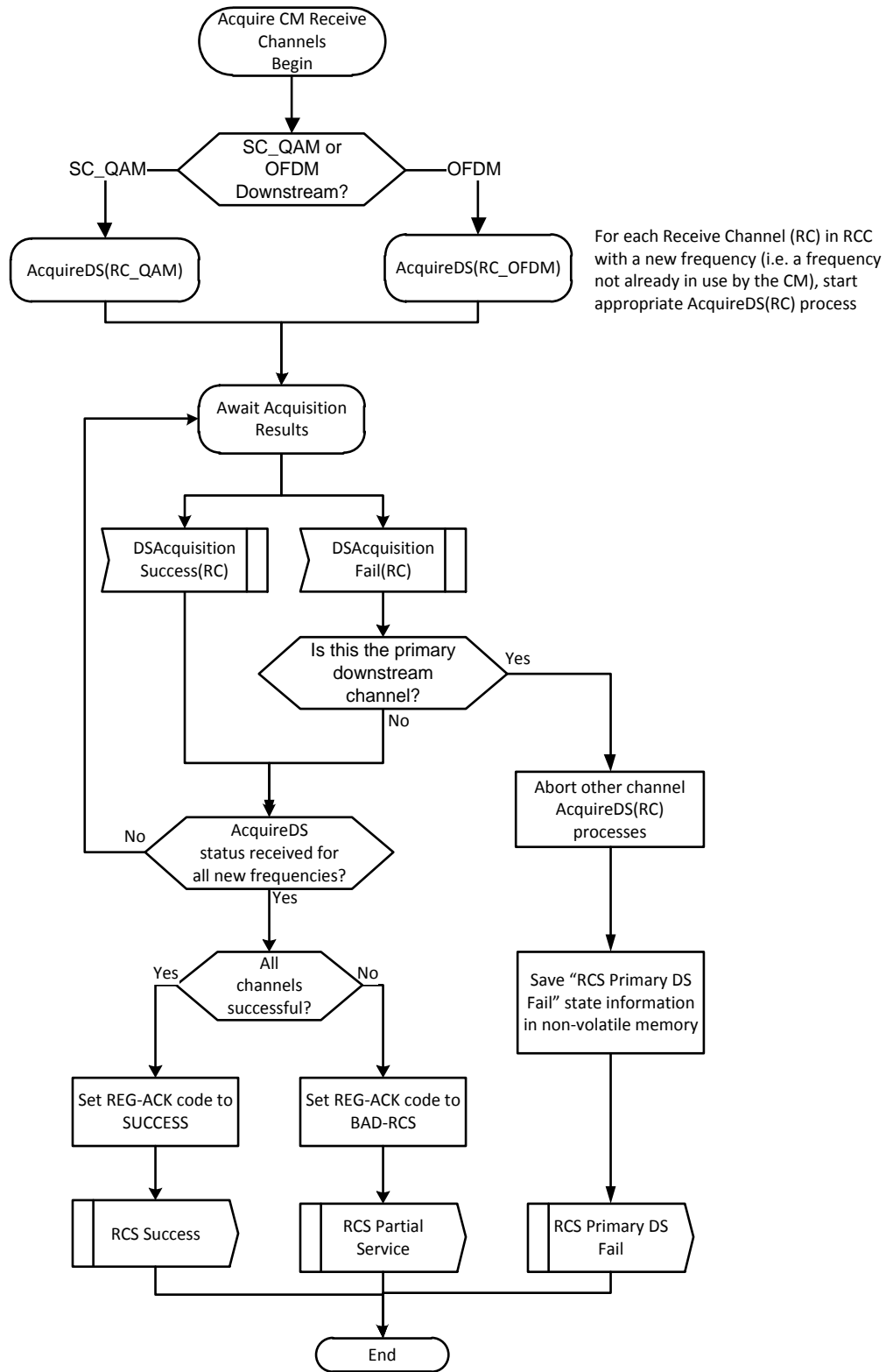
Figure 10-27 - CM Acquires Receive Channels
