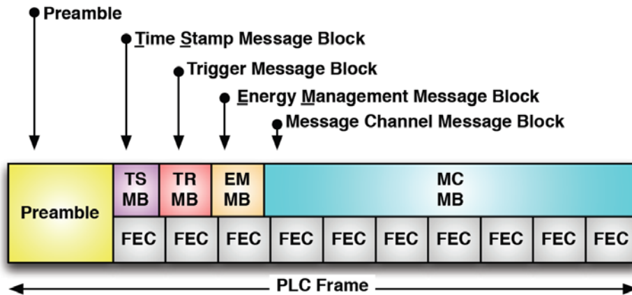
Figure 6–72 - PLC Frame
