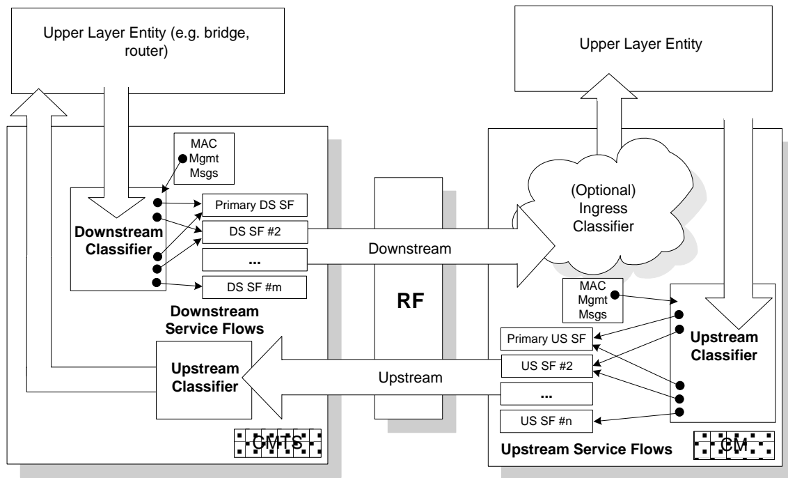
Figure 7–11 - Classification within the MAC Layer
