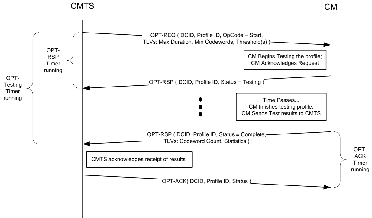
Figure 10–38 - Typical OFDM Profile Test Transaction
