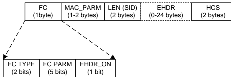
Figure 6–2 - MAC Header Format
