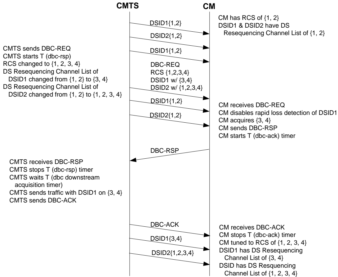
Figure XII–2 - Changing the RCS and Downstream Resequencing Channel List
