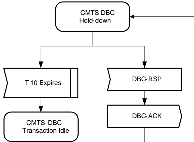
Figure 11-47 - CMTS DBC Hold-down
