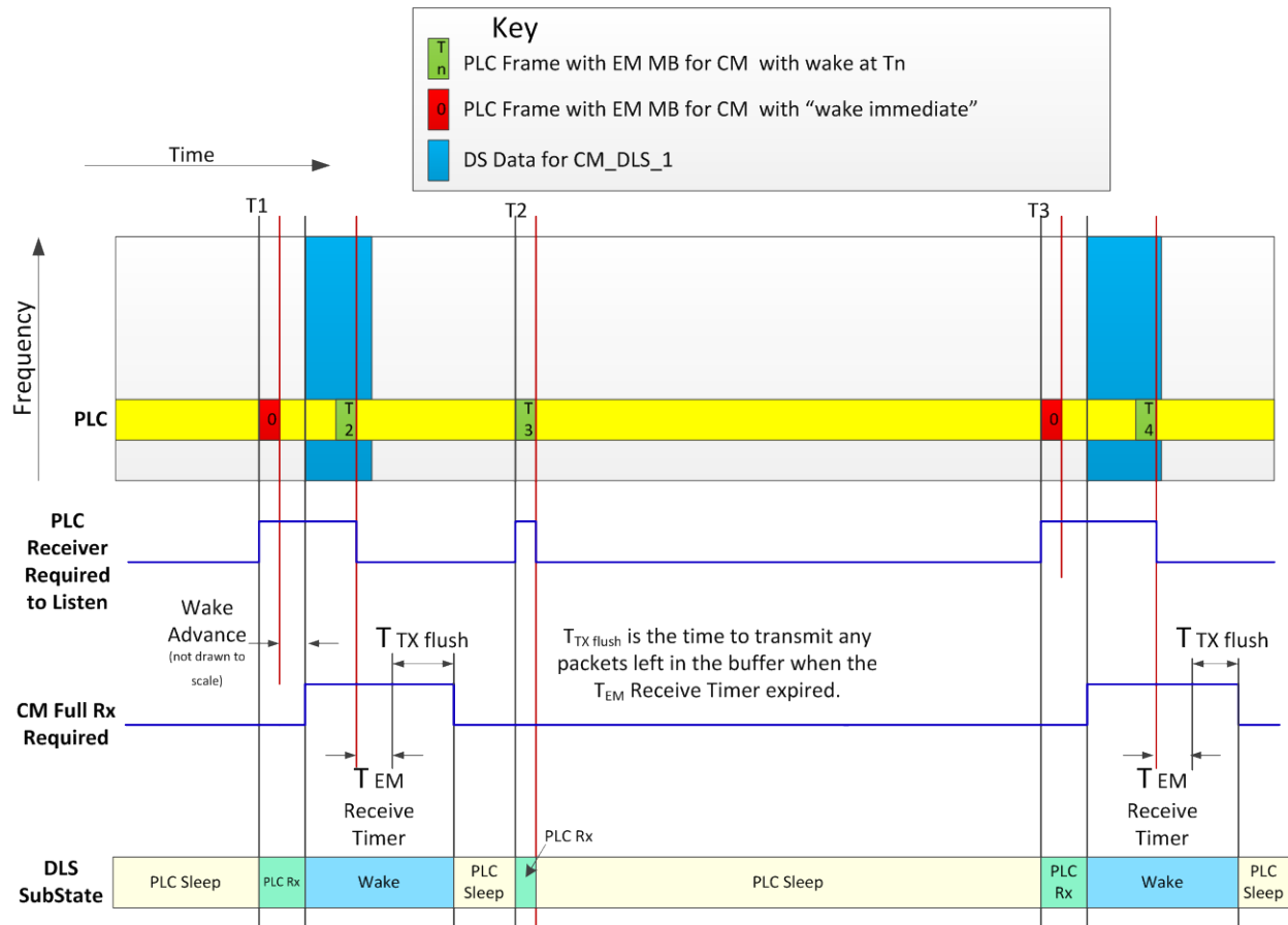
Figure 11–57 - Example Full OFDM Receiver Cycling and PLC Receiver Cycling
