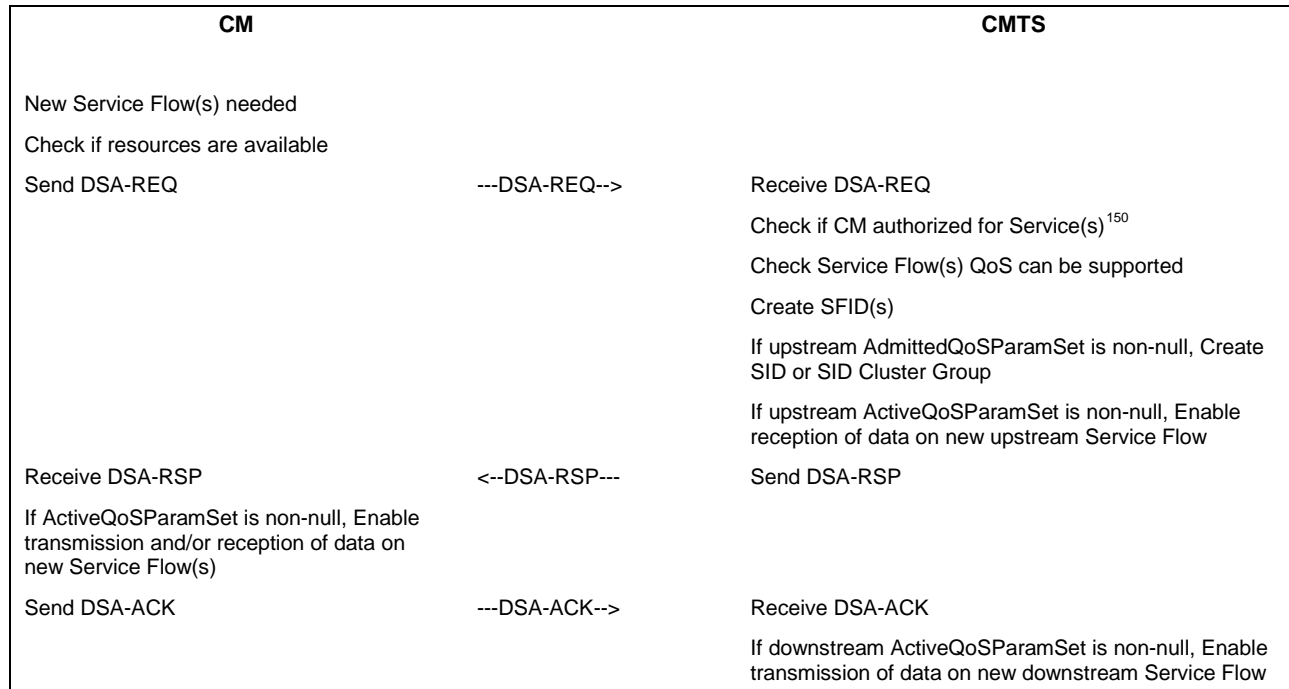
Figure 11–9 - Dynamic Service Addition Initiated from CM
