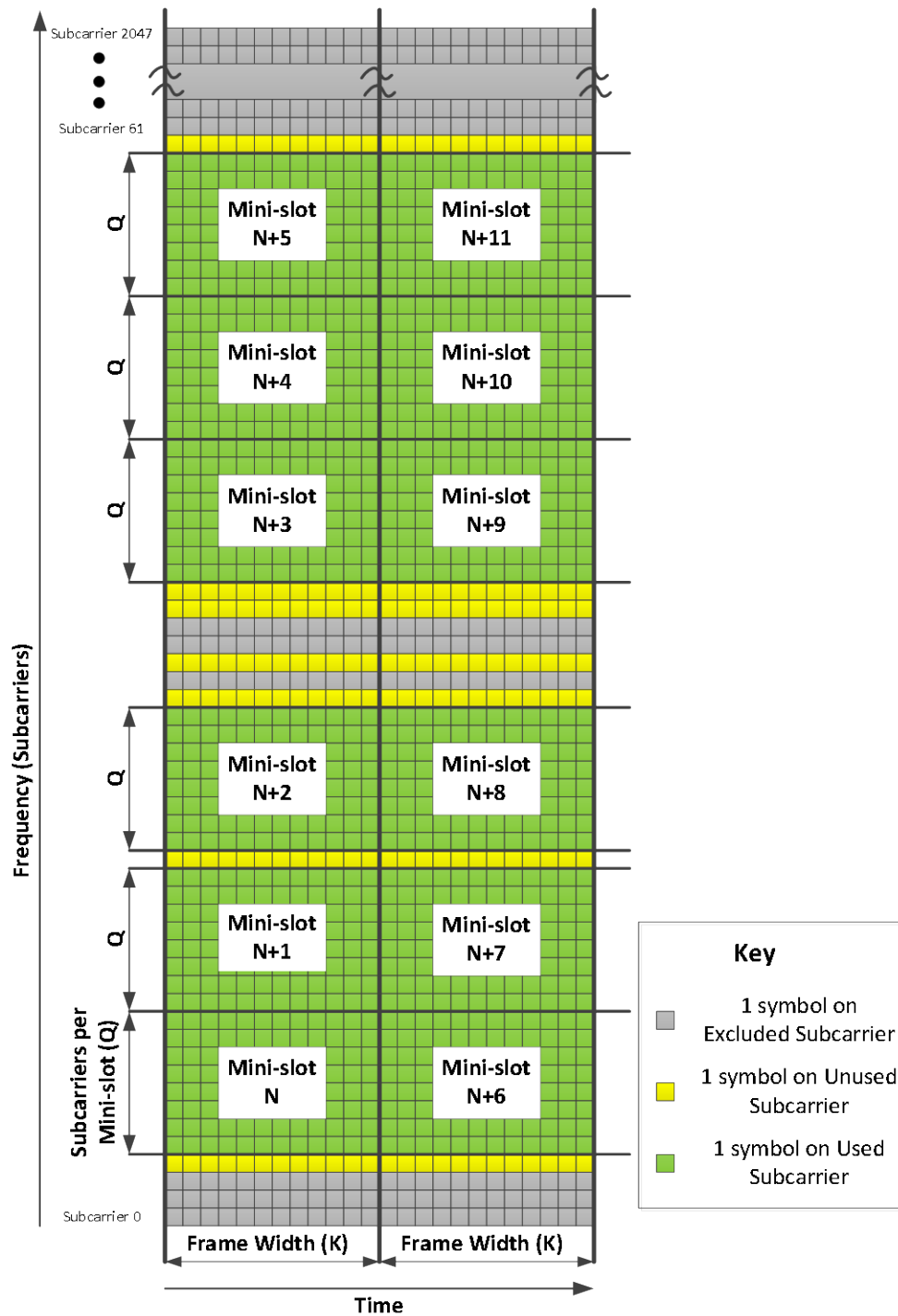
Figure 6-18 - Example Minislot Mapping for OFDMA
