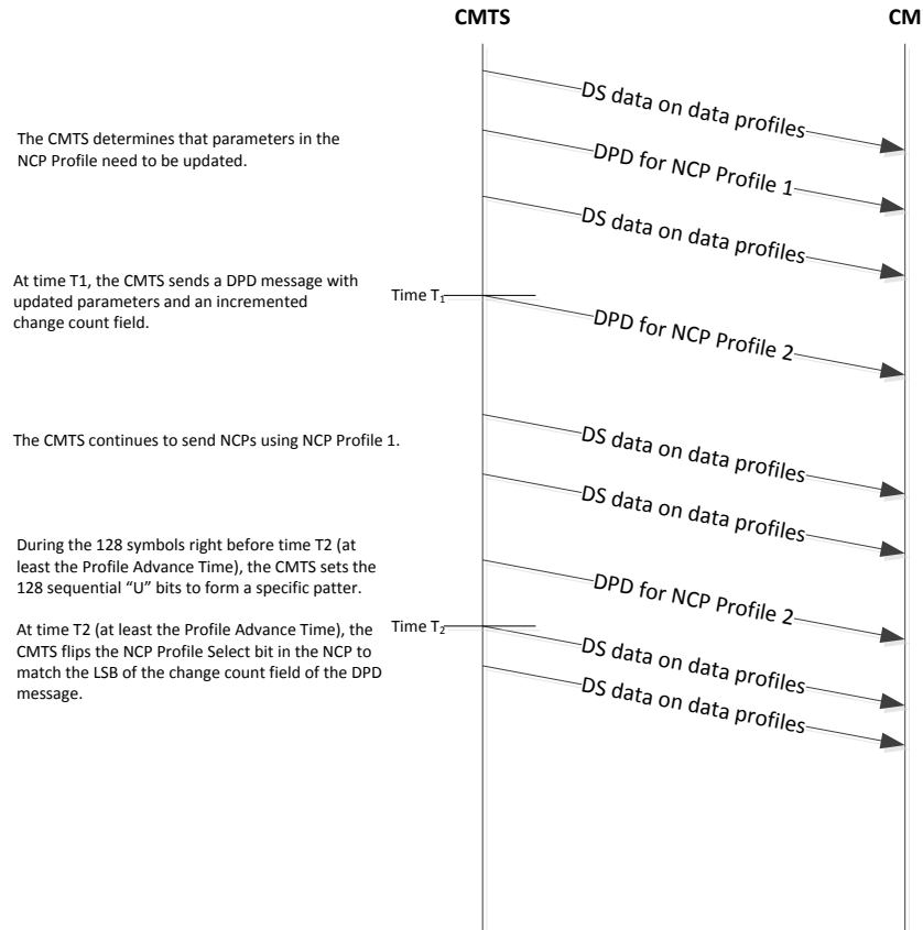
Figure XII-7 - DPD Change to the NCP Profile
