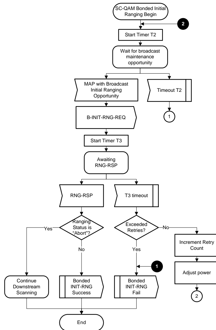
Figure 10–10 - SC-QAM Bonded Initial Ranging
