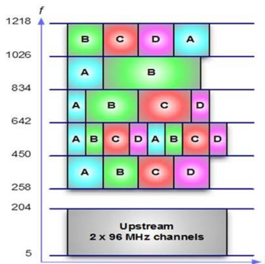
Figure 5-1 - Example view of DS and US Channels, and DS Profiles 7
