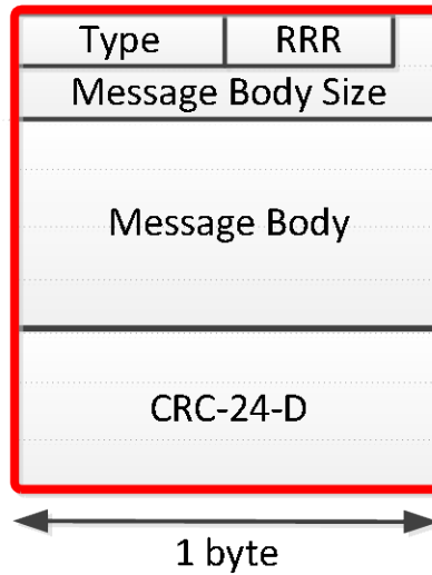
Figure 6–77- Generic Format for Message Blocks 5-15
