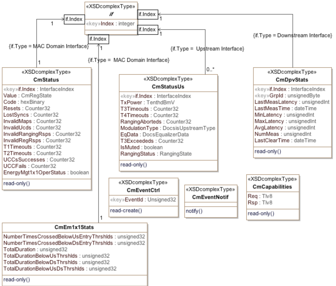
Figure N-1 - CM Operational Status Object Model Diagram 261
