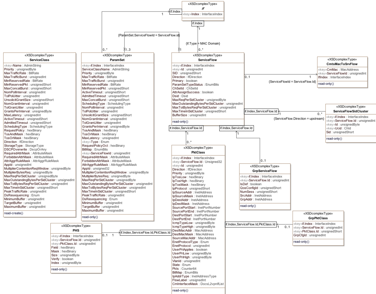
Figure O-7 - Qos Configuration Object Model Diagram 319
