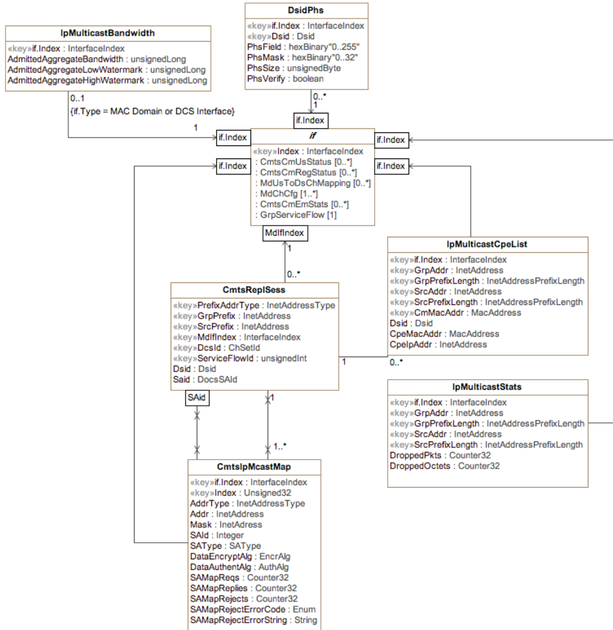
Figure M-3 - Multicast Status Reporting Object Model Diagram 249
