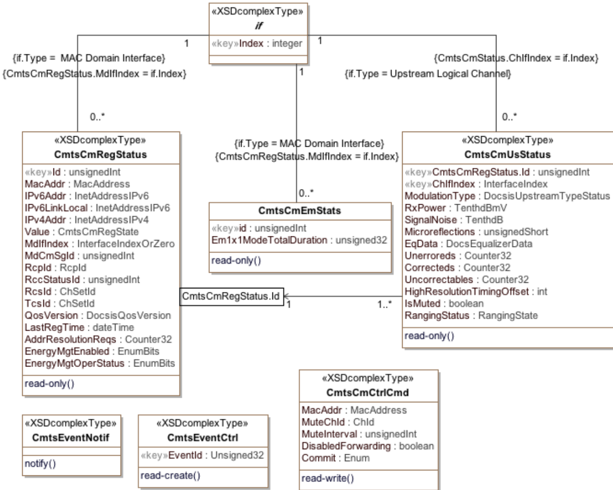
Figure N-2 - CMTS Operational Status Object Model Diagram 272
