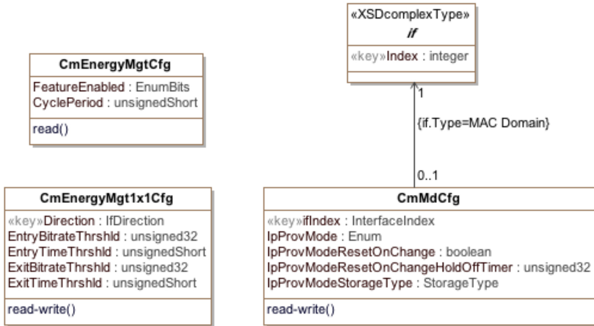
Figure O-10 - CM MAC Domain Configuration Object Model Diagram 369
