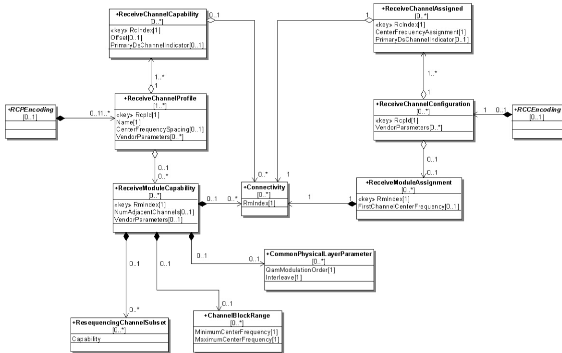
Figure VII-1 - RCP/RCC Object Model Diagram 431
