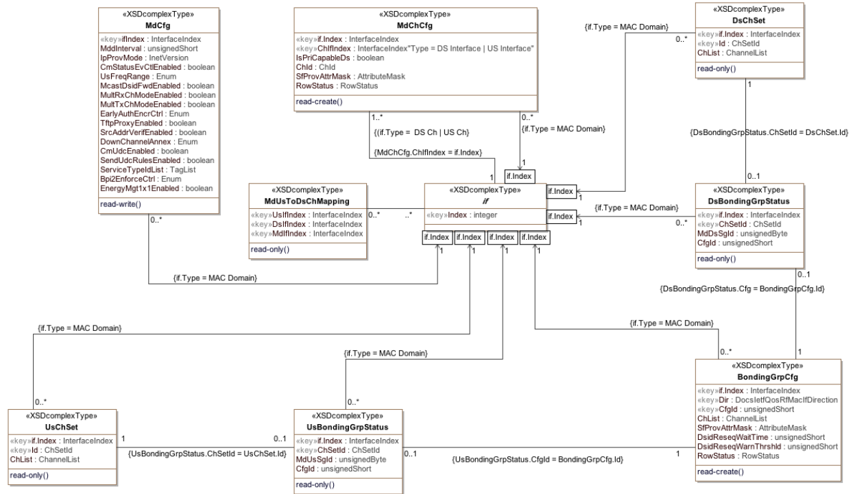
Figure O-3 - CMTS Bonding Object Model Diagram 290
