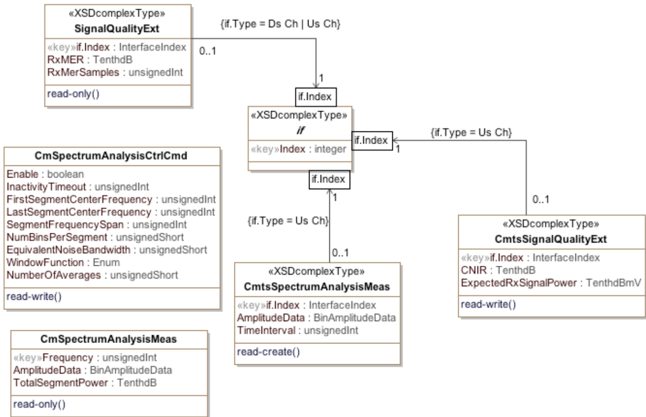
Figure J-1 - Signal Quality Monitoring Object Model Diagram 206
