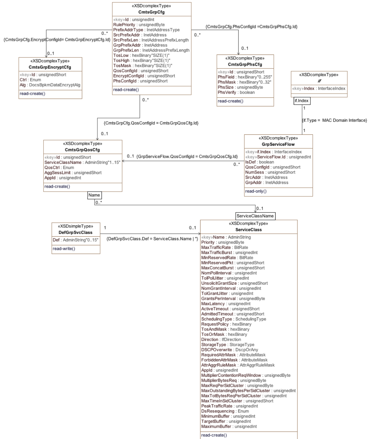
Figure M-2 - Multicast Configuration Object Model Diagram 236
