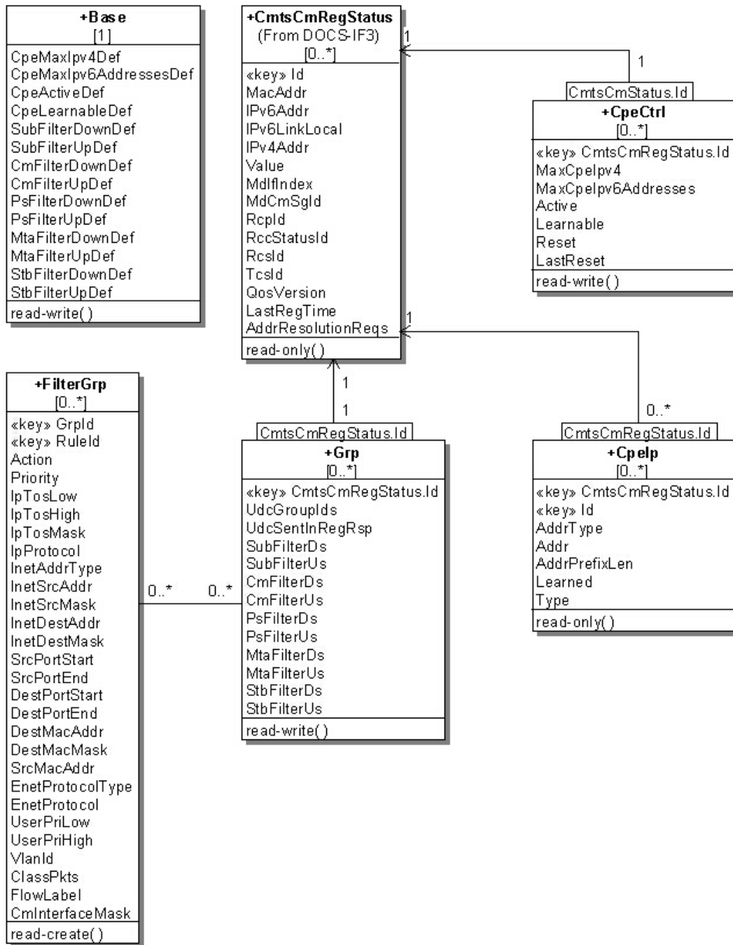
Figure P-1 - Subscriber Management Object Model Diagram 375
