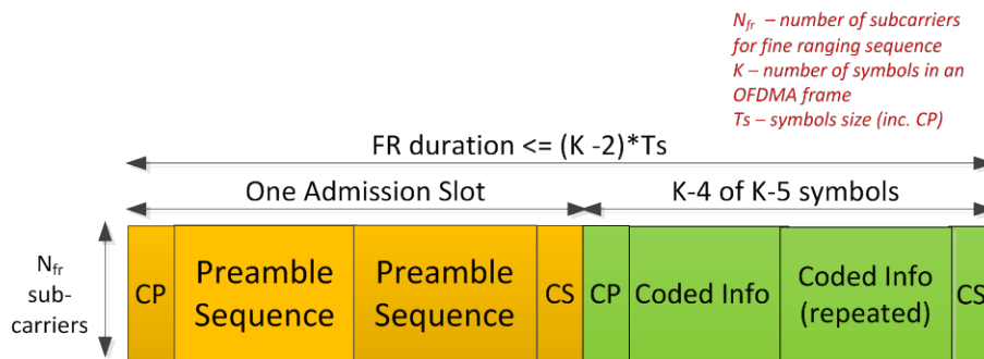
Figure 7-26 - Fine Ranging Signal
