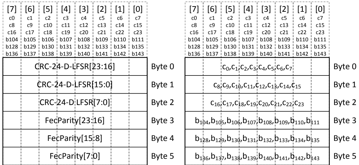
Figure 7-72 - Mapping FEC Encoded CRC-NCP Bytes into a Bitstream
