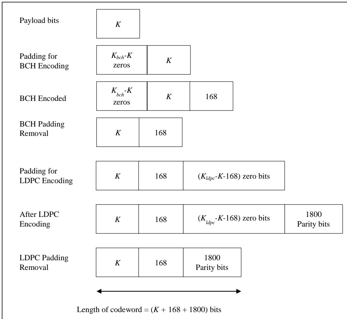
Figure 7-44 - Padding Process
