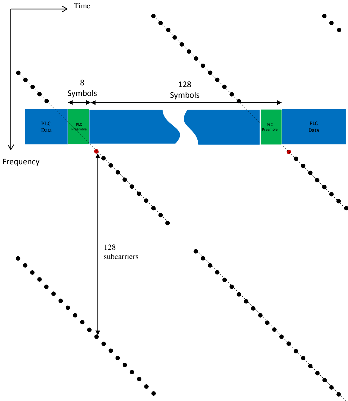
Figure 7-77 - 4K FFT Downstream Pilot Pattern
