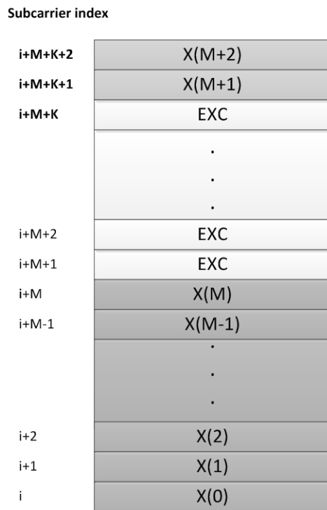
Figure 7-25 - Initial Ranging Preamble and an Exclusion Band
