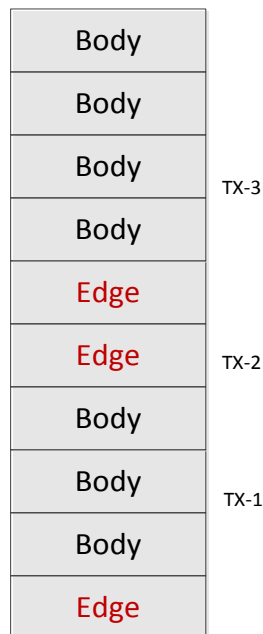
Figure 7-35 - Edge and Body Minislots in a Transmission Burst
