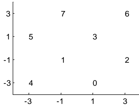
Figure A-3 - 8-QAM Constellation Mapping of \{y_0, y_1, y_2\}
