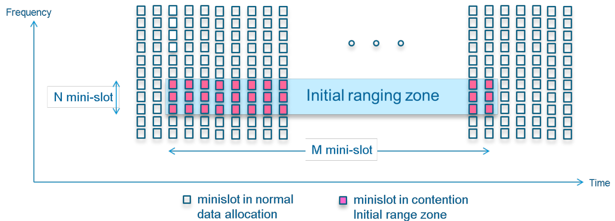
Figure 7-18 - Initial Ranging Zone
