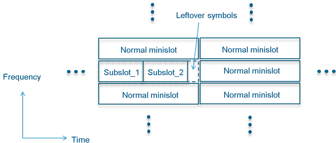
Figure 8-2 - Subslot Structure
