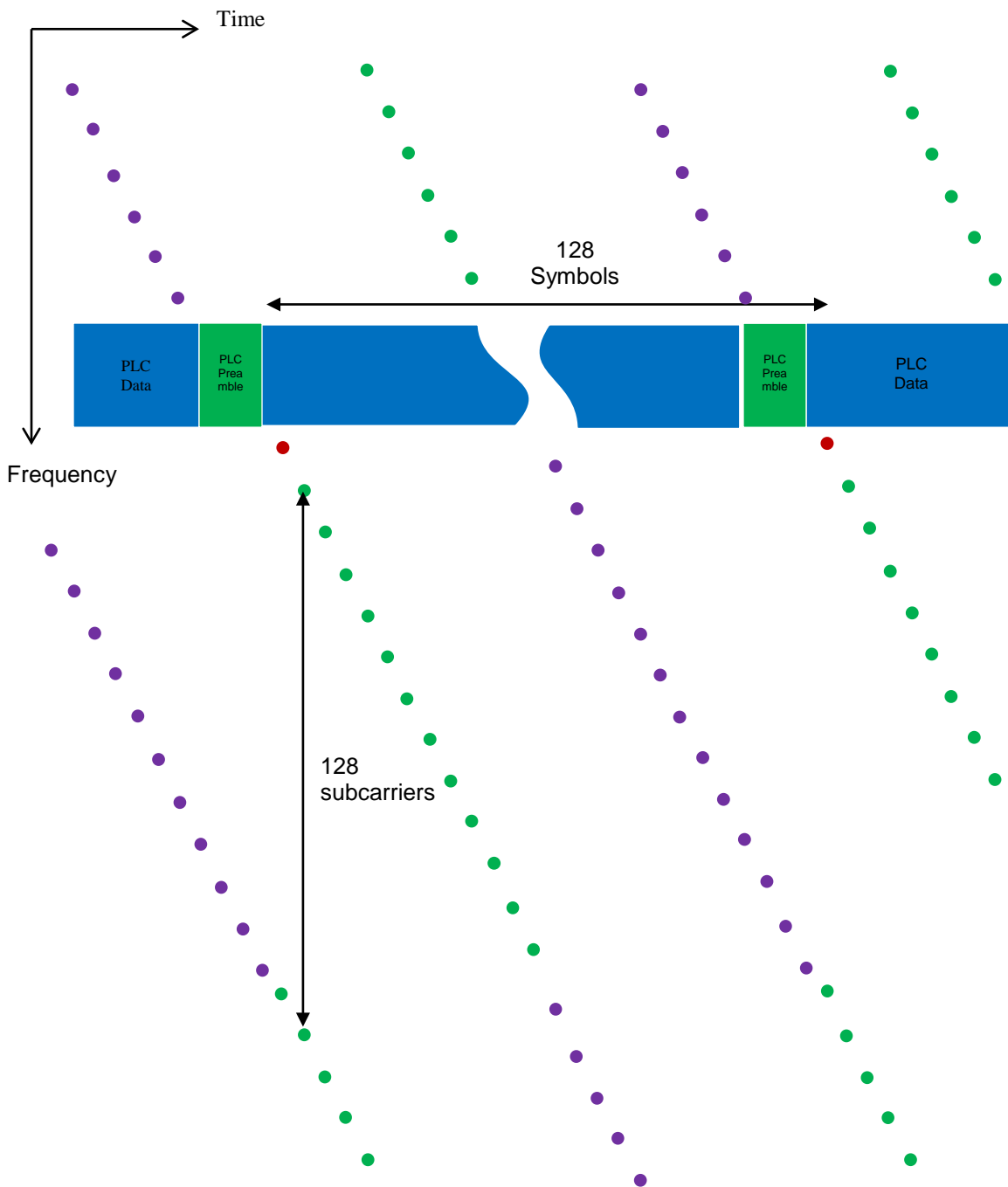
Figure 7-79 - 8K FFT Downstream Scattered Pilot Pattern
