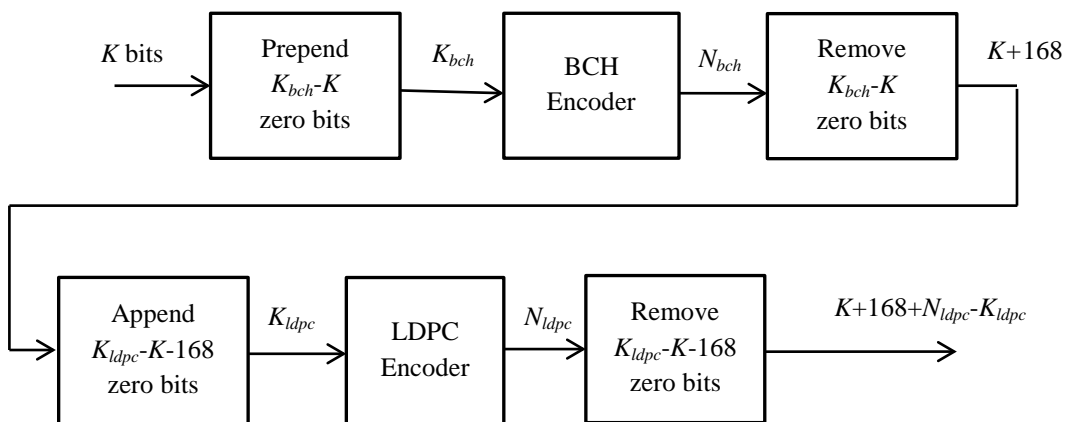
Figure 7-43 - Codeword Shortening Process
