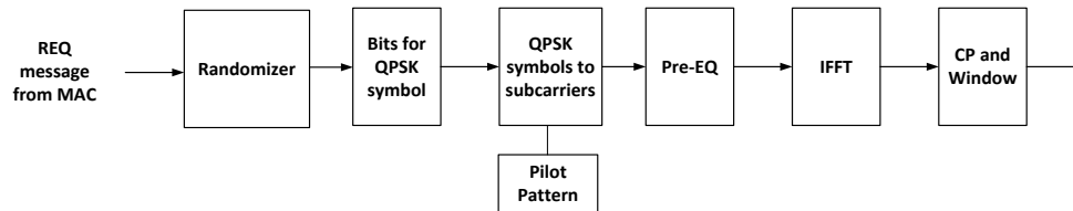
Figure 7-11 - REQ Messages Processing
