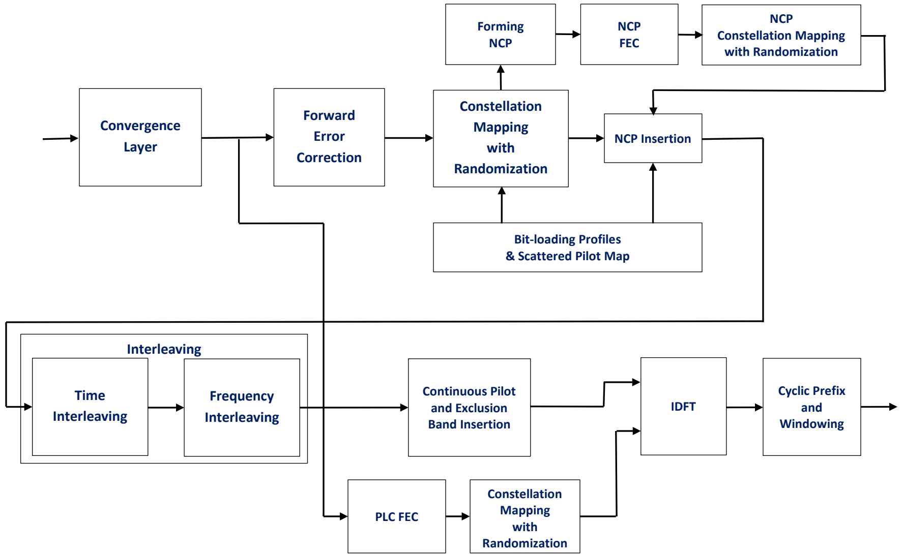
Figure 7-42 - Downstream PHY Processing
