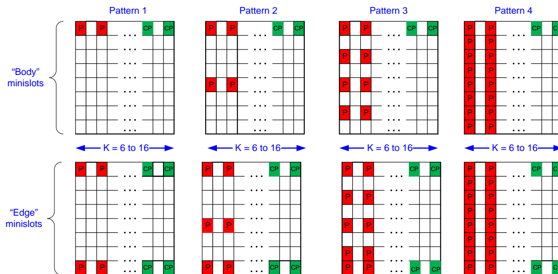
Figure 7-36 - Pilot Patterns 1-4 for Minislots with 8 Subcarriers
