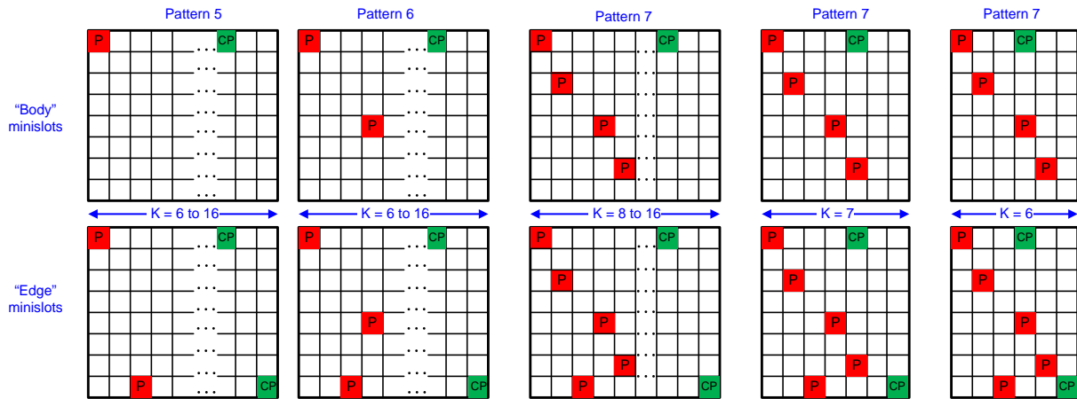
Figure 7-37 - Pilot Patterns 5-7 for Minislots with 8 Subcarriers
