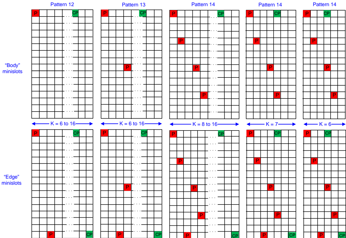
Figure 7-39 - Pilot Patterns 12-14 for Minislots with 16 Subcarriers
