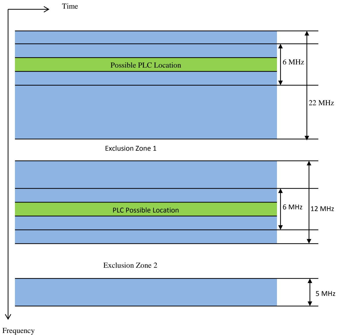
Figure 7-58 - Examples of PLC placement
