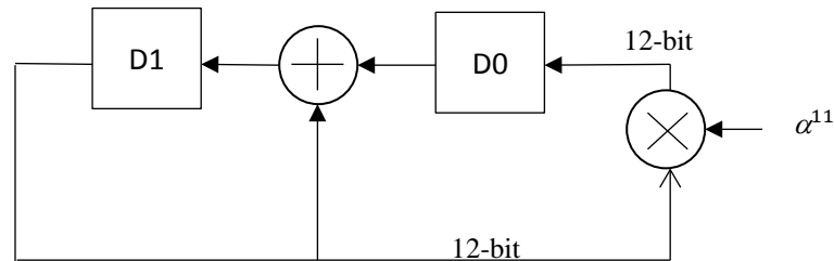
Figure 7-49 - Linear Feedback Shift Register for Randomization Sequence
