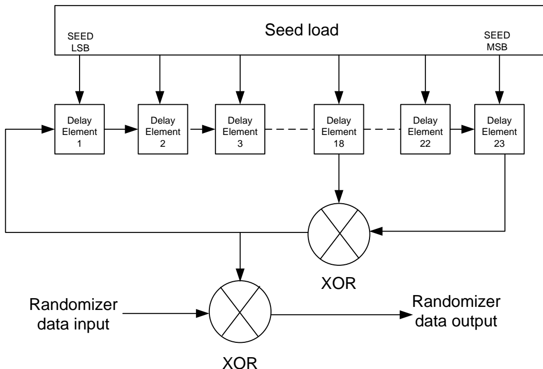
Figure 7-4 - Upstream Data Randomizer
