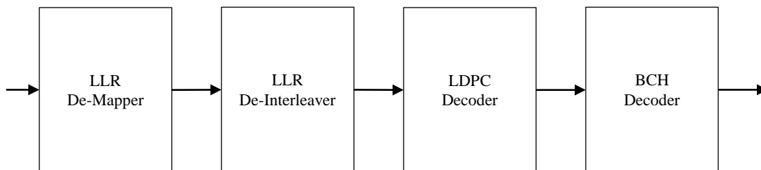
Figure 7-46 - FEC Decoding Process
