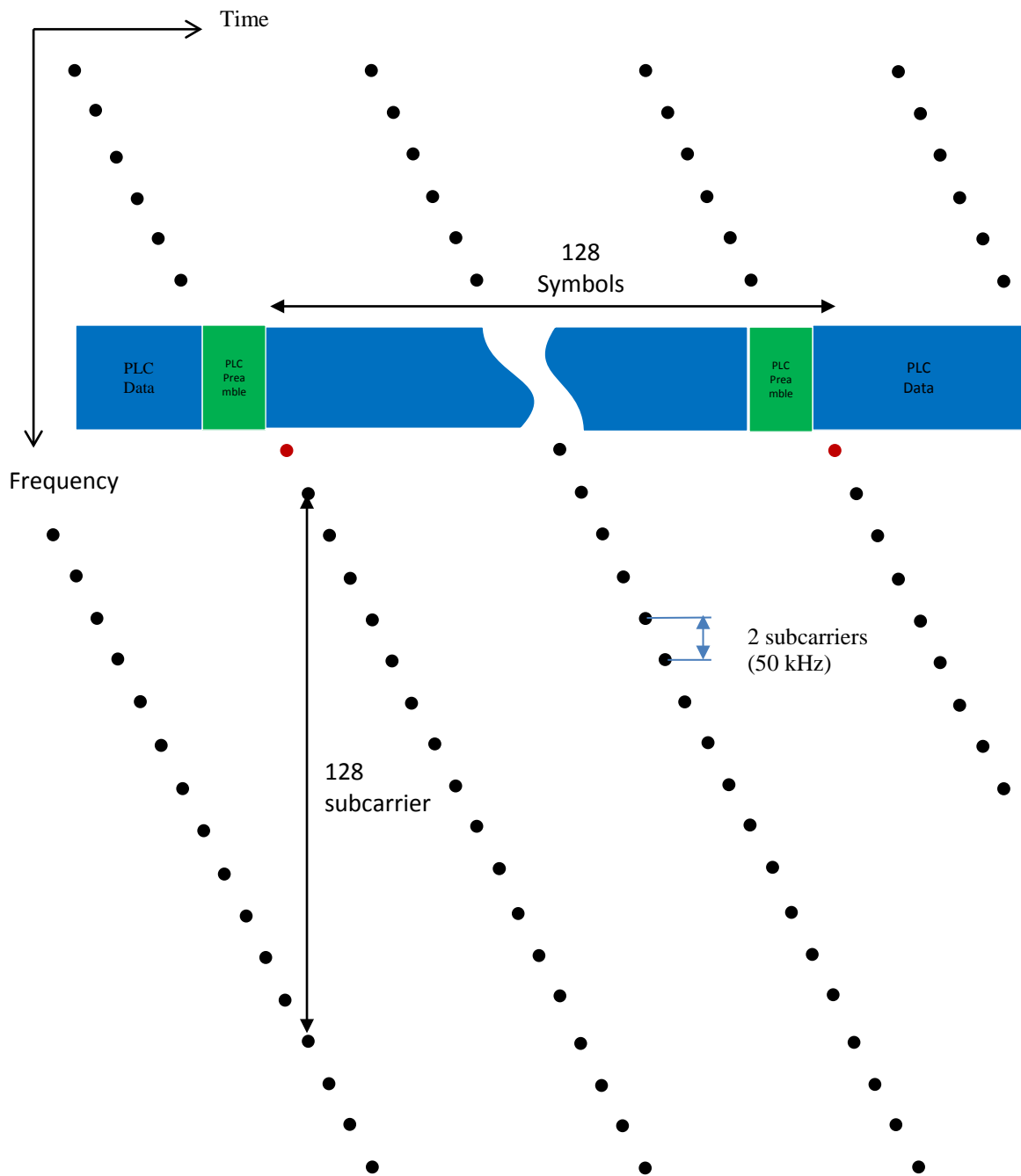
Figure 7-78 - A Downstream Scattered Pilot Pattern for 8K FFT (for Explanation Purposes Only)
