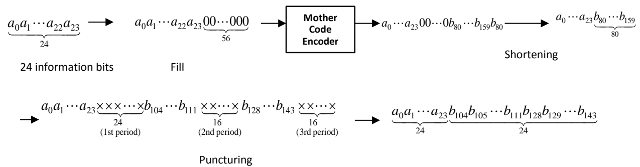
Figure 7-73 - Shortening and Puncturing Encoder for the NCP FEC
