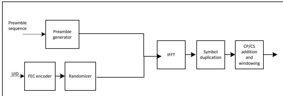
Figure 7-28 - Fine Ranging Transmitter Processing
