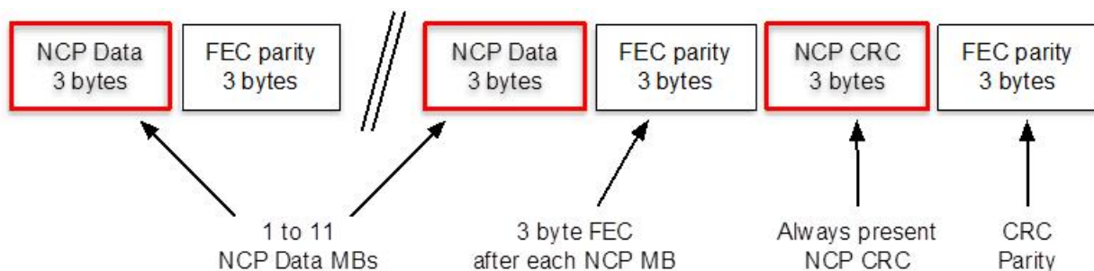
Figure 8-11 - NCP Message Blocks Field with FEC
