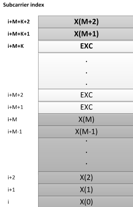
Figure 7-31 - Fine Ranging Preamble and an Exclusion Band
