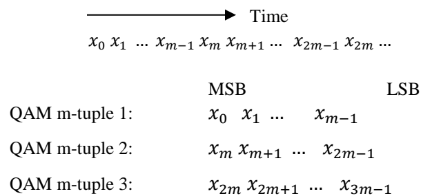
Figure 7-10 - Bitstream to QAM M-Tuple Mapping
