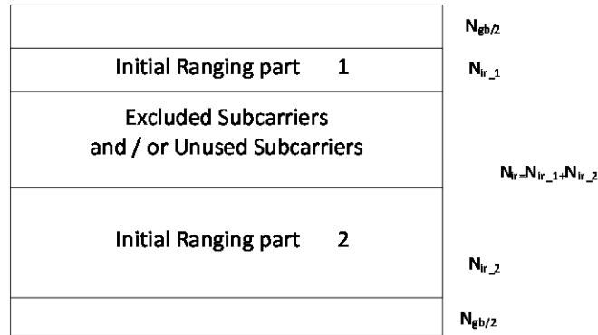
Figure 7-24 - Initial Ranging with Exclusions and Unused Subcarriers
