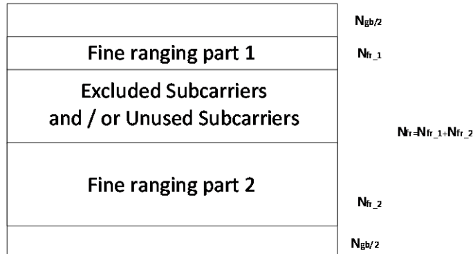
Figure 7-30 - Fine Ranging and Exclusion Bands
