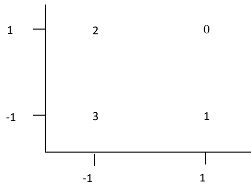
Figure 7-76 - QPSK Constellation Mapping of \{y_{i,0} y_{i,1}\}
