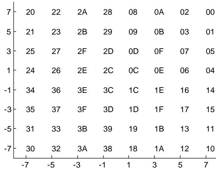
Figure A-6 - 64-QAM Constellation Mapping of \{y_0y_1y_2y_3y_4y_5\}
