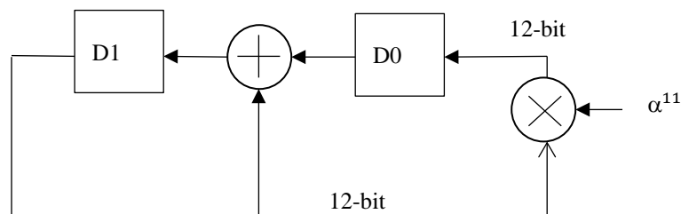
Figure 7-65 - Linear Feedback Shift Register for PLC Randomization
