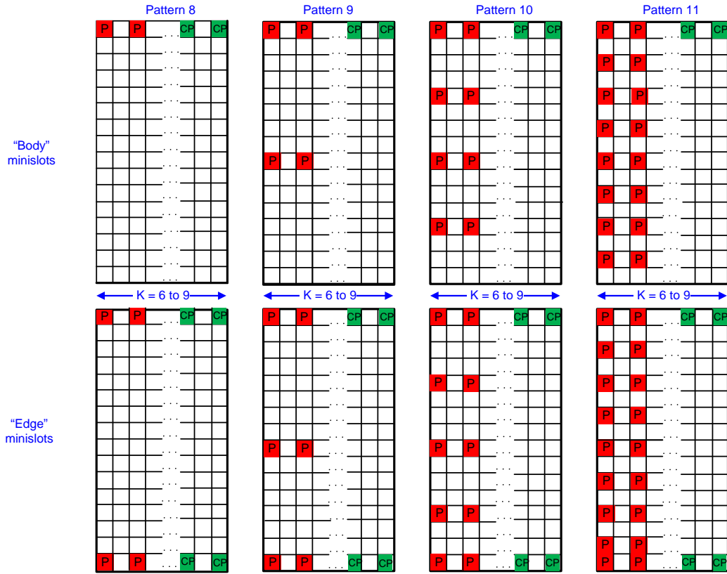
Figure 7-38 - Pilot Patterns 8-11 for Minislots with 16 Subcarriers
