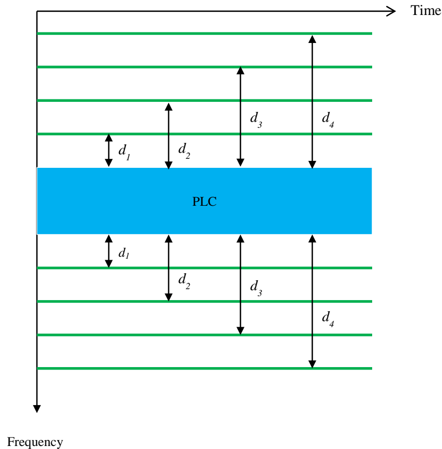
Figure 7-80 - Placement of Predefined Continuous Pilots around the PLC
