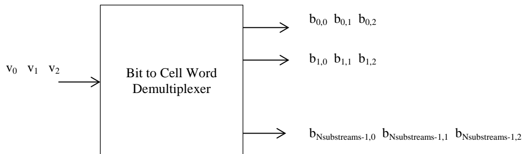
Figure 7-48 - Bit-to-Cell Word Demultiplexer
