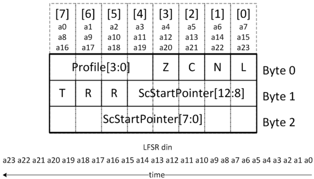
Figure 7-68 - Mapping NCP Bytes into a Bitstream for FEC Encoding
