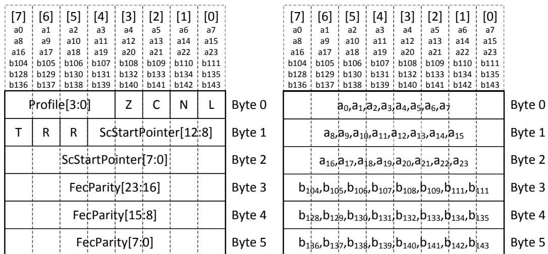
Figure 7-69 - Mapping FEC Encoded NCP Bytes into a Bitstream
