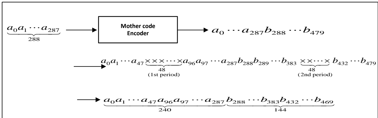
Figure 7-61 - Puncturing Encoder for the PLC FEC
