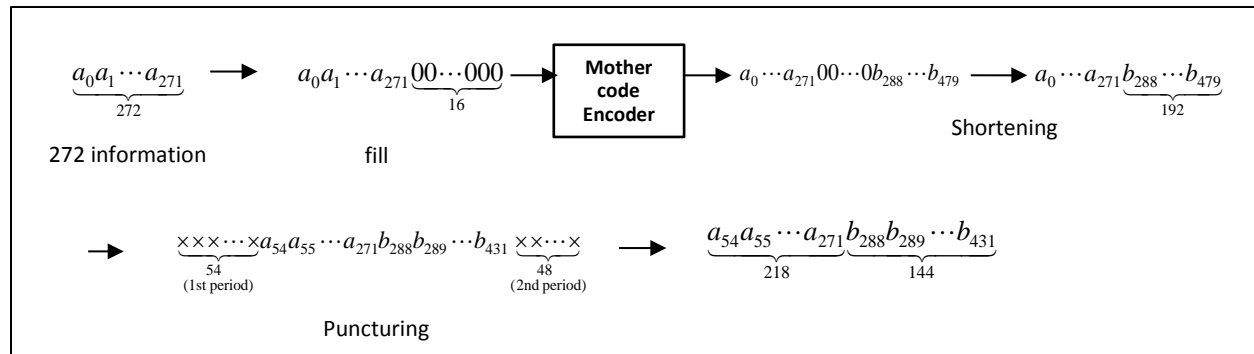
Figure 7-29 - Shortening and Puncturing Encoder for the Fine Ranging FEC
