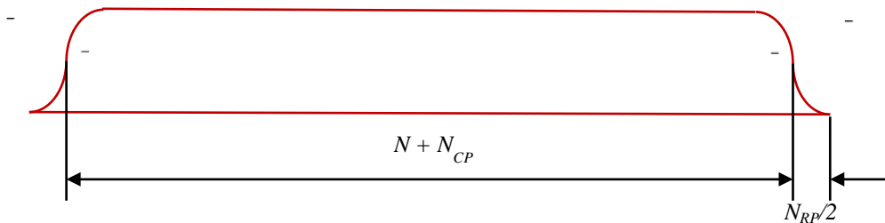
Figure 7-15 - Tapering Window
