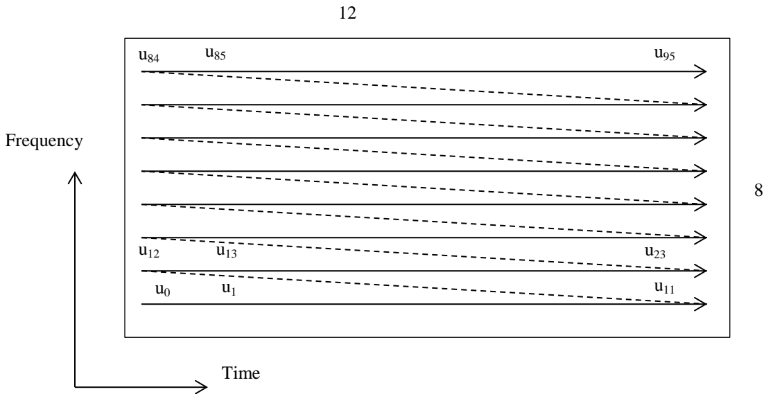
Figure 7-63 - Block Interleaving of PLC Subcarriers for 4K FFT
