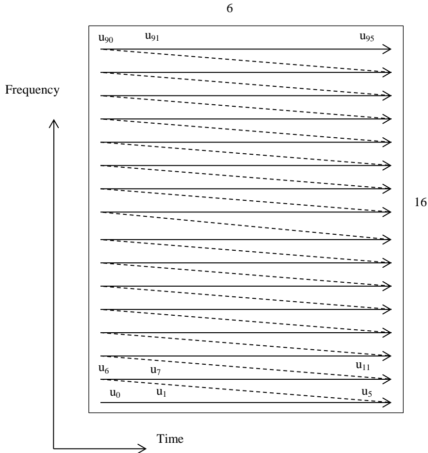
Figure 7-64 - Block Interleaving of PLC Subcarriers for 8K FFT
