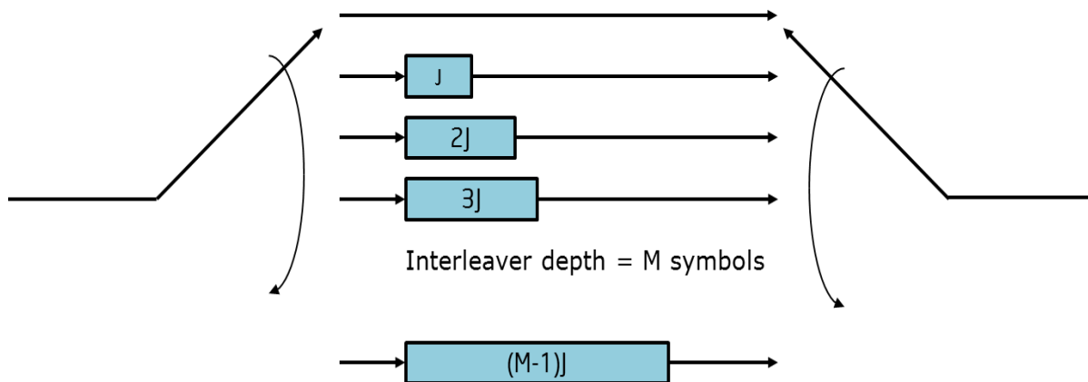
Figure 7-52 - Time Interleaver Structure
