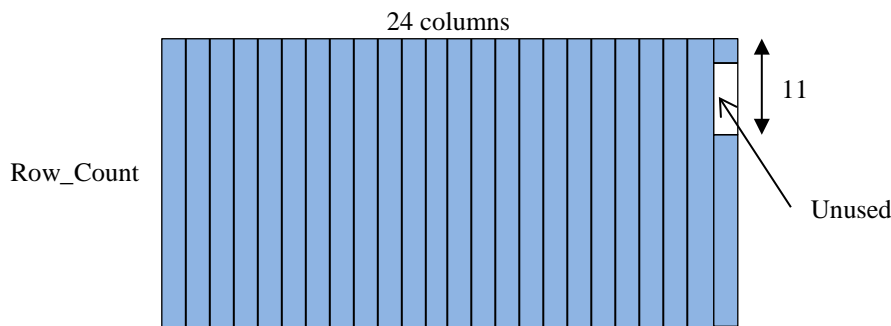
Figure 7-45 - Bit De-interleaver Block for a Shortened Codeword
