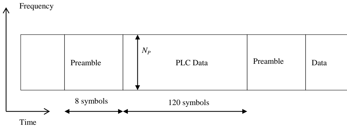
Figure 7-57 - Structure of the PLC
