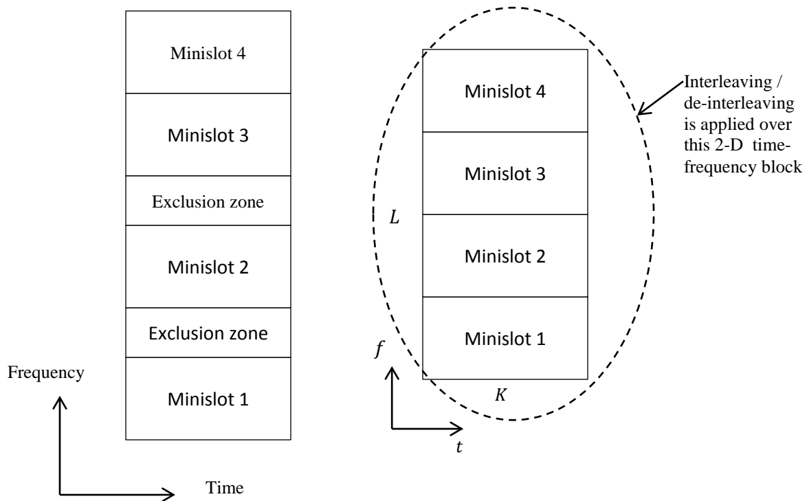
Figure 7-6 - Illustrating Minislots of a Grant over which Interleaving is Performed
