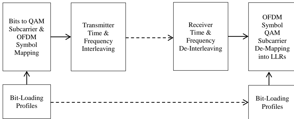
Figure 7-50 - Bit Loading, Symbol Mapping, and Interleaving
