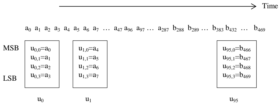
Figure 7-62 - Mapping Encoded Bitstream into a Stream of Nibbles
