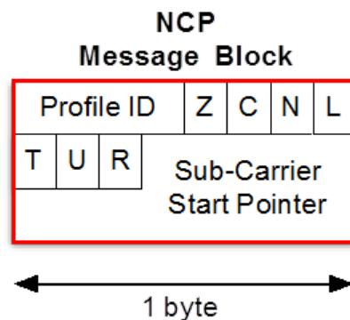
Figure 8-8 - NCP Data Message Block
