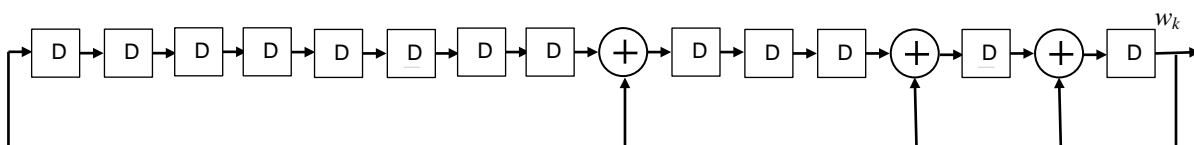
Figure 7-81 - 13-Bit Linear Feedback Shift Register for the Pilot Modulation Pseudo-Random Sequence
