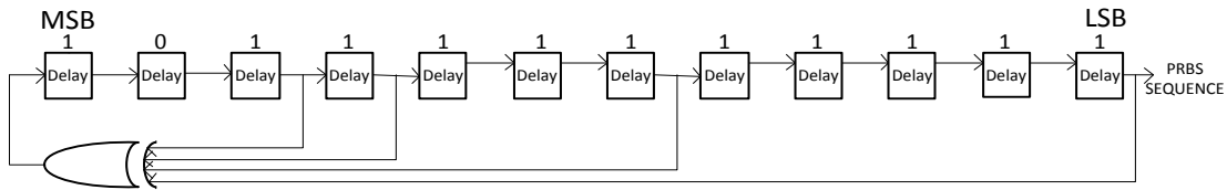
Figure 7-32 - Polynomial Sequence for Pseudorandom Binary Sequence Generation
