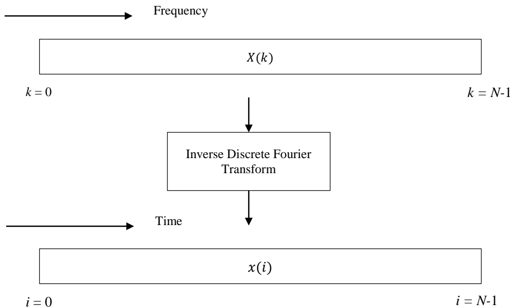
Figure 7-56 - Inverse Discrete Fourier Transform
