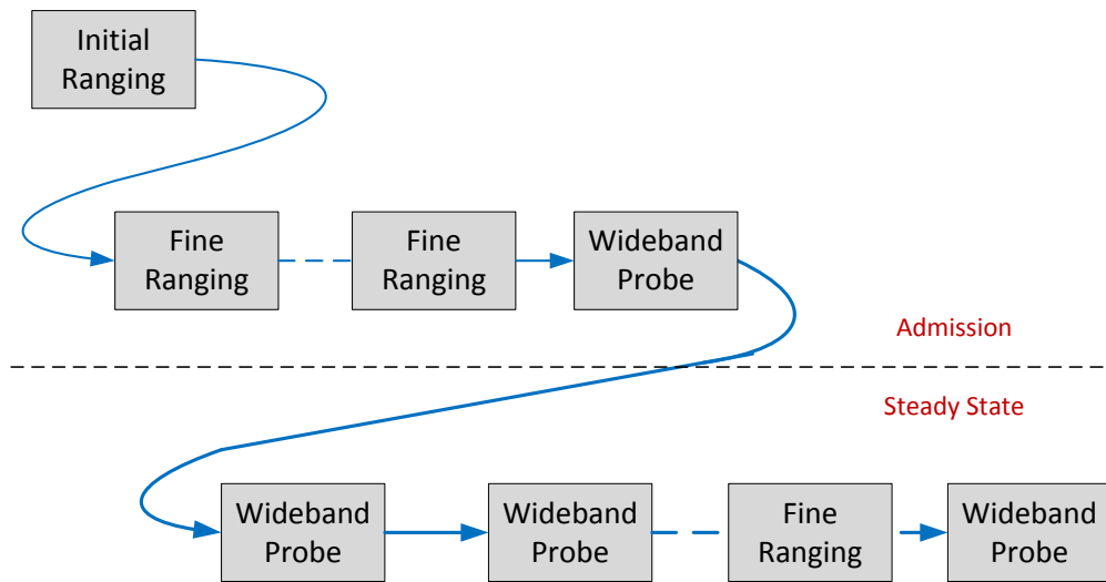
Figure 7-17 - Ranging Steps
