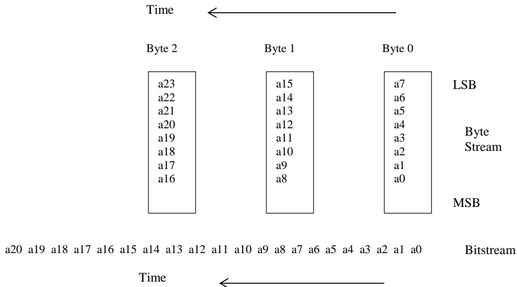
Figure 7-60 - Mapping Bytes into a Bitstream for FEC Encoding
