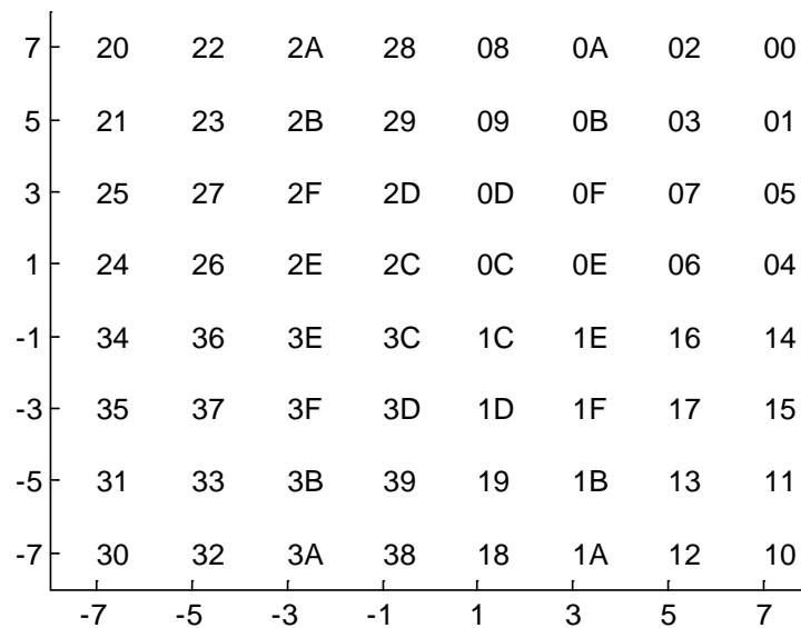
Figure 7-74 - 64-QAM Constellation Mapping of \{y_{i,0}y_{i,1}y_{i,2}y_{i,3}y_{i,4}y_{i,5}\}
