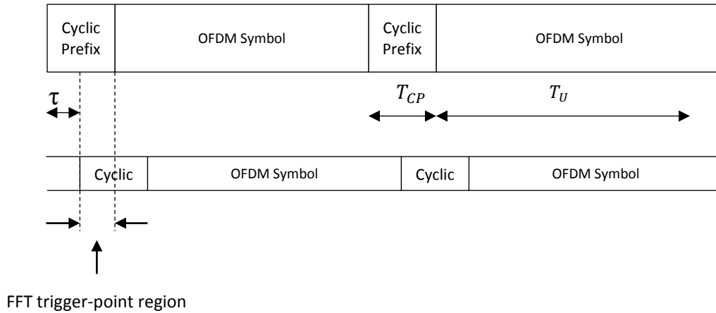
Figure 7-13 - Signal with Micro-Reflection at the Receiver
