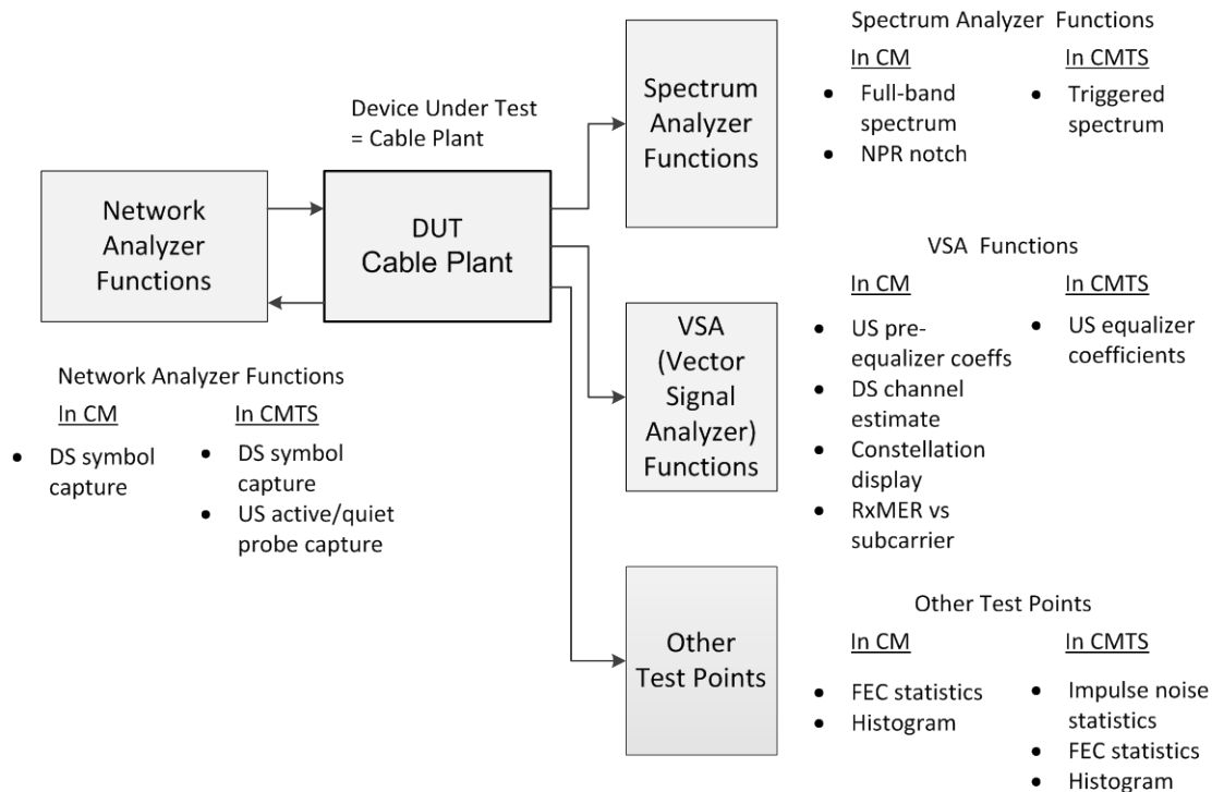
Figure 9-1 - Test points in CM and CMTS Supporting Proactive Network Maintenance
