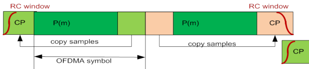
Figure 7-20 - Initial Ranging Admission Slot Structure
