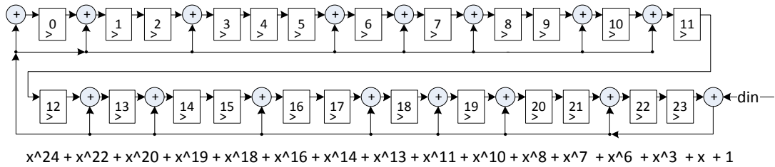
Figure 7-70 - Polynomial Sequence for CRC-24-D Encoding
