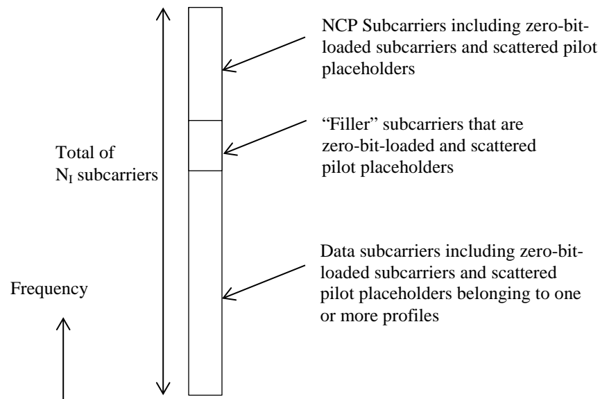
Figure 7-51 - NCP Insertion
