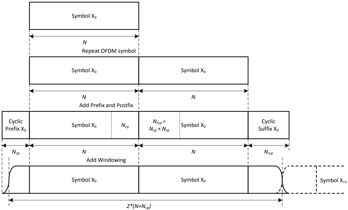
Figure 7-23 - Initial Ranging Symbol Pair Structure
