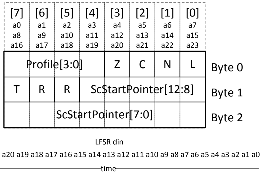
Figure 7-71 - Mapping NCP Data into the CRC-24-D Encoder
