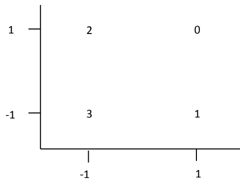
Figure A-2 - QPSK Constellation Mapping of \{y_0y_1\}
