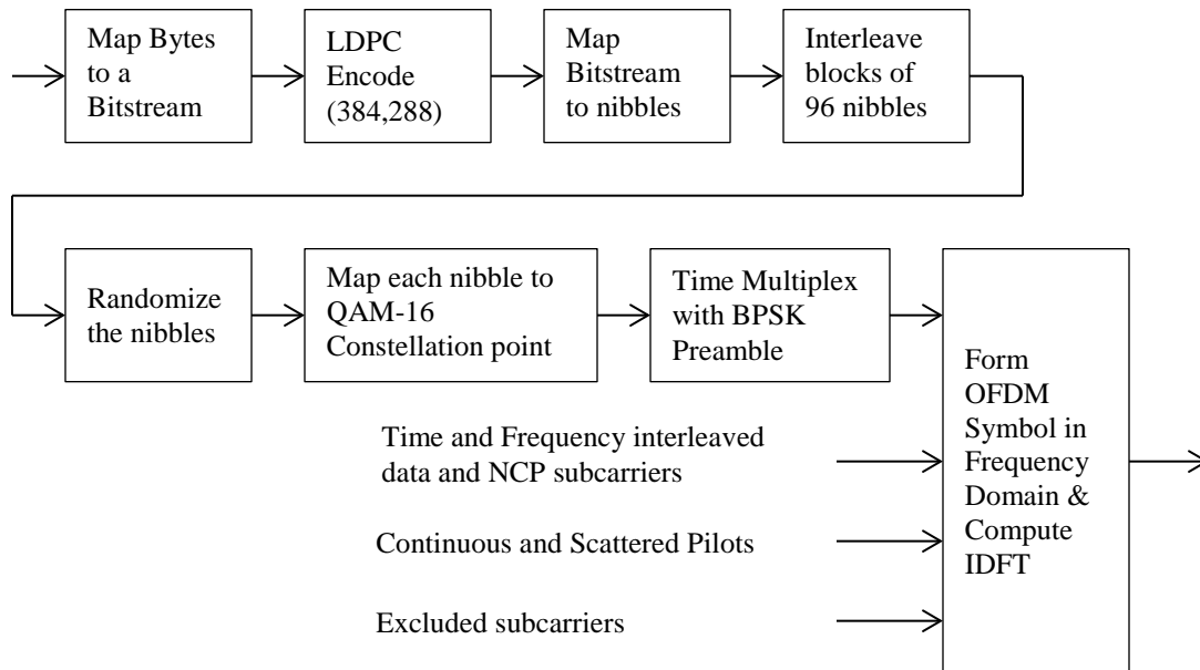
Figure 7-59 - Physical Layer Operations for Forming the PLC Subcarriers
