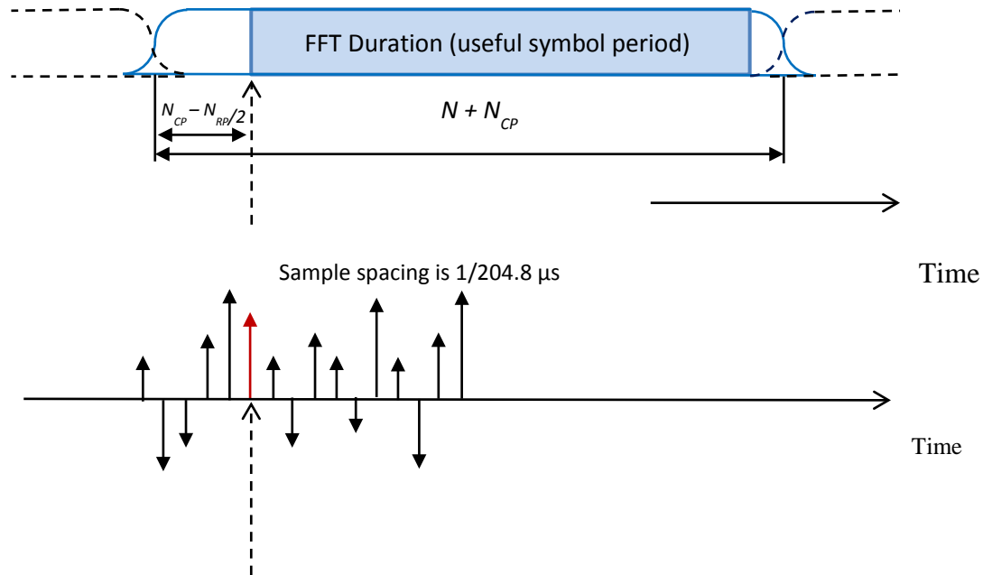
Figure 7-67 - Time Domain Representation of PLC Timestamp Synchronization
